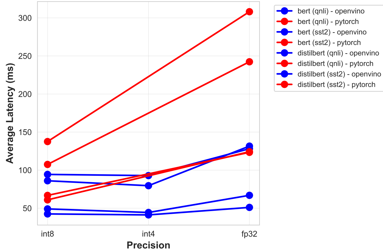
Latency vs Precision (Lower is Better)
