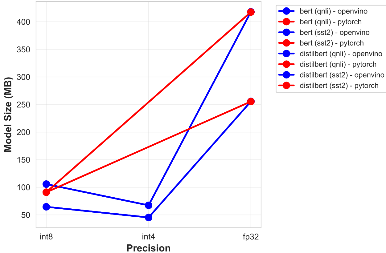
Model Size vs Precision (Lower is Better)
