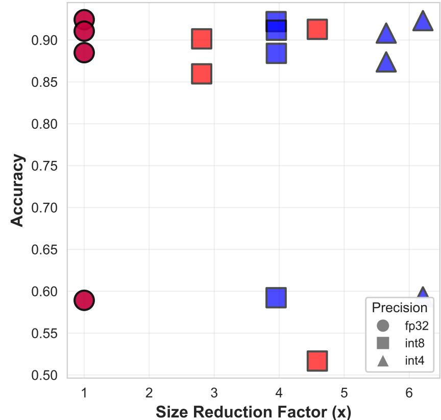
Accuracy vs Compression (Top-Right is Best)
