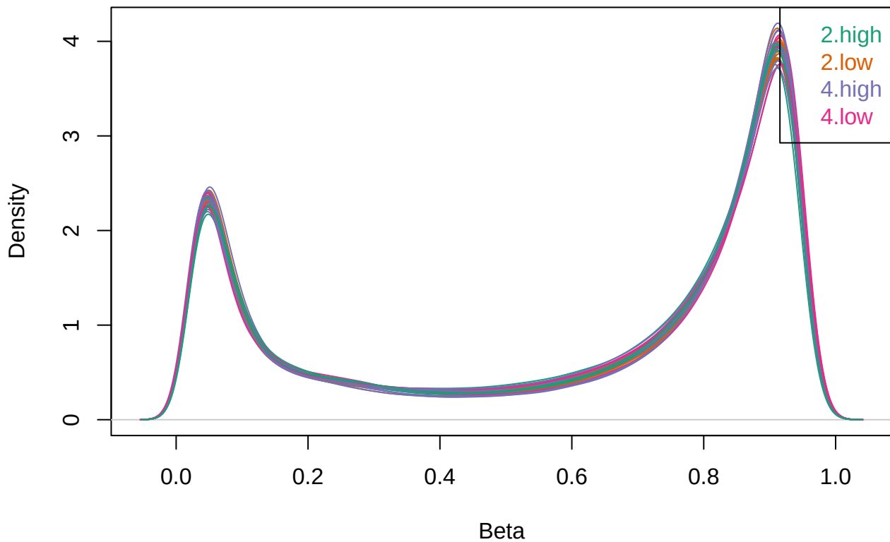
Beta density (normalized, filtered)
