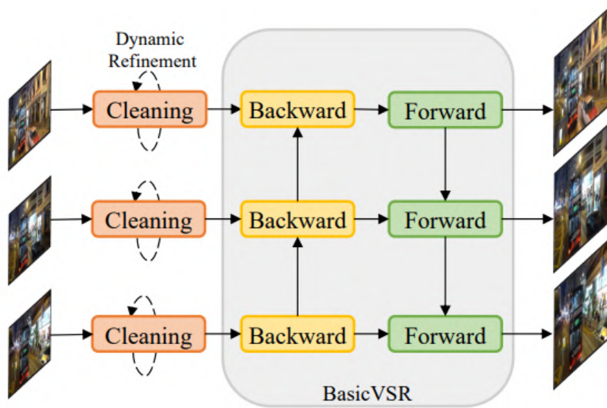
Figure 4.9: RealBasicVSR architecture
