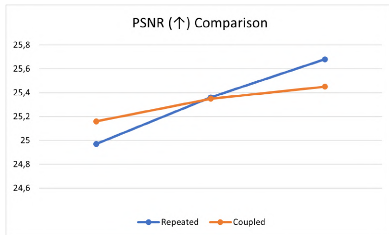
Figure 4.7: Repeated vs Coupled propagation - PSNR
