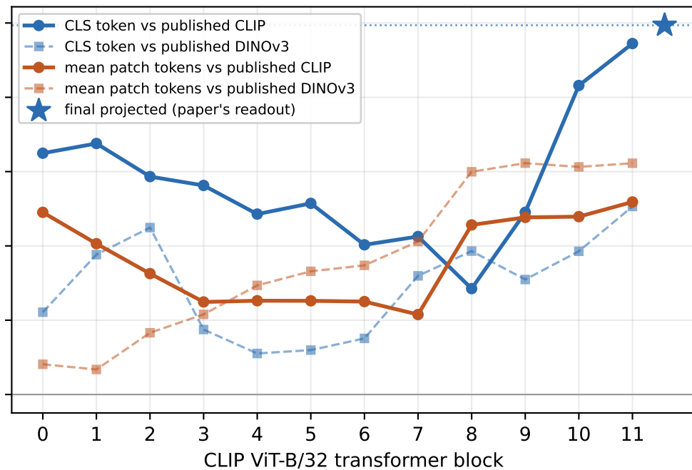
Local dispersion (kNN, k=5)
