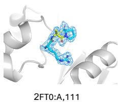
Turn A-GCG:A-GCT w2torus(4-fixed)
