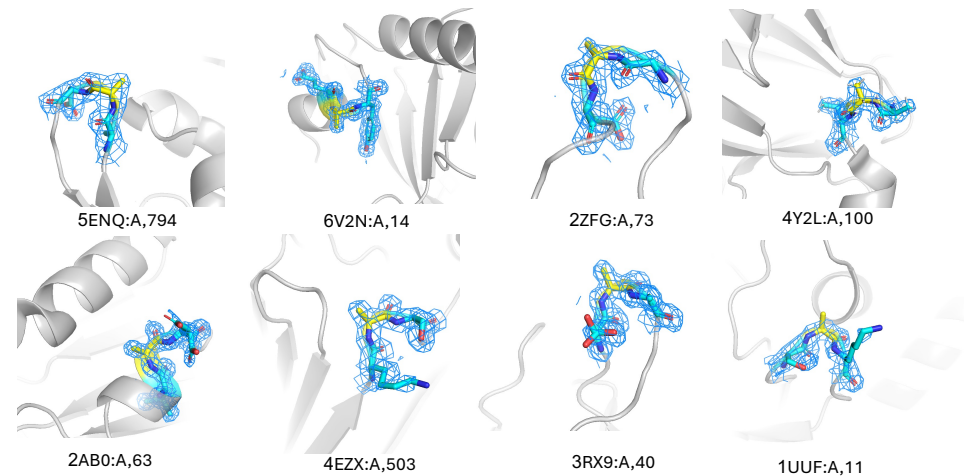
Turn A-GCG:A-GCT mmd(unbiased)
