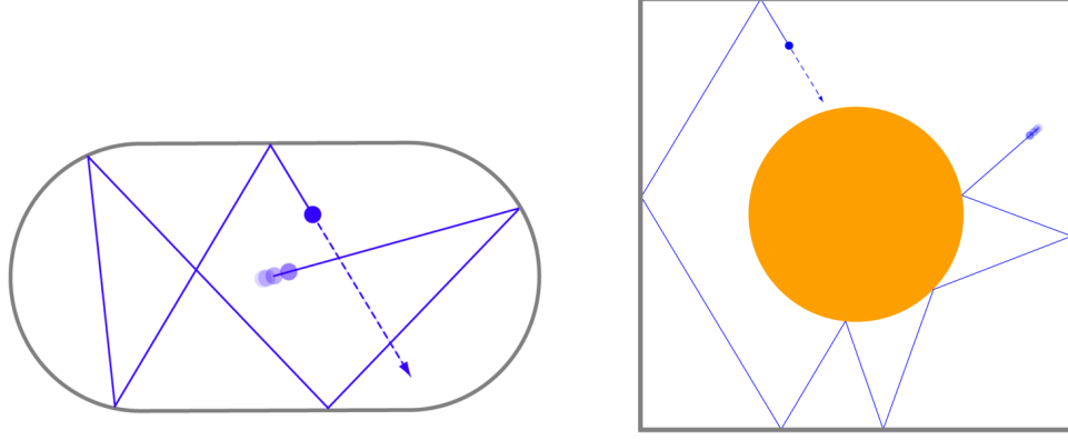
Figure 3: Billiard dynamical systems: (a) The “Bunimovich stadium”; (b) The “Sinai billiard” (source: Wikipedia)
