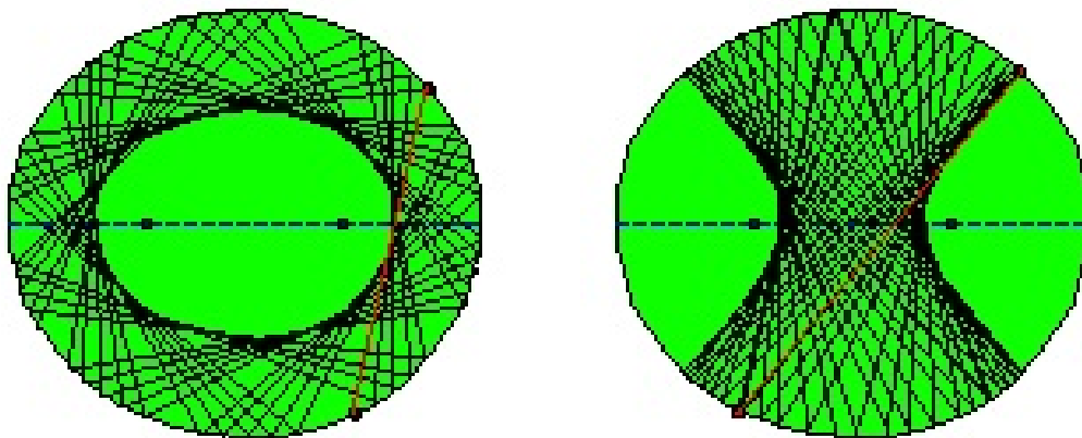
Figure 4: Billiard in an ellipse-shaped domain
