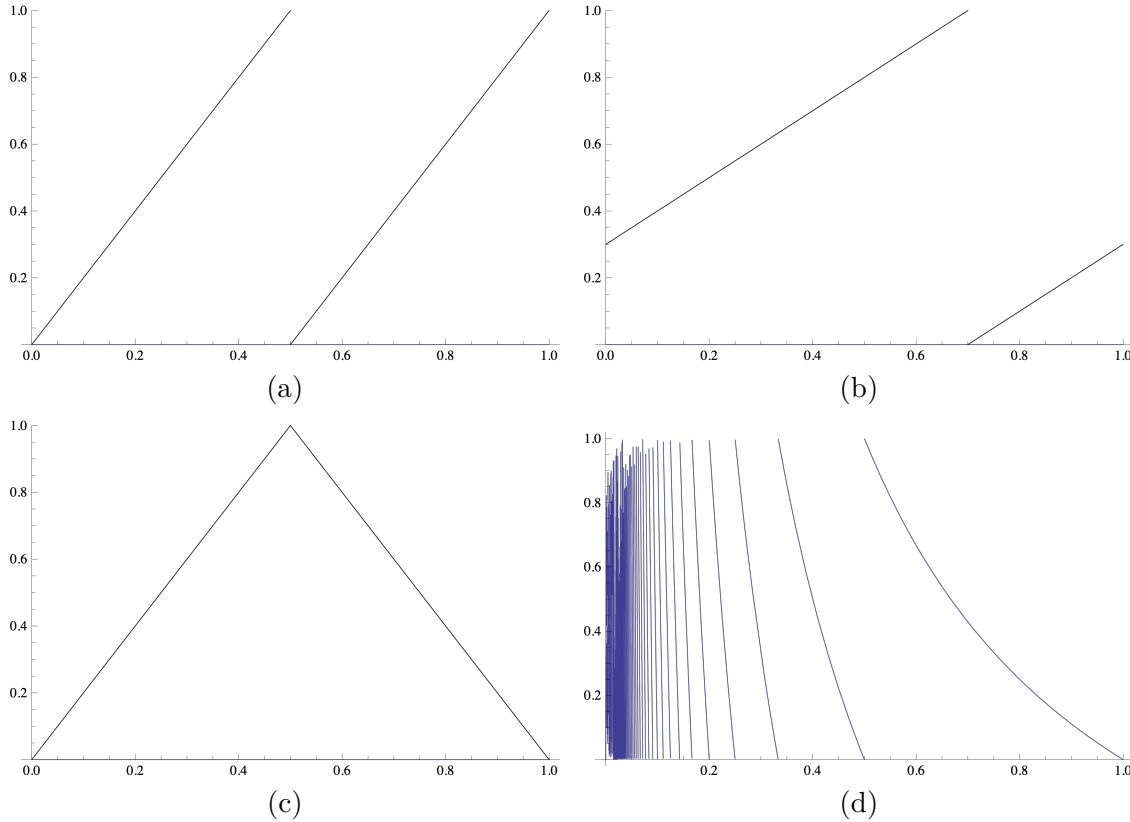
Figure 10: (a) The doubling map; (b) The circle rotation map R_\alpha for \alpha = 0.3 ; (c) the tent map \Lambda_2 ; (d) The Gauss map.
