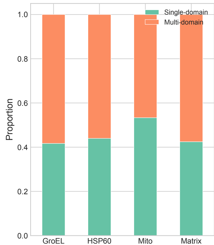
C. Domain Count Distribution
