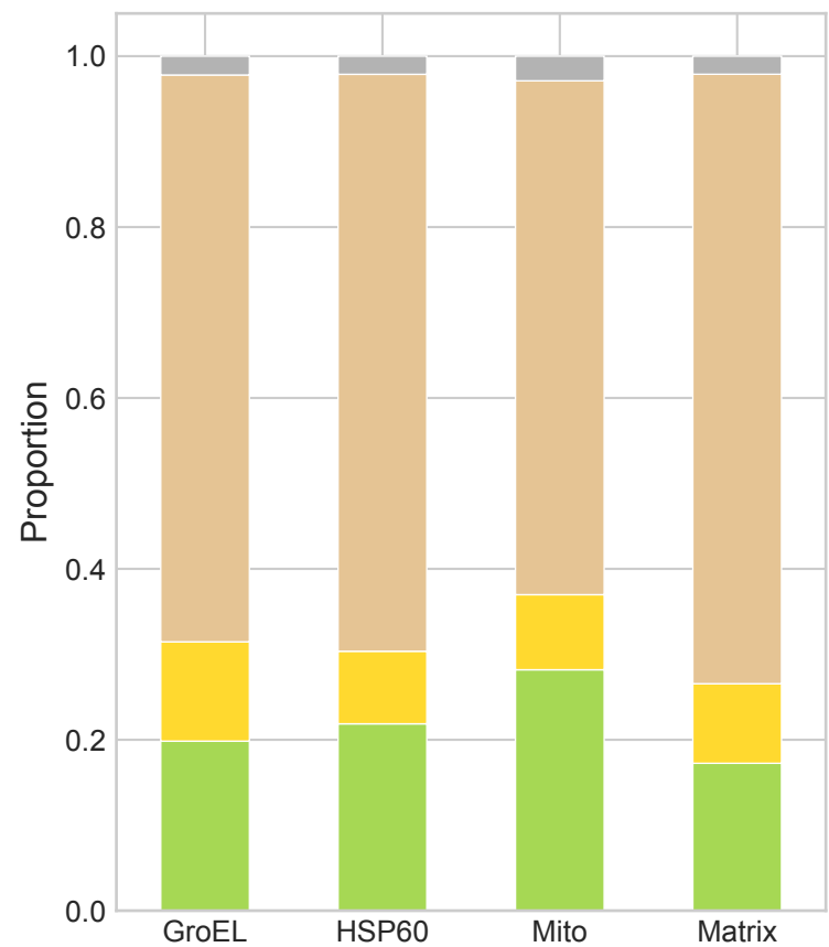
A. CATH Class Distribution
