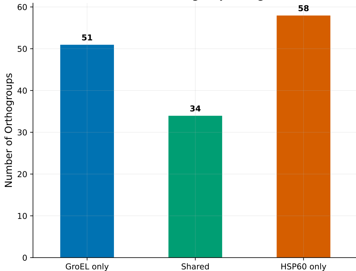
Substrate Orthogroup Categories
