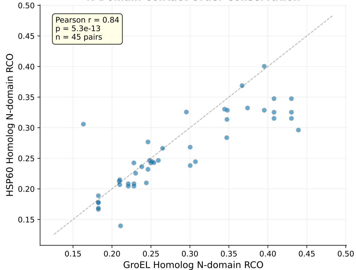
N-Domain Contact Order Conservation
