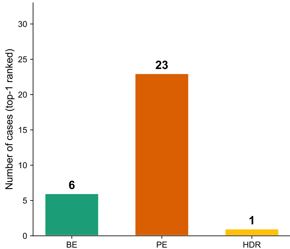
v3 (Multi-nuclease + TOPSIS 6D)
