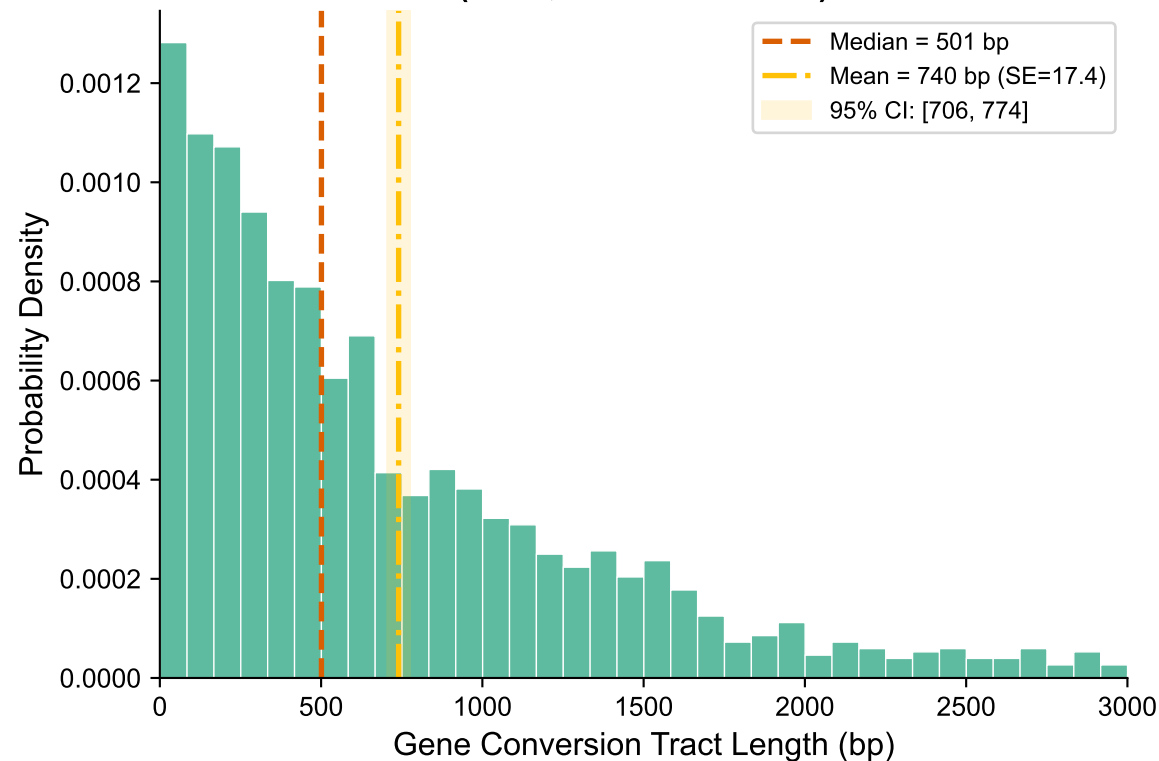
enFnCas9 + cssDNA + iPSC (n=50,000 simulations)
