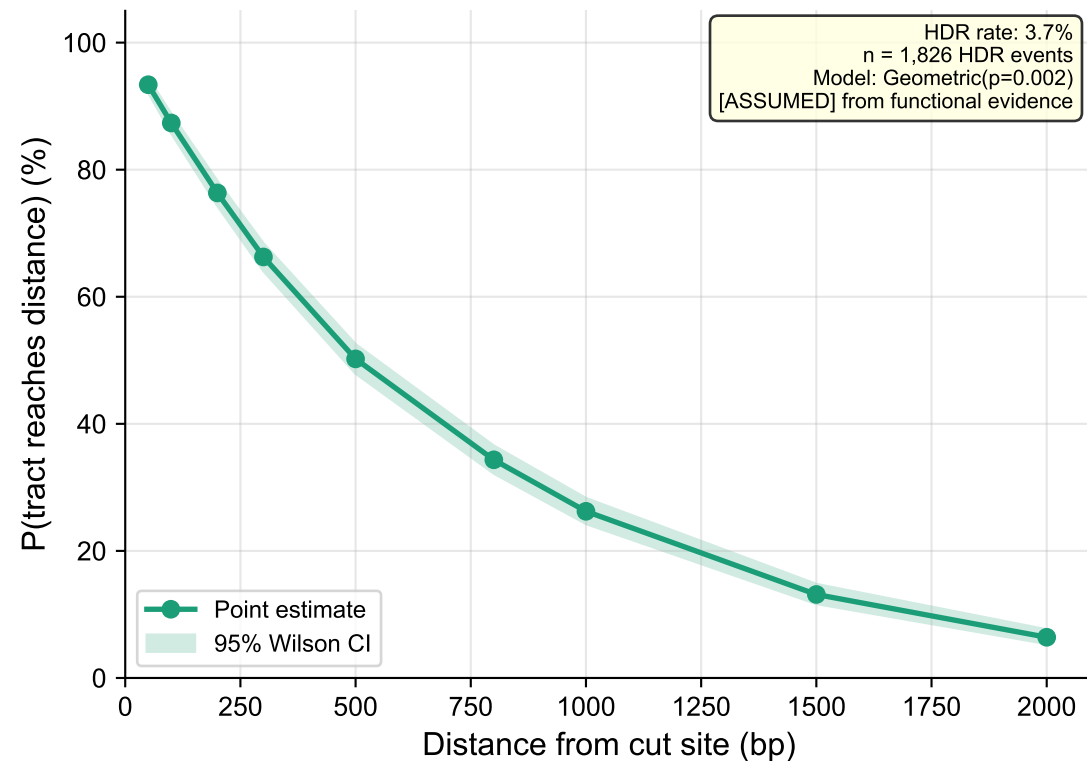
Conversion Probability with 95% Confidence Intervals
