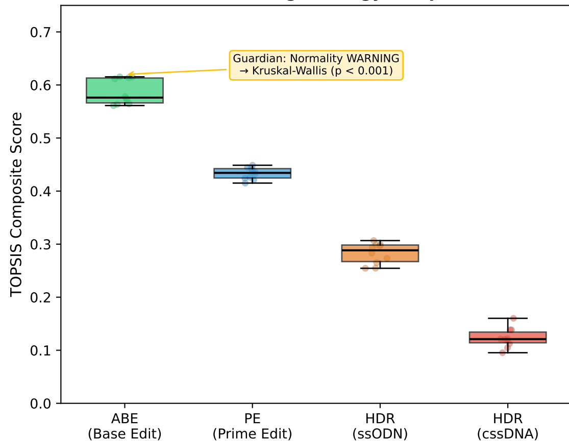
A. CRISPR Editing Strategy Comparison
