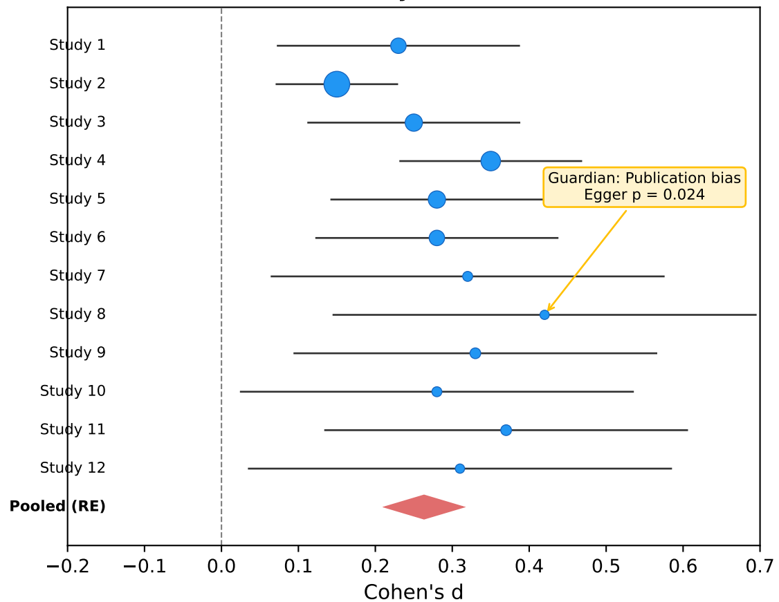
B. Meta-Analysis Forest Plot
