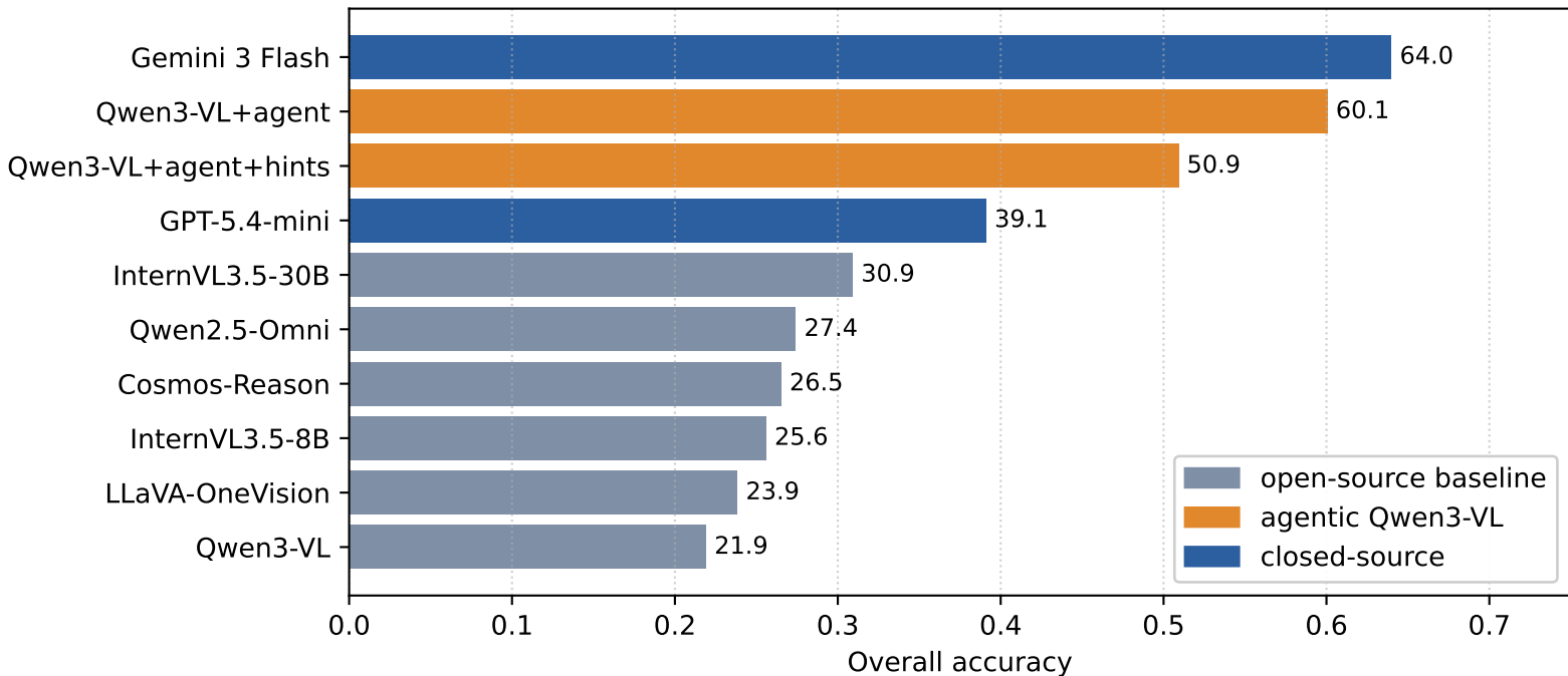
Overall accuracy across 10 model configurations (n = 7 371)
