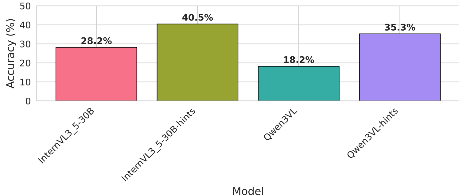
Model Accuracy on the benchmark (w/o Visual)
