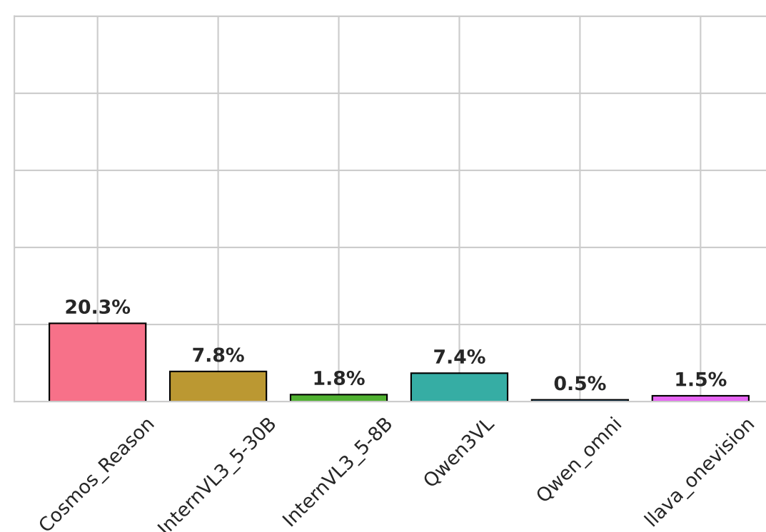
Traffic laws understanding
