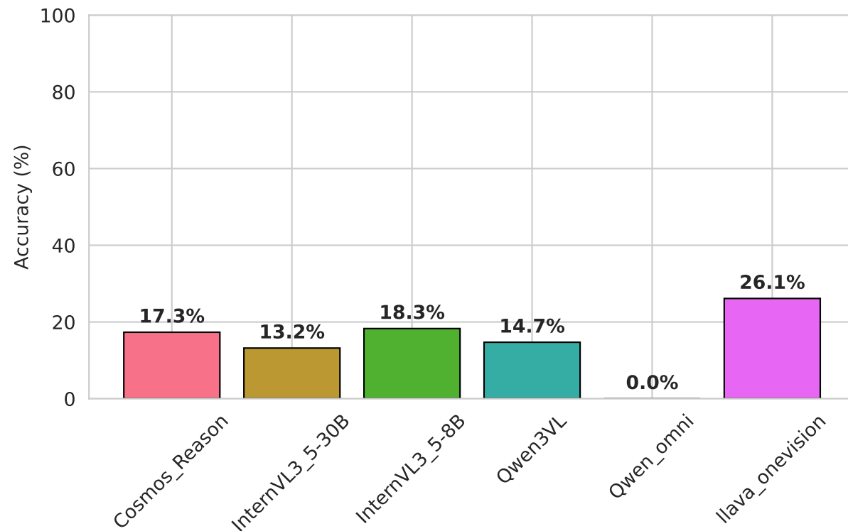
Spatial-temporal understanding
