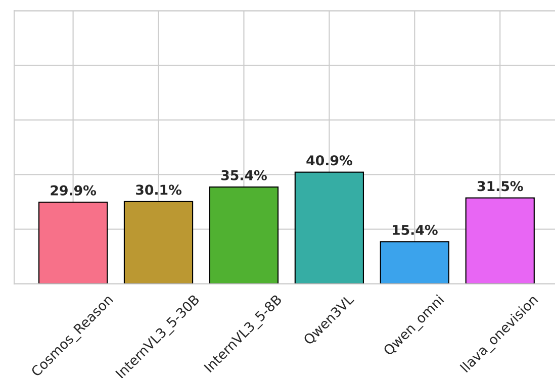
Visual understanding
