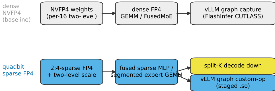
Fig 1. System overview: dense NVFP4 baseline vs quadbit sparse-FP4 path
