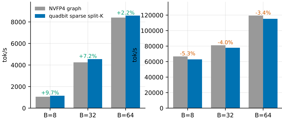
Fig 3. Graph-vs-graph serving: sparse split-K decode beats production NVFP4 Decode (latency-critical) Prefill
