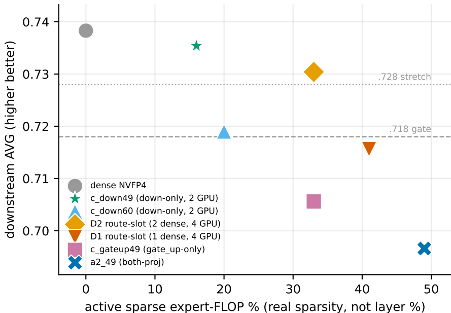
DeepSeek-V4-Flash: training-free sparse-FP4 Pareto c_down49 cleanest 2-GPU; D2 max sparse-FLOP (4-GPU)
