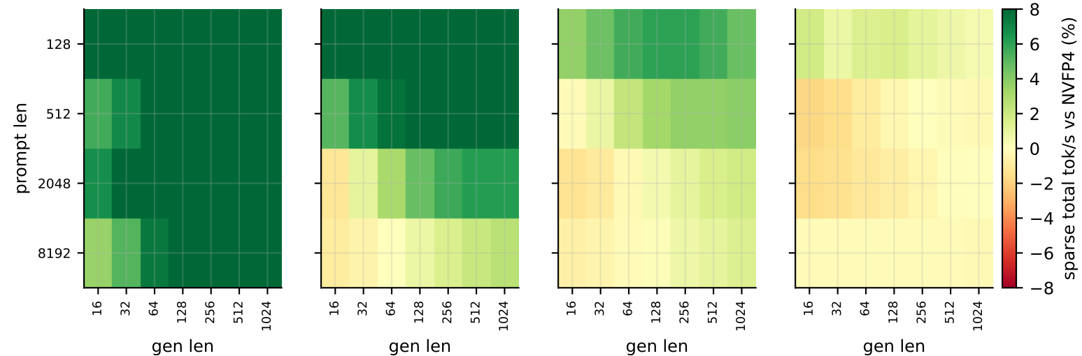
Fig 4. Request-regime crossover (112 regimes): 83 sparse wins / 29 losses / 0 ties
