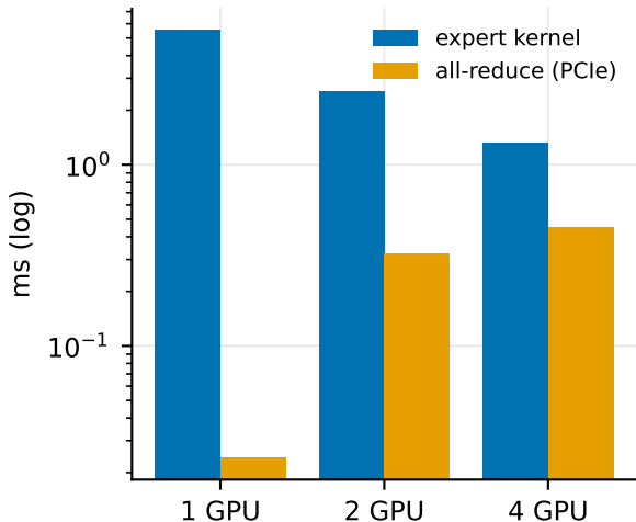
Fig 6. Distributed sparse-FP4 MoE (DeepSeek-V4-Flash, expert-parallel, no NVLink)
