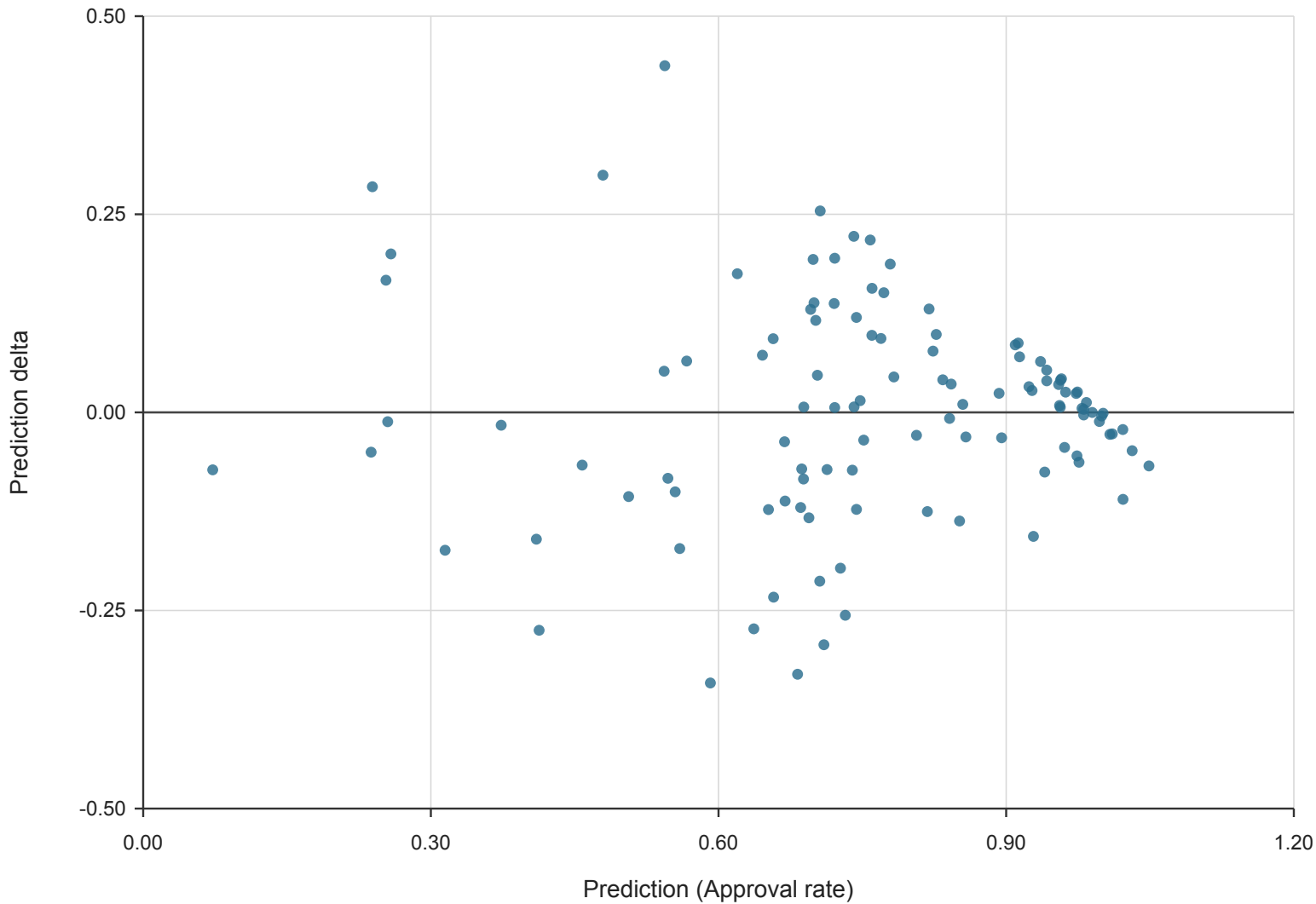
Residuals vs fitted values: no_region
