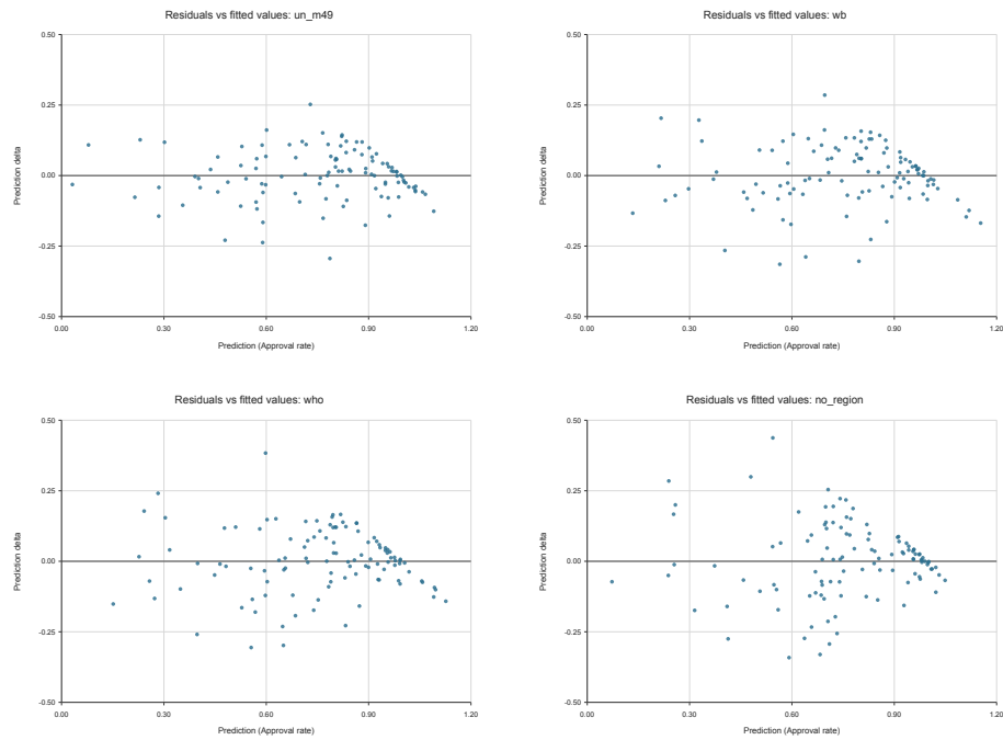
Fig.3. Residuals against fitted approval rates in the four regression specifications. The figures are generated from data/support/residuals_vs_fitted_un_m49.svg , data/support/residuals_vs_fitted_wb.svg , data/support/residuals_vs_fitted_who.svg , and data/support/residuals_vs_fitted_no_region.svg .
