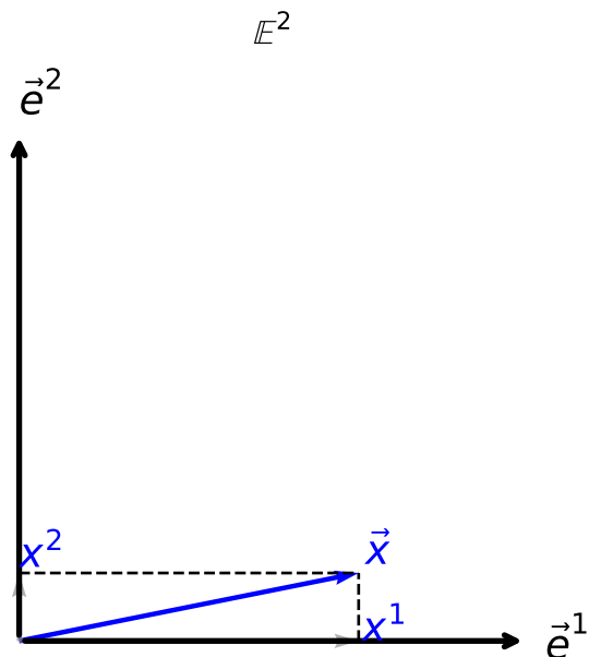
Figure 1: In this diagram, \mathbf{x} is shown along with its projections onto the x^1 and x^2 axes. The dashed lines and gray arrows indicate the coordinate decomposition that defines the Cartesian components.
