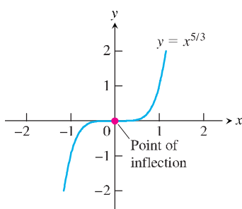
FIGURE 4.26 The graph of f(x) = x^{5/3} has a horizontal tangent at the origin where the concavity changes, although f'' does not exist at x = 0 (Example 3).
