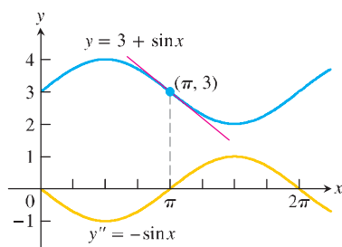
FIGURE 4.25 Using the sign of y'' to determine the concavity of y (Example 2).
