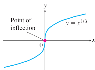
FIGURE 4.28 A point of inflection where y' and y'' fail to exist (Example 5).
