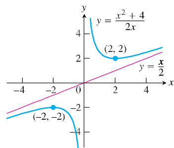
FIGURE 4.31 The graph of y = \frac{x^2 + 4}{2x} (Example 9).
