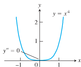
FIGURE 4.27 The graph of y = x^4 has no inflection point at the origin, even though y'' = 0 there (Example 4).
