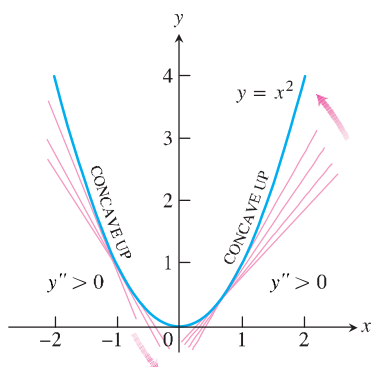
FIGURE 4.24 The graph of f(x) = x^2 is concave up on every interval (Example 1b).
