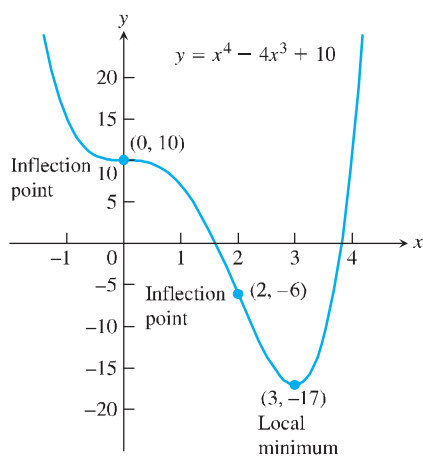
FIGURE 4.29 The graph of f(x) = x^4 - 4x^3 + 10 (Example 7).
