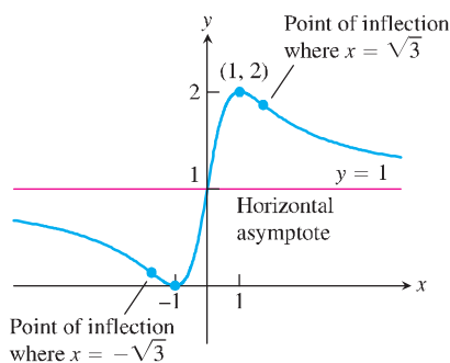
FIGURE 4.30 The graph of y = \frac{(x+1)^2}{1+x^2} (Example 8).
