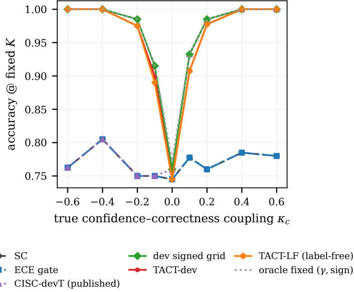
Figure 2: Main result on the confidence-usage frontier. TACT-dev and the fully label-free TACT-LF track the signed oracle across the sweep; CISC-devT and the ECE gate sit at the SC floor for all \kappa < 0 .
