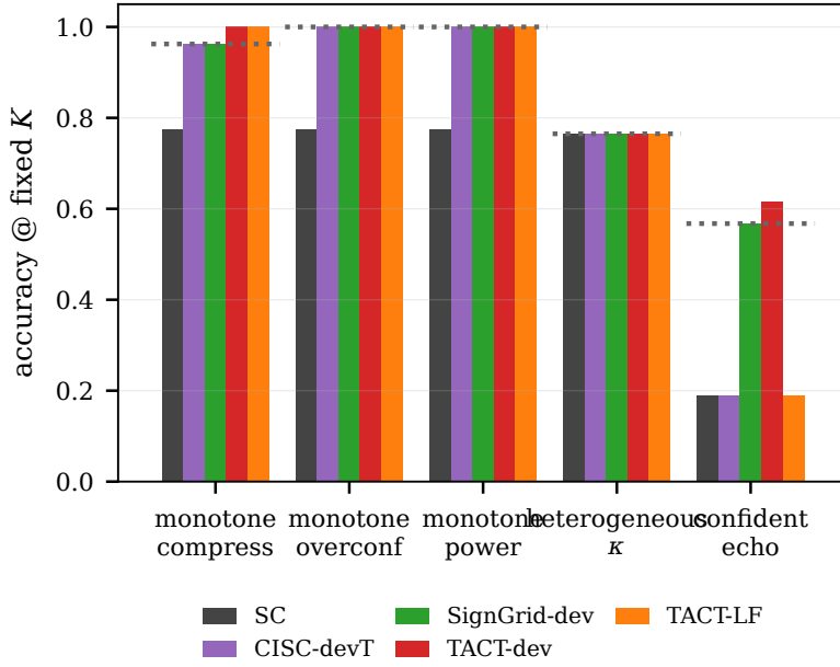
Figure 3: Adversarial regimes. Dotted line: the oracle over raw-value weights. Left group of bars: rank invariance beats that family under compression; right: the labeled variant counters the confident echo while the label-free variant alarms and refuses.
