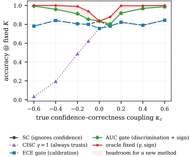
Figure 1: The pre-measured problem statement: accuracy of baseline confidence policies at fixed K=15 as the true coupling \kappa varies. A trivial sign-corrected AUC gate (green) nearly saturates the homogeneous sweep; the headroom for any new method (shaded) concentrates in the mid-range and, off this plot, in distortion, heterogeneity, and label-free cells.
