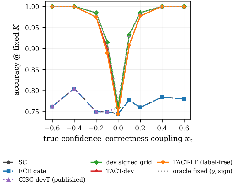
Figure 2: Main result on the confidence-usage frontier. TACT-dev and the fully label-free TACT-LF track the signed oracle across the sweep; CISC-devT and the ECE gate sit at the SC floor for all \kappa < 0 .
