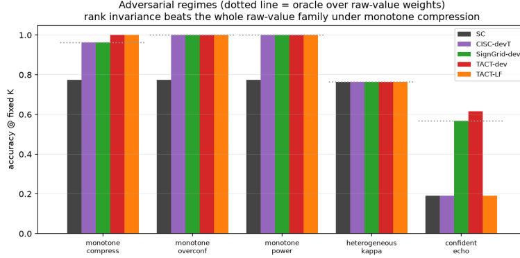
Figure 3: Adversarial regimes. Dotted line: the oracle over raw-value weights. Left group of bars: rank invariance beats that family under compression; right: the labeled variant counters the confident echo while the label-free variant alarms and refuses.
