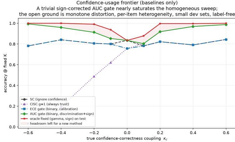
Figure 1: The pre-measured problem statement: accuracy of baseline confidence policies at fixed K=15 as the true coupling \kappa varies. A trivial sign-corrected AUC gate (green) nearly saturates the homogeneous sweep; the headroom for any new method (shaded) concentrates in the mid-range and, off this plot, in distortion, heterogeneity, and label-free cells.
