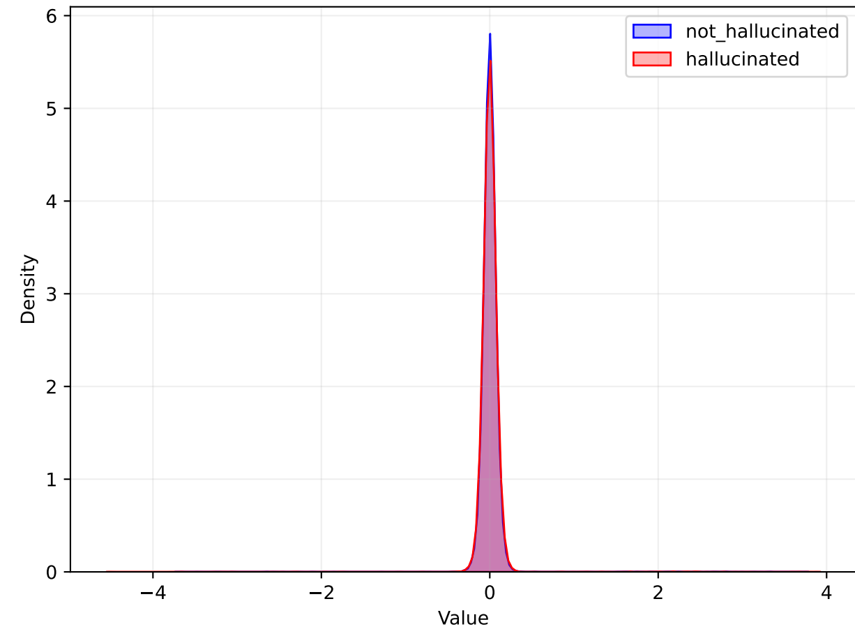
MLP Distribution
