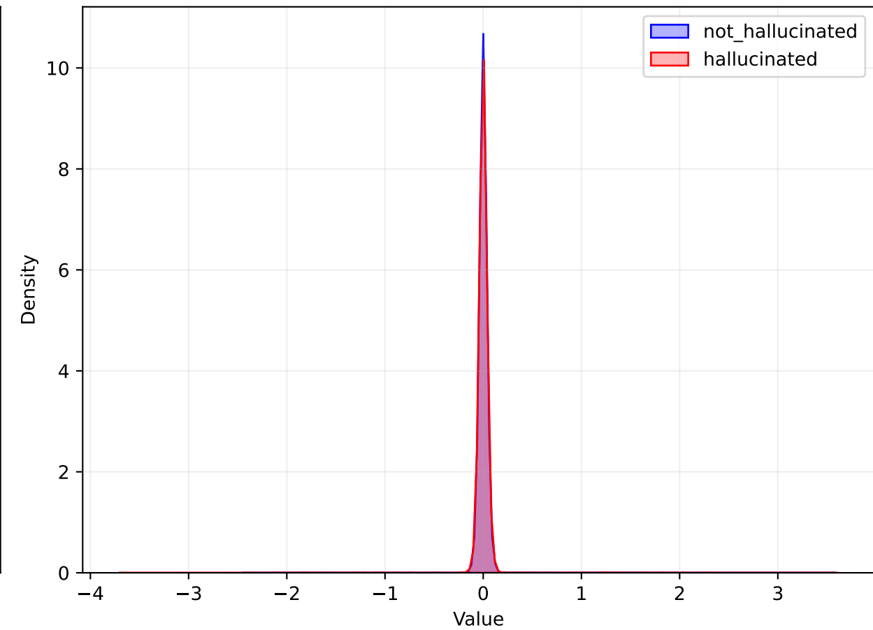
MLP Distribution
