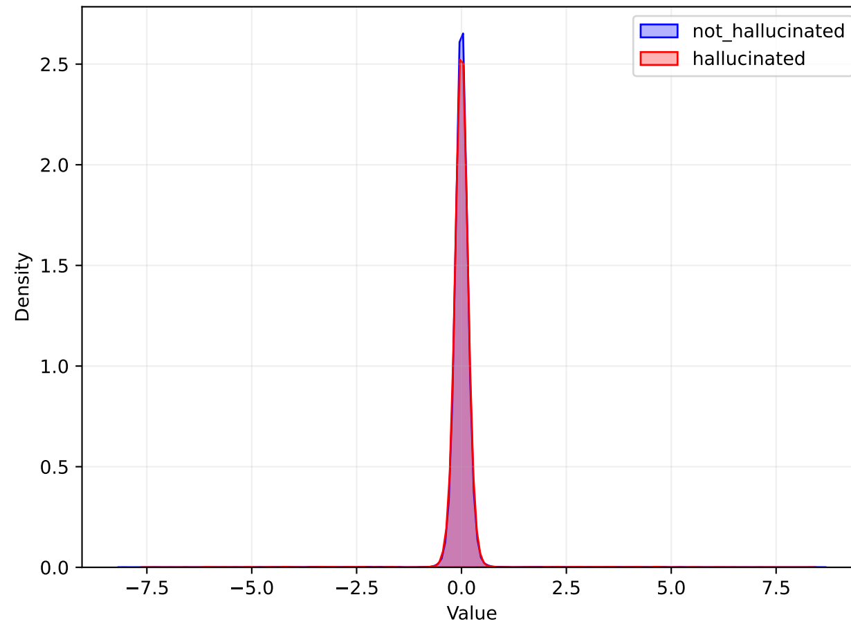
ATTN Distribution
