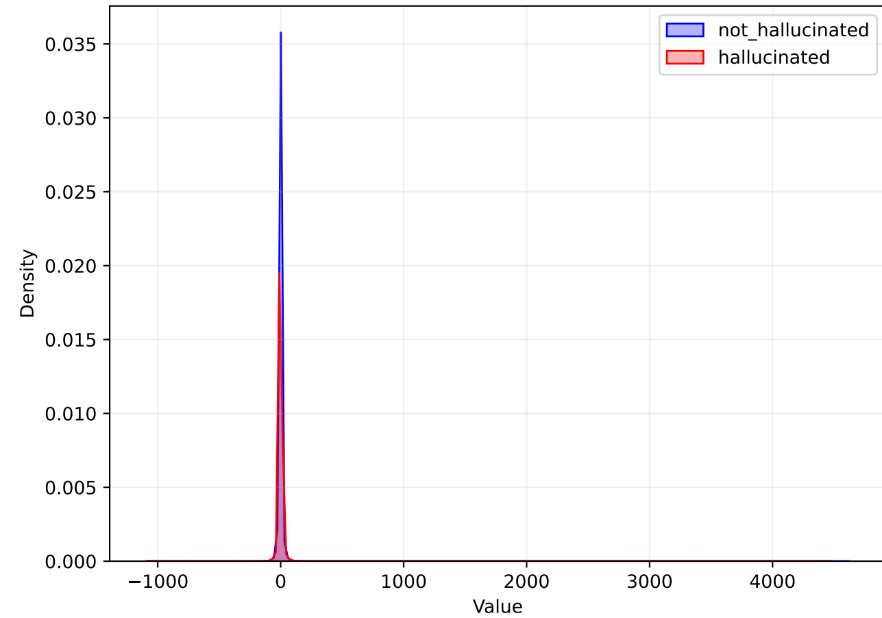
HIDDEN Distribution
