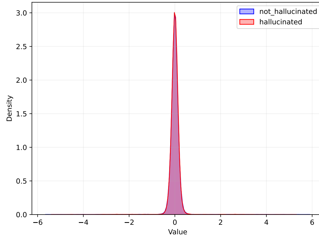
ATTN Distribution
