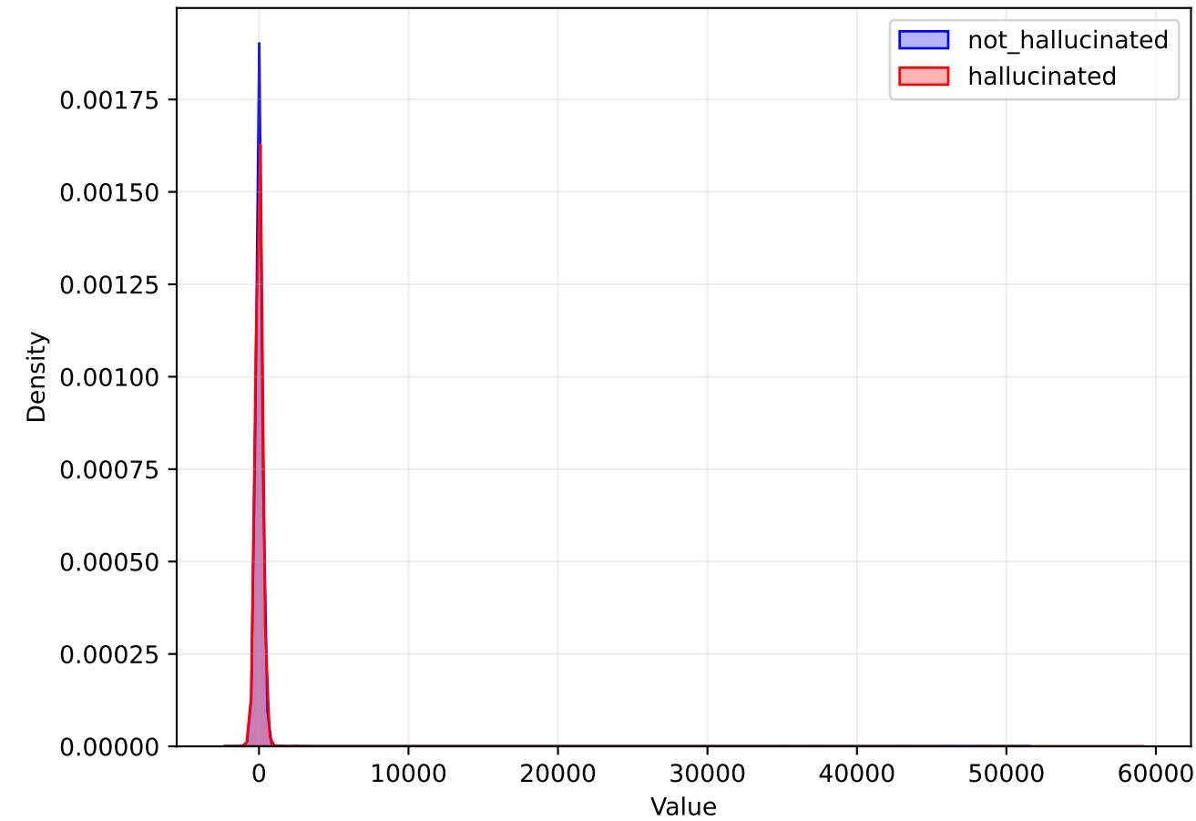
HIDDEN Distribution
