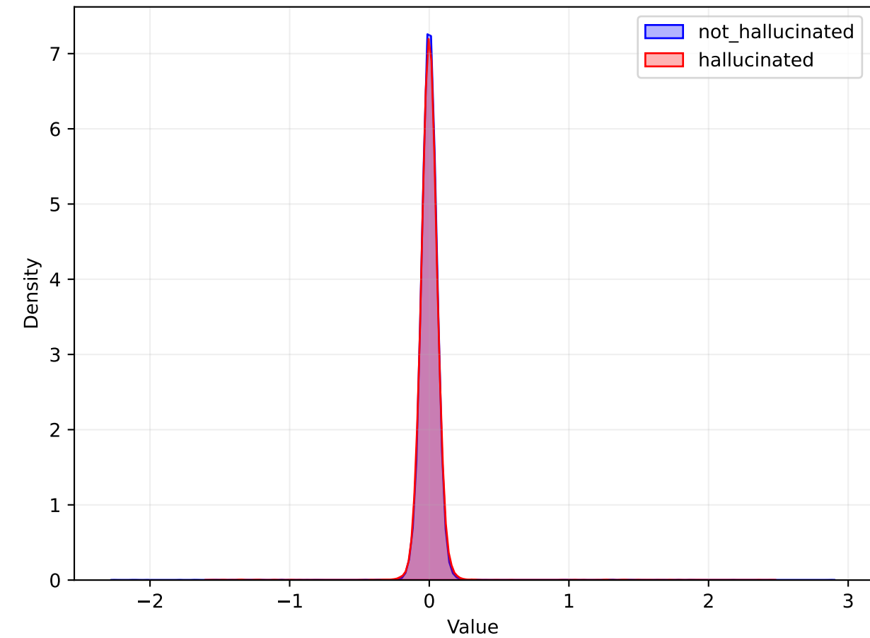
MLP Distribution
