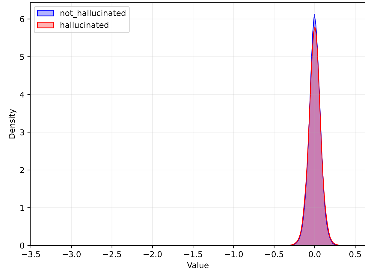
MLP Distribution
