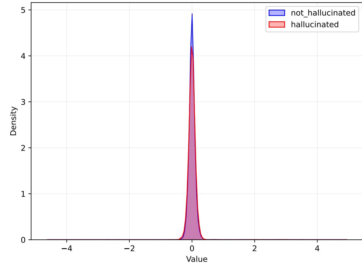
MLP Distribution
