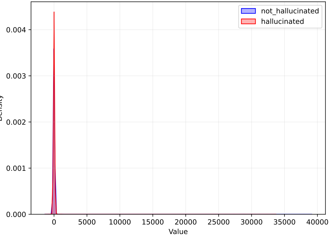
HIDDEN Distribution
