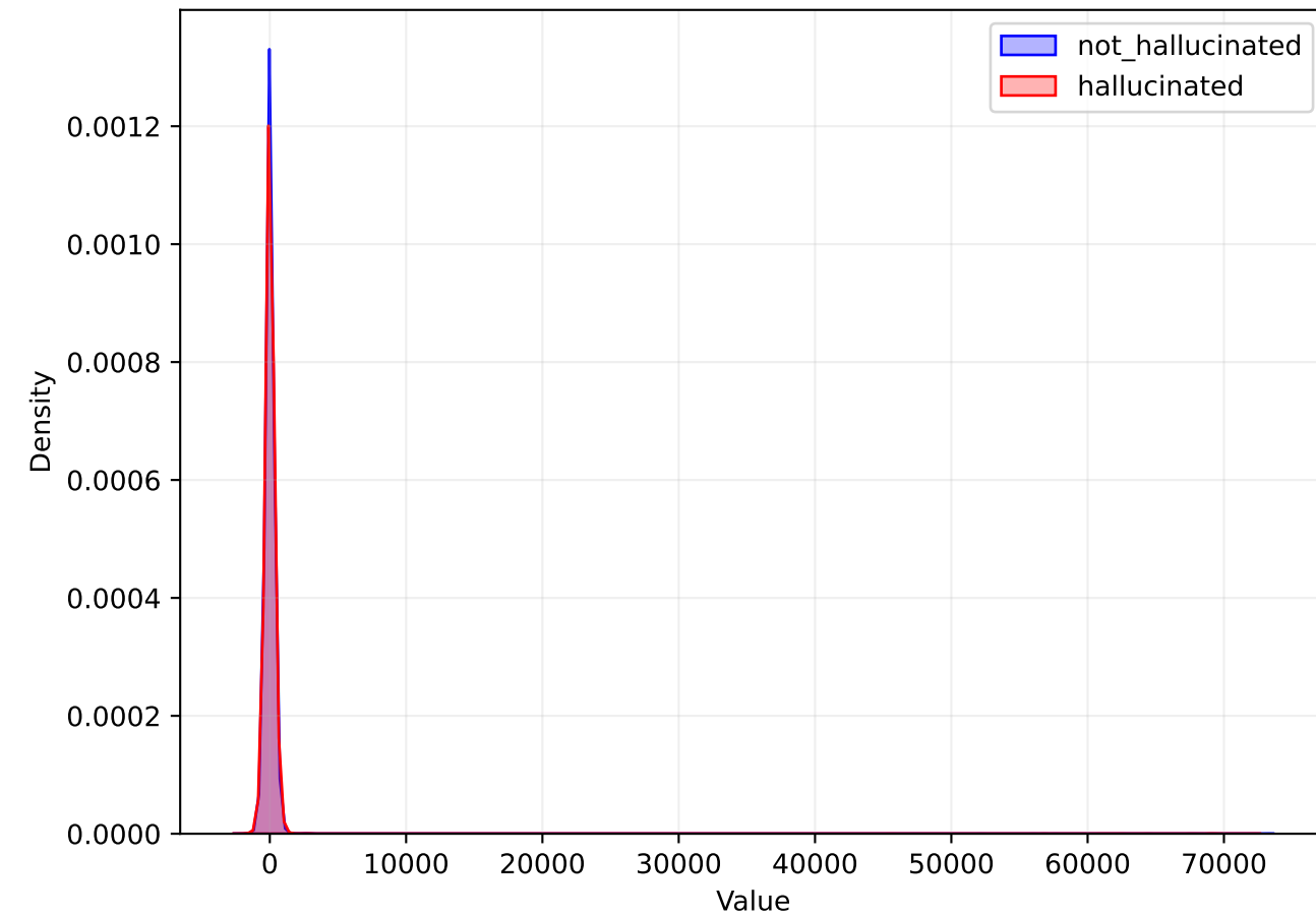
HIDDEN Distribution
