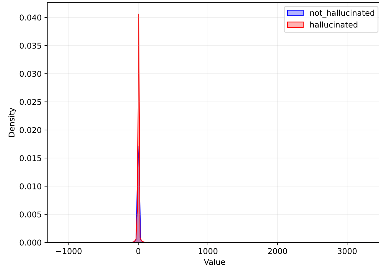
HIDDEN Distribution
