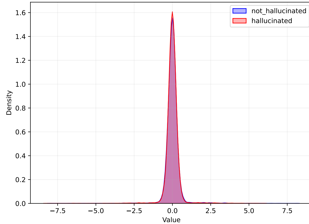
ATTN Distribution
