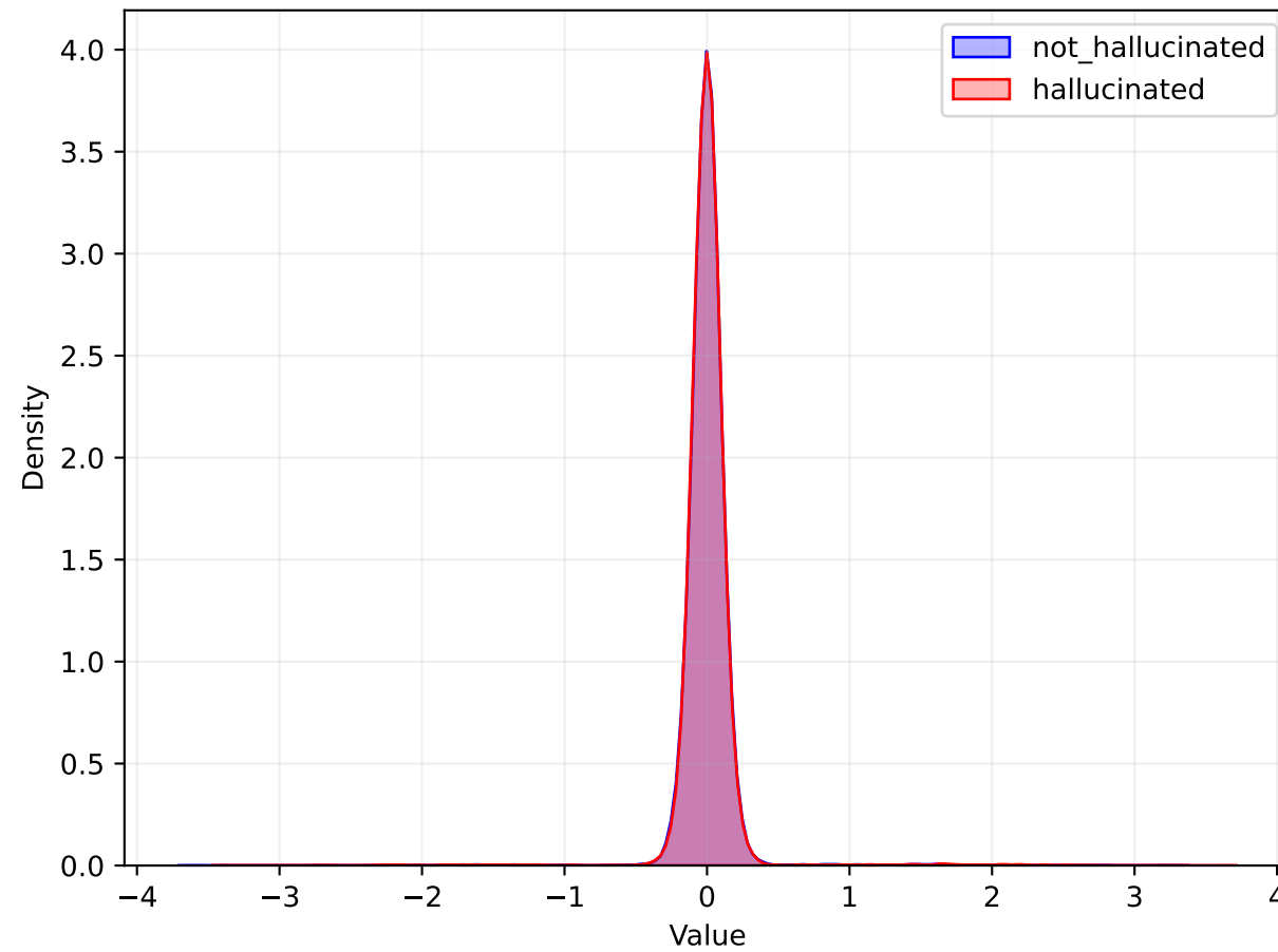
ATTN Distribution
