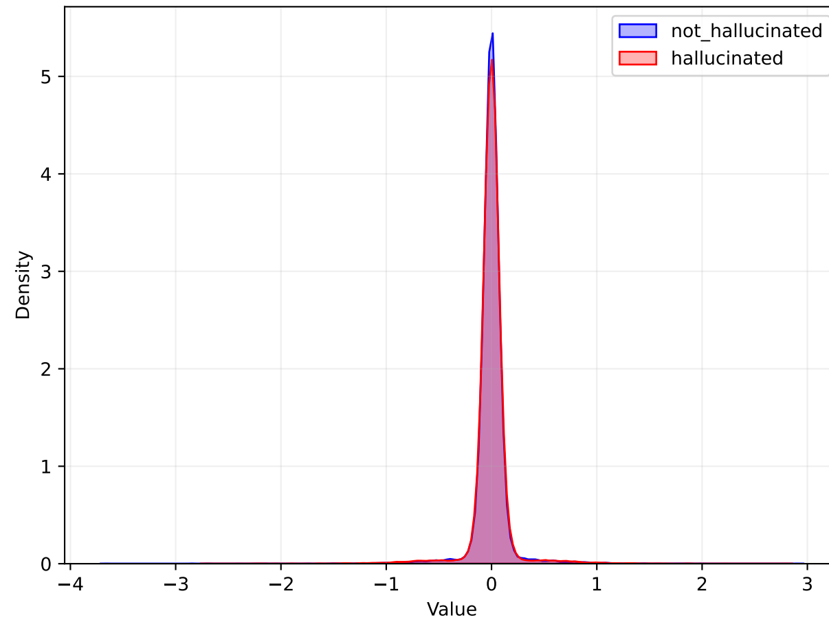
ATTN Distribution
