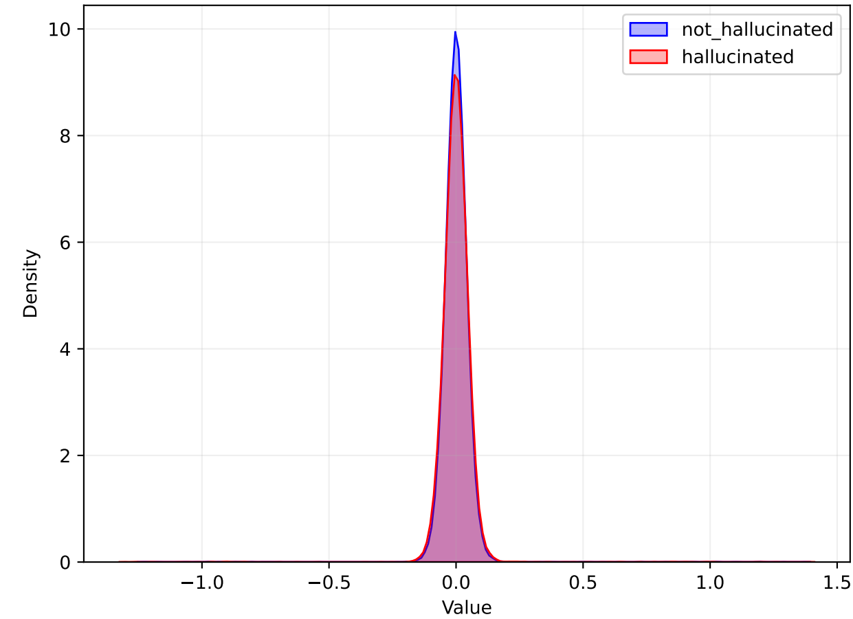
MLP Distribution
