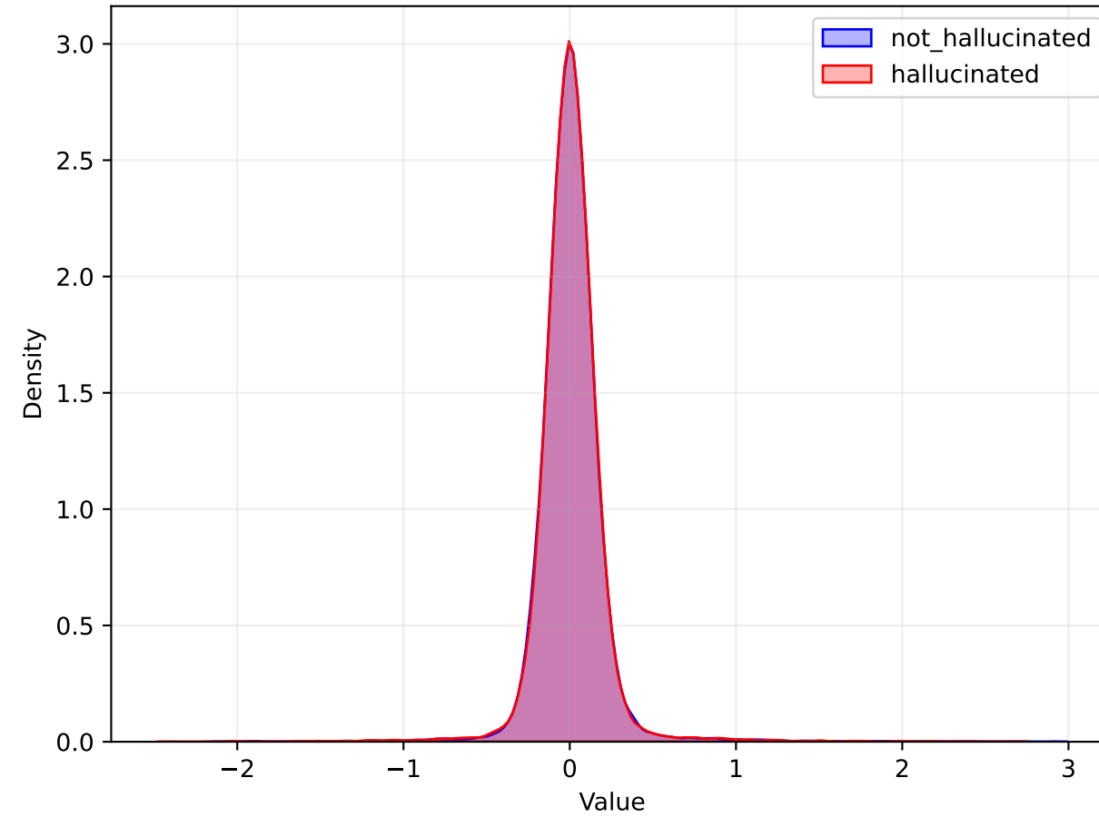
ATTN Distribution
