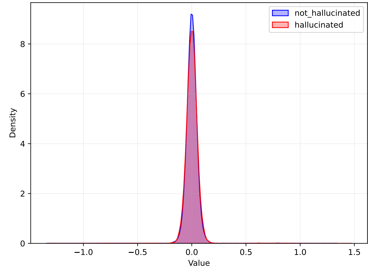
MLP Distribution
