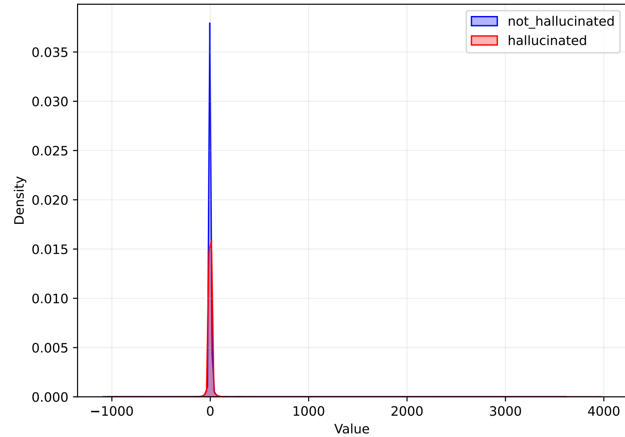
HIDDEN Distribution
