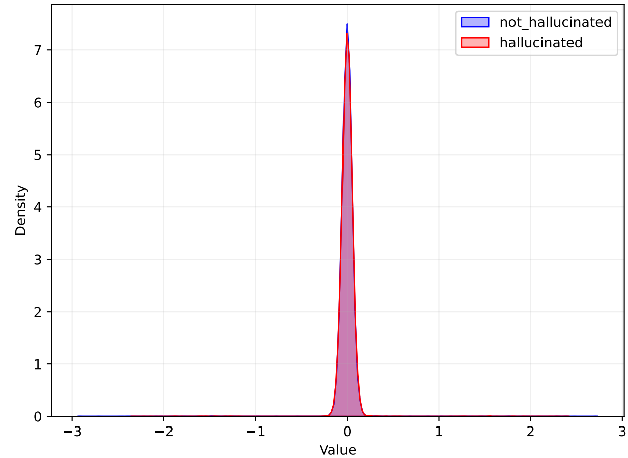
MLP Distribution
