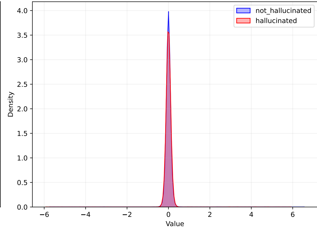
MLP Distribution
