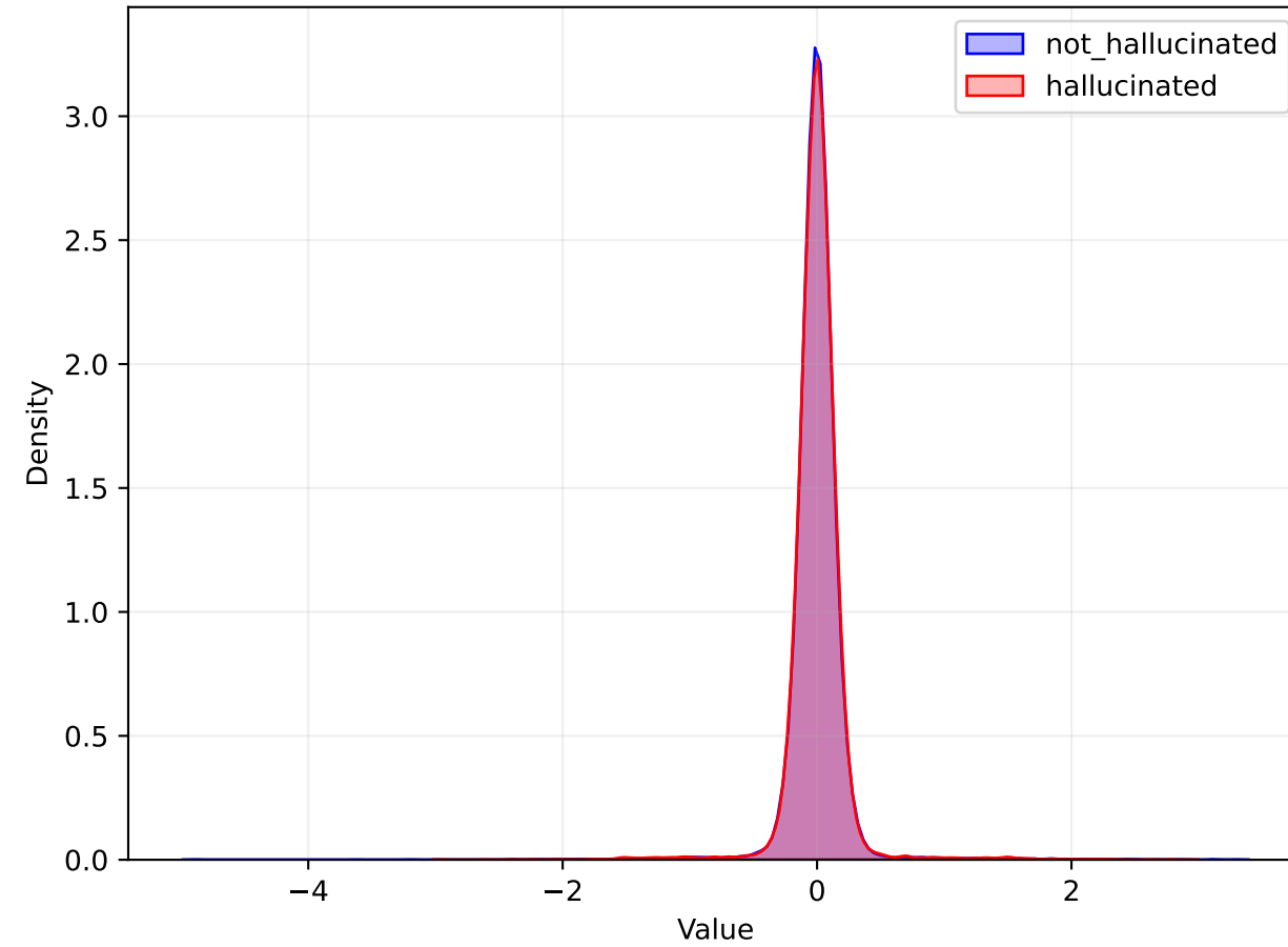
ATTN Distribution
