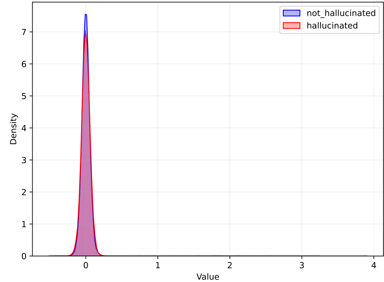
MLP Distribution
