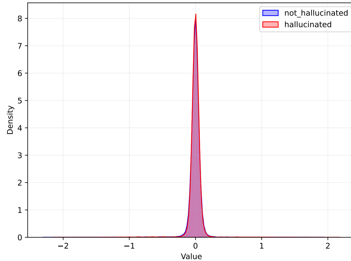
ATTN Distribution
