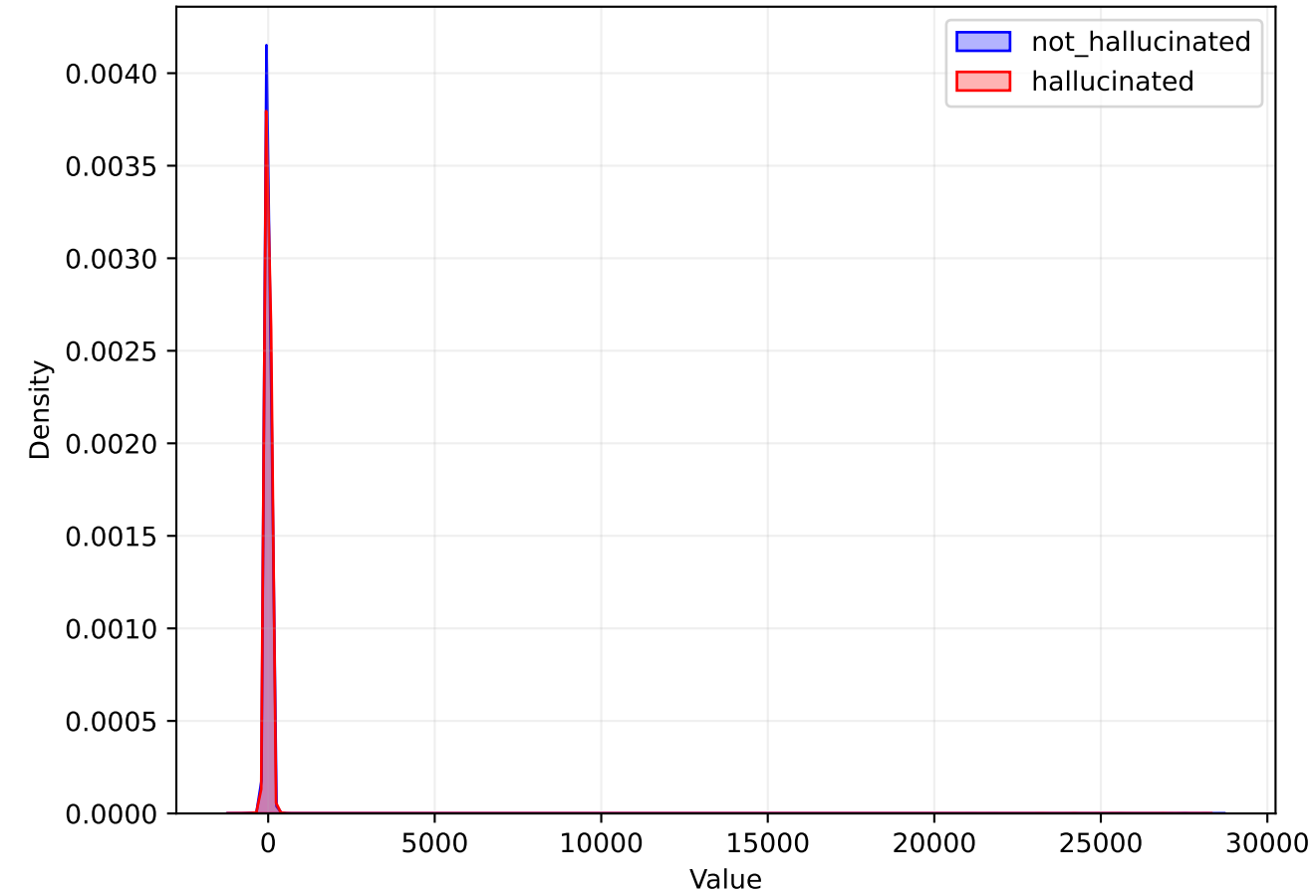
HIDDEN Distribution
