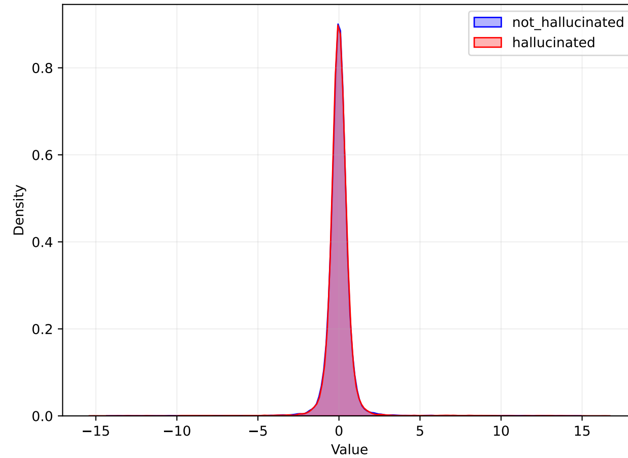
ATTN Distribution
