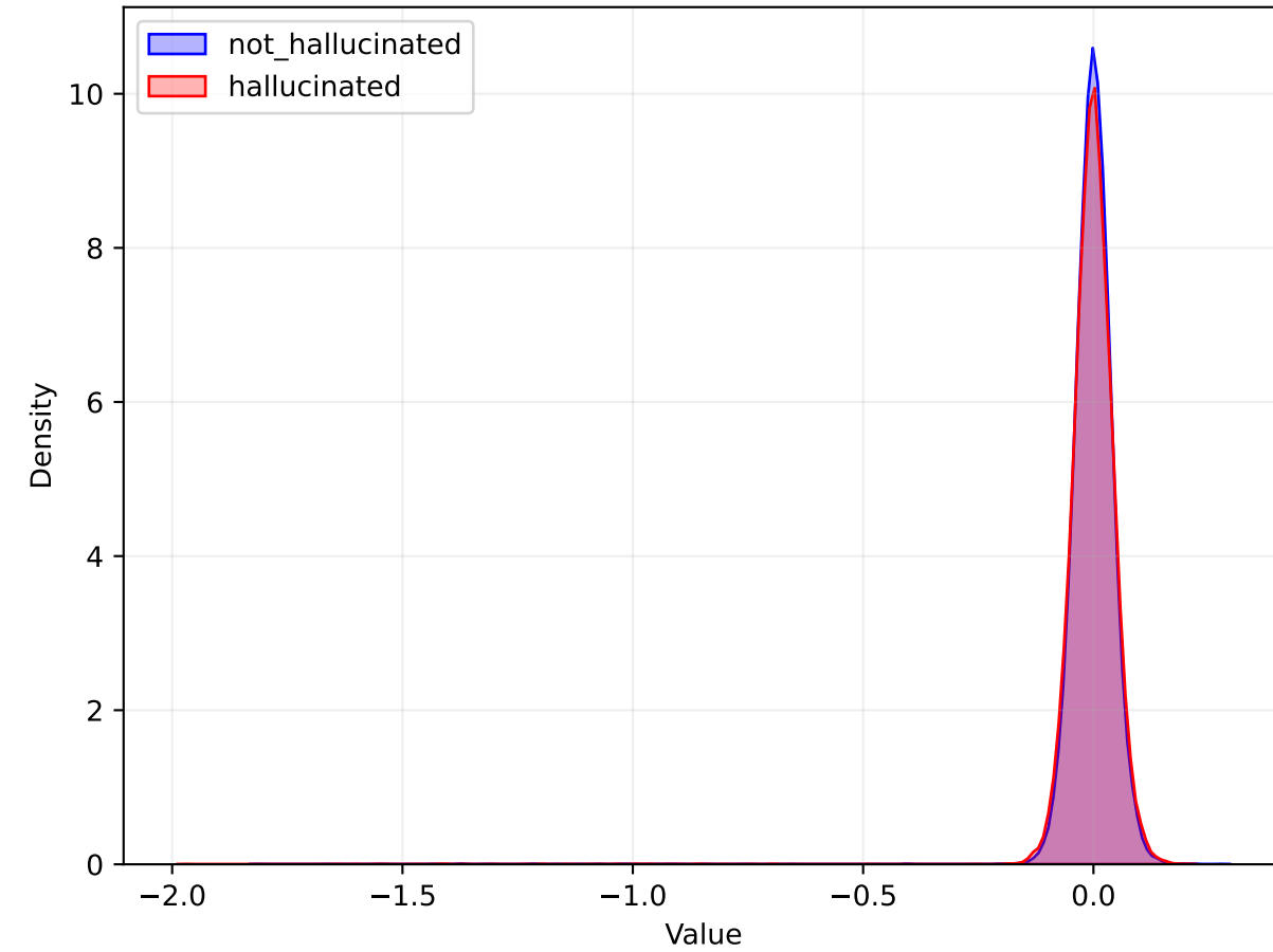
MLP Distribution
