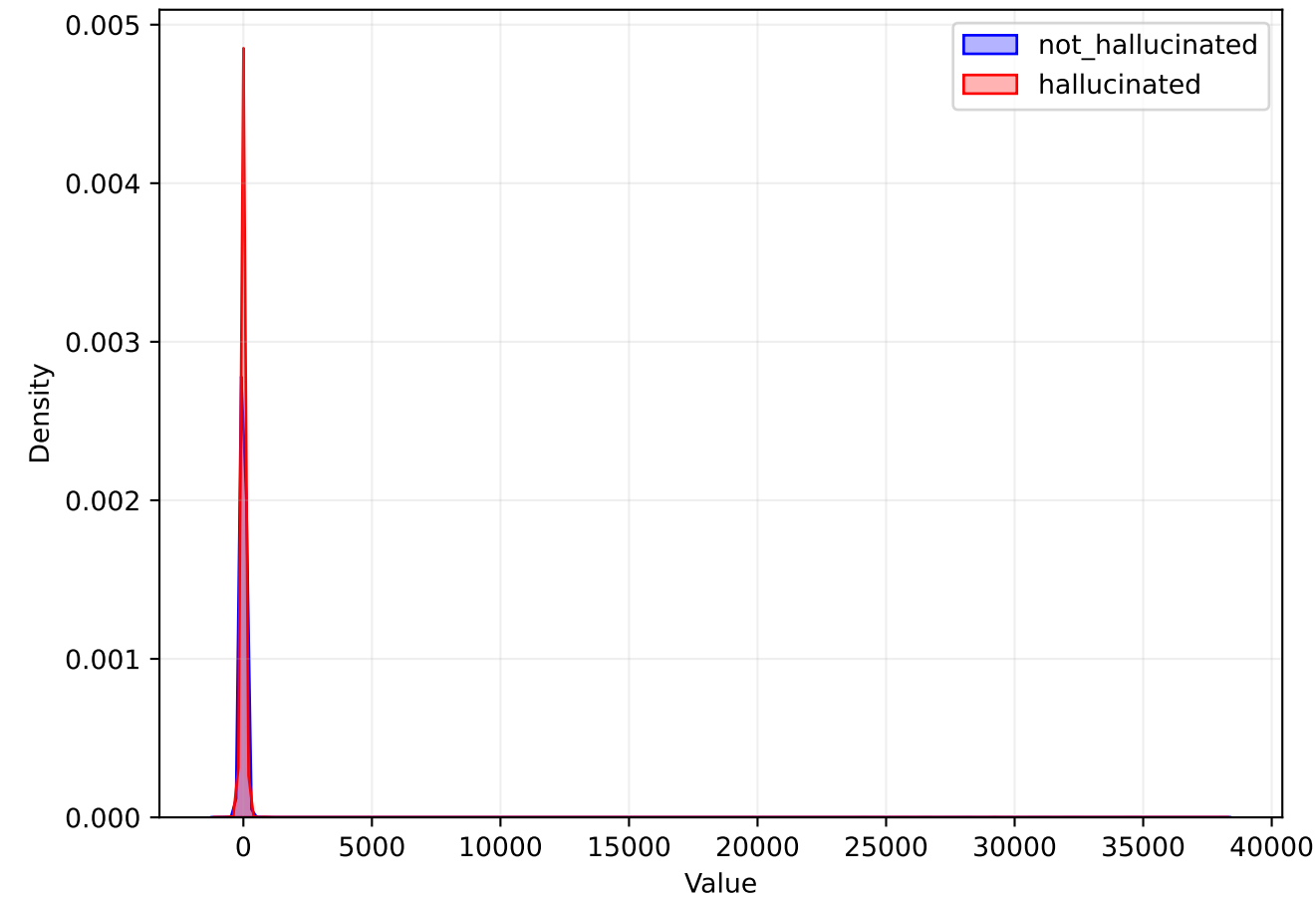
HIDDEN Distribution
