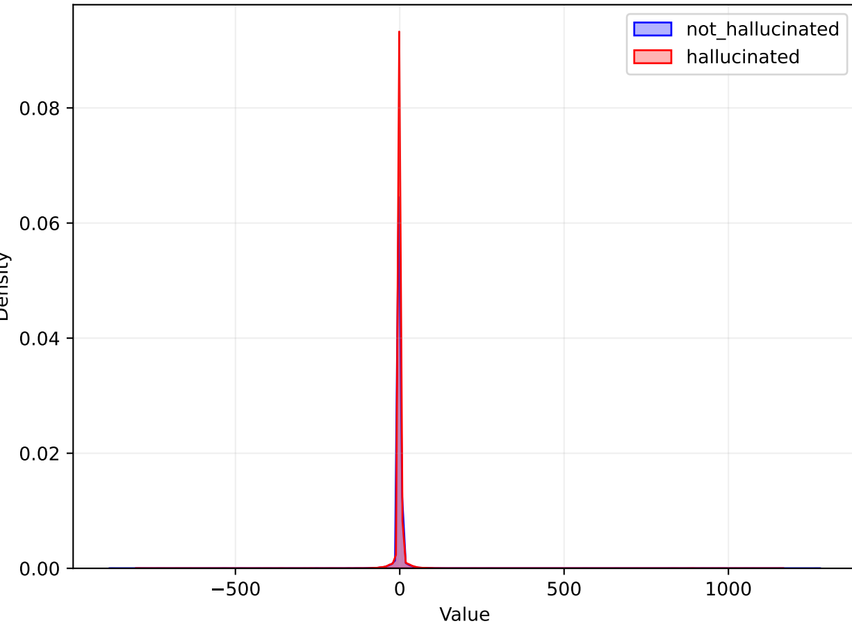
HIDDEN Distribution
