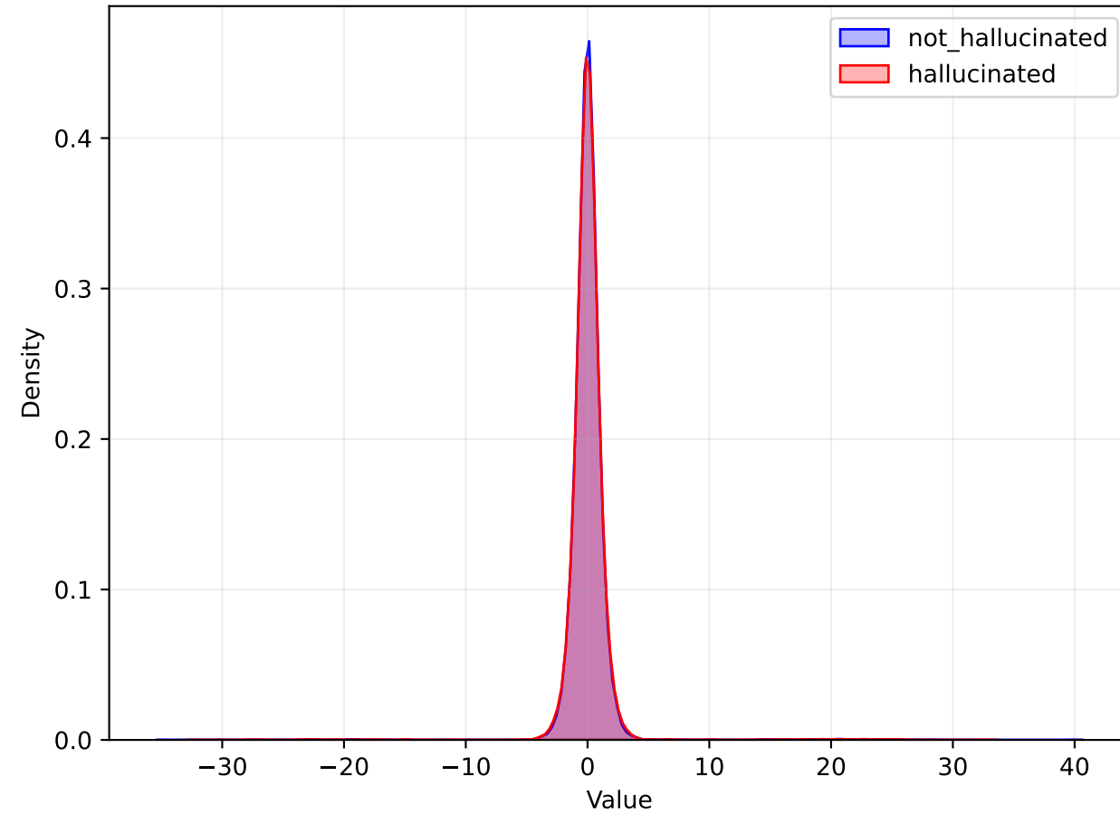
ATTN Distribution
