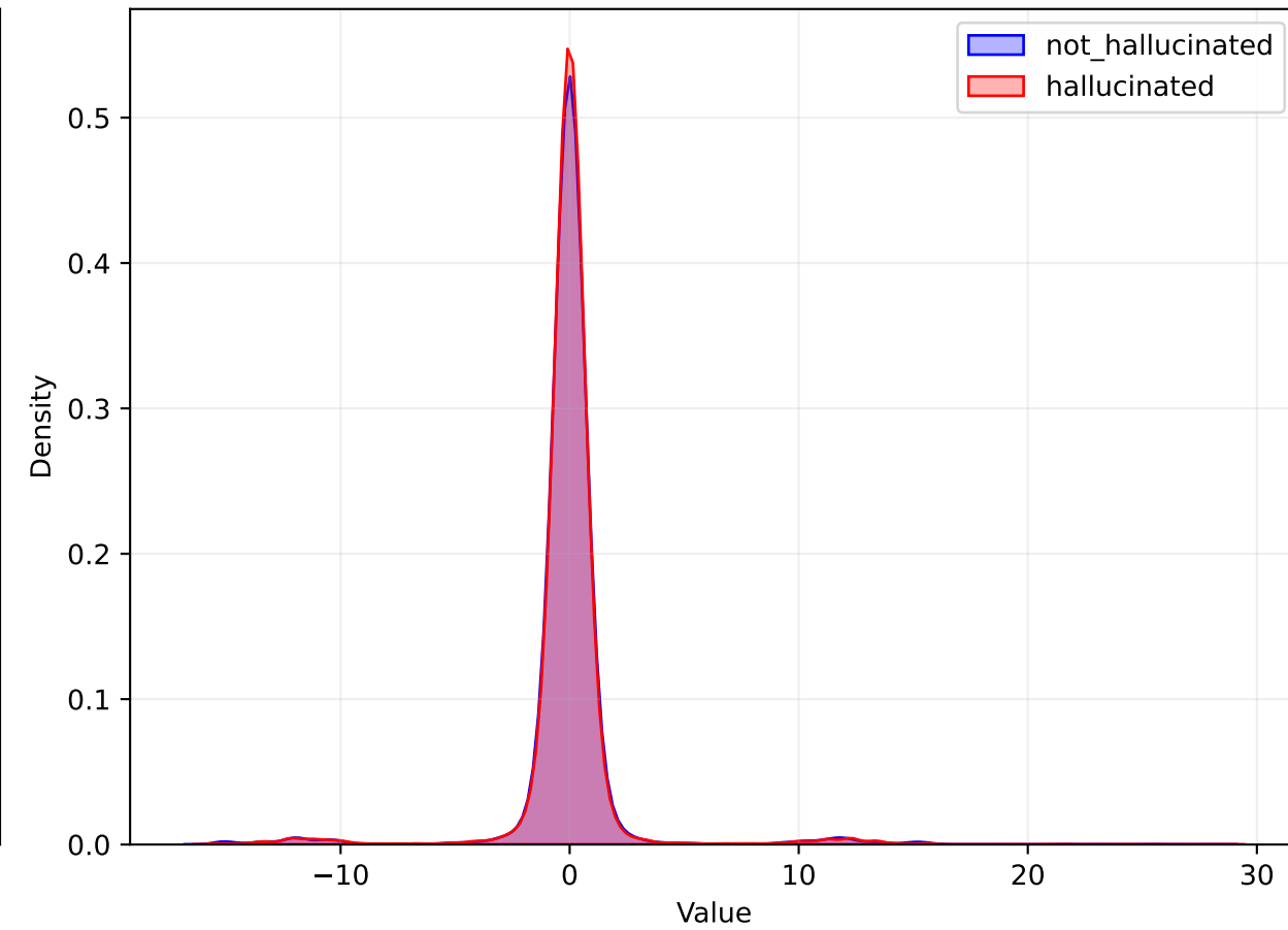
ATTN Distribution
