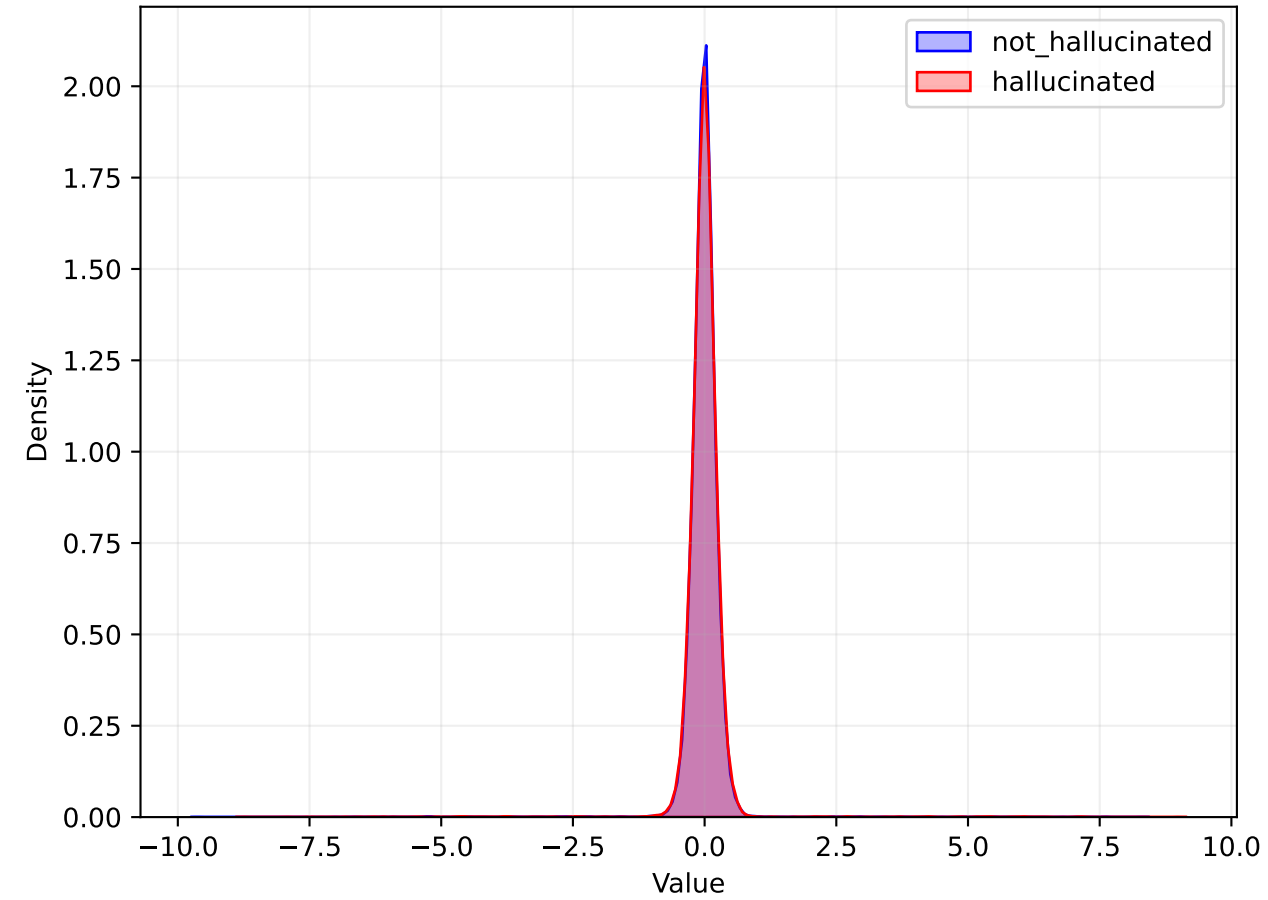
ATTN Distribution
