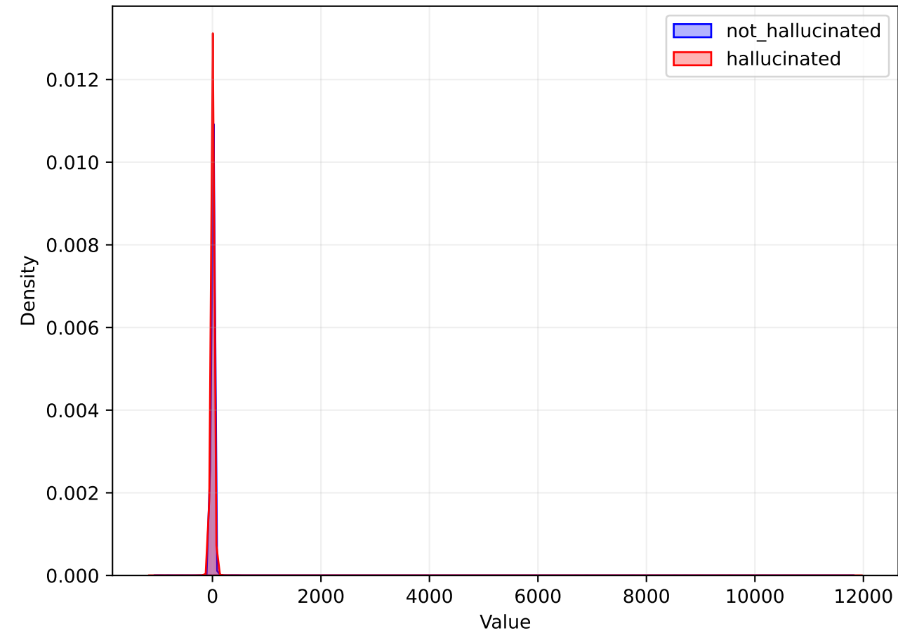
HIDDEN Distribution
