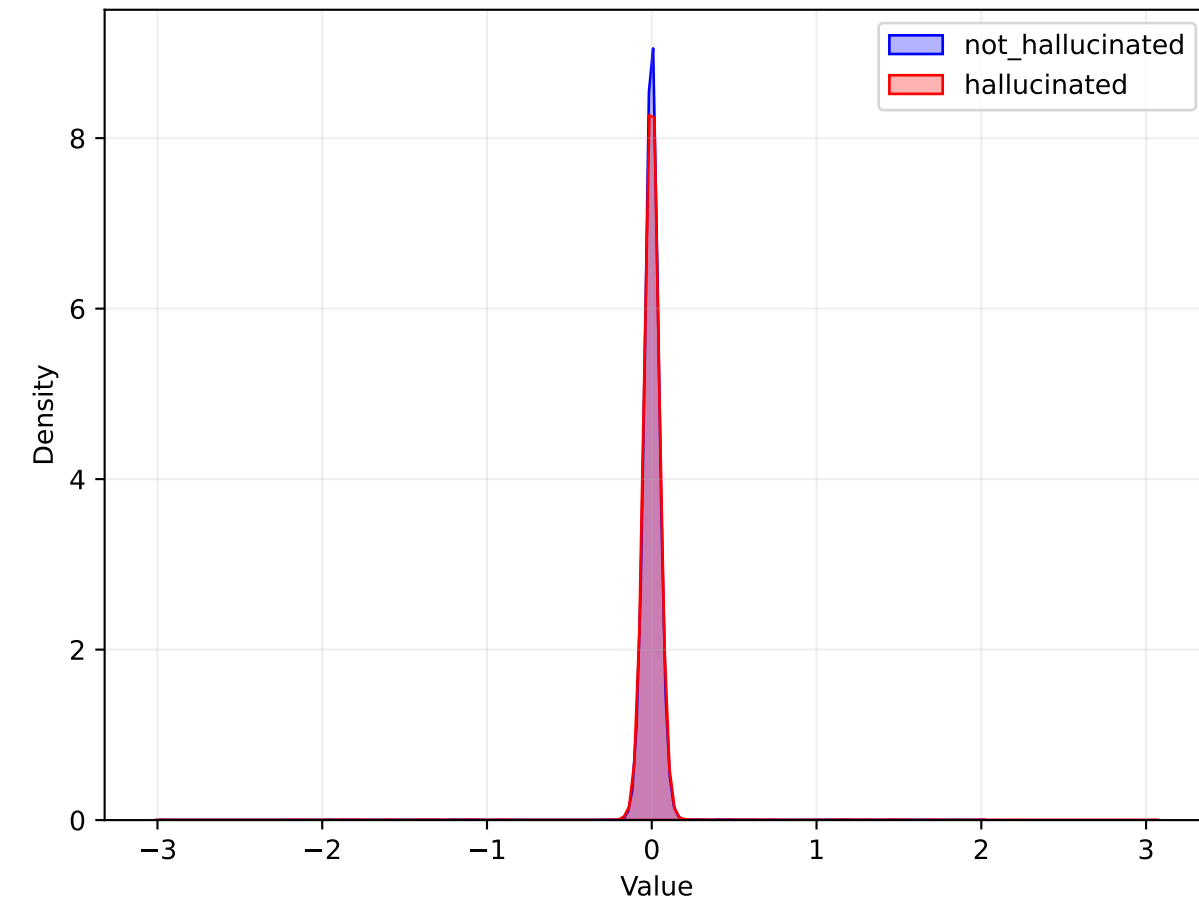
MLP Distribution
