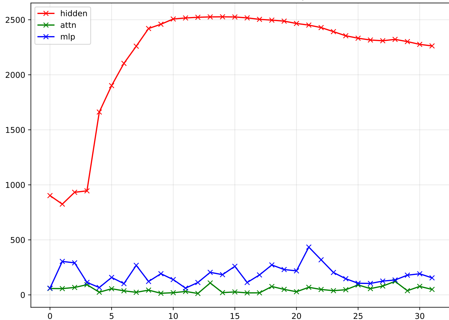
Kurtosis - Hallucinated Only
