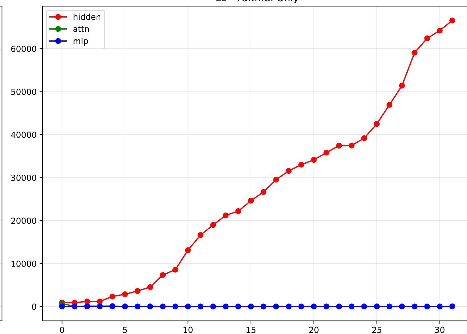
L2 - Faithful Only
