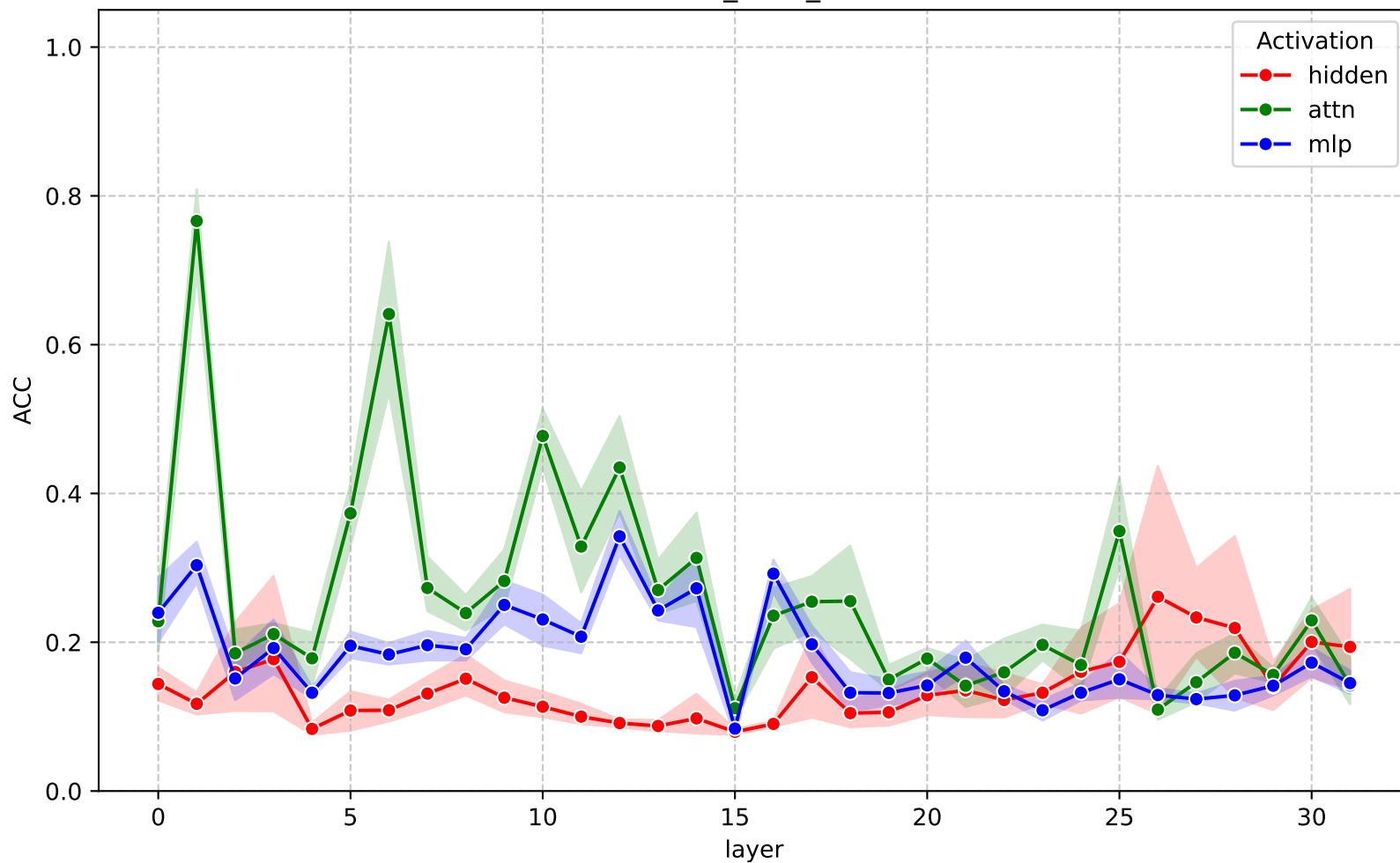
ACC across layers - gemma-3-4b-it (cross_cquad_ffn)
