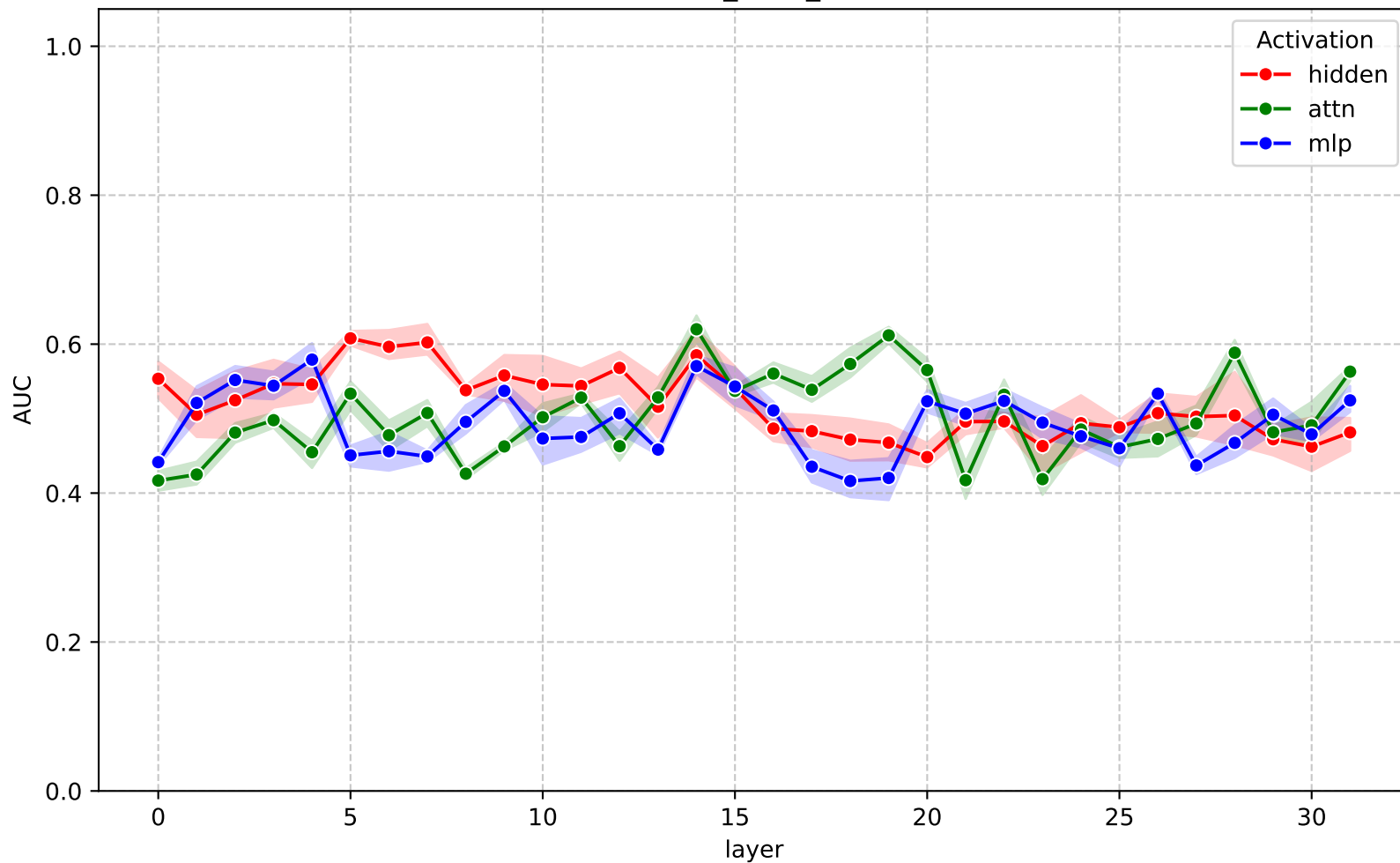
AUC across layers - gemma-3-4b-it (cross_cquad_ffn)
