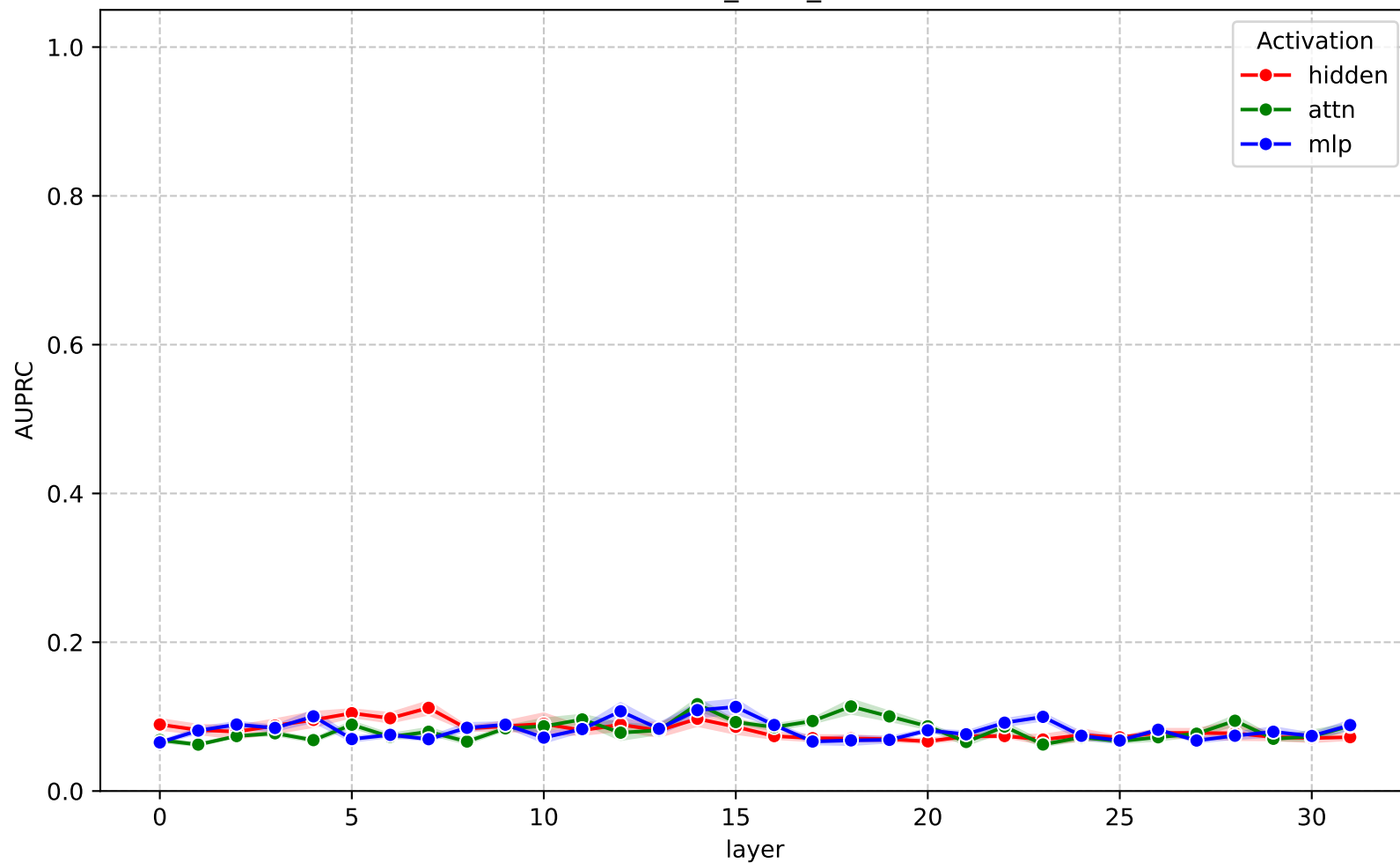
AUPRC across layers - gemma-3-4b-it (cross_cquad_ffn)
