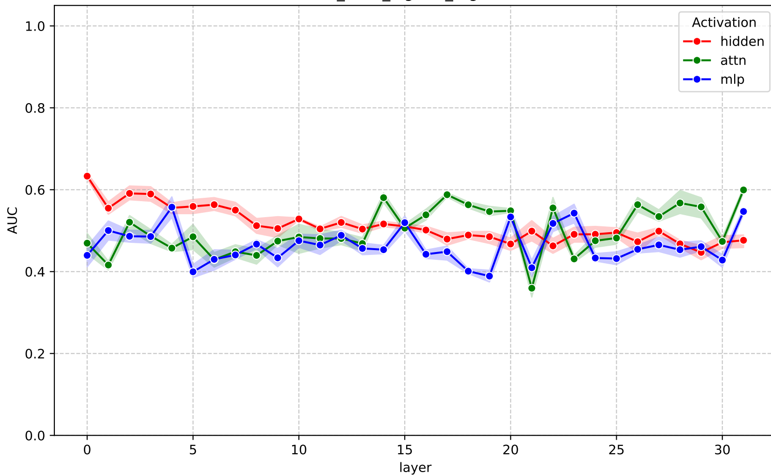
AUC across layers - gemma-3-4b-it (cross_cquad_logistic_regression)
