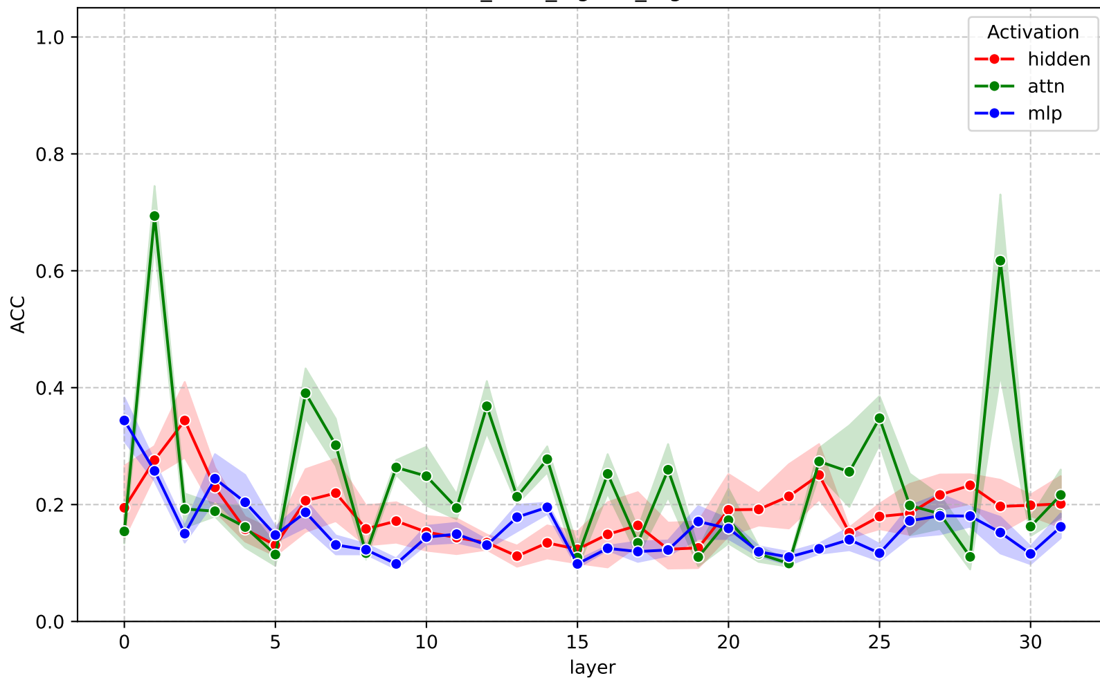
ACC across layers - gemma-3-4b-it (cross_cquad_logistic_regression)
