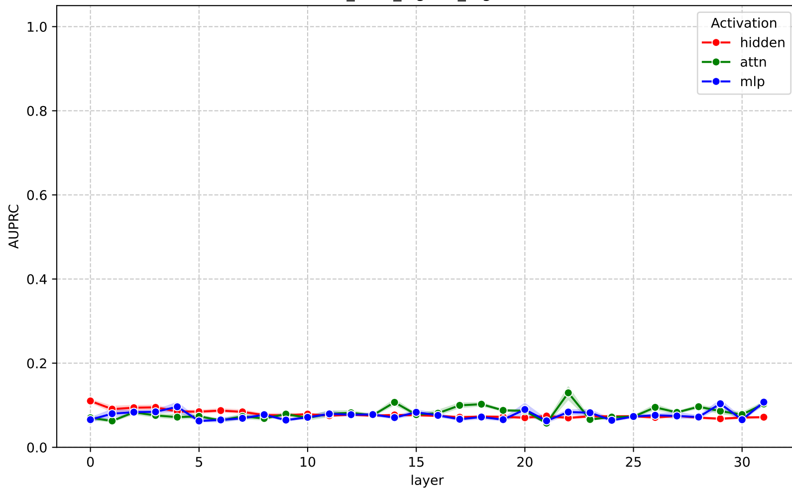
AUPRC across layers - gemma-3-4b-it (cross_cquad_logistic_regression)
