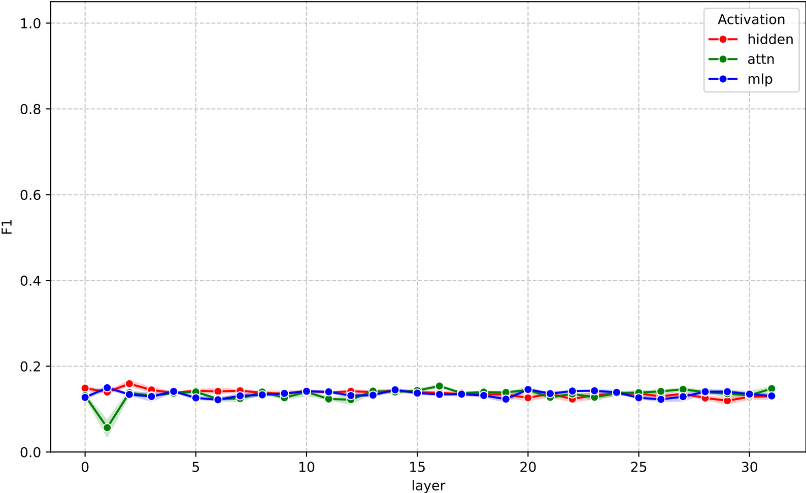
F1 across layers - gemma-3-4b-it (cross_cquad_logistic_regression)
