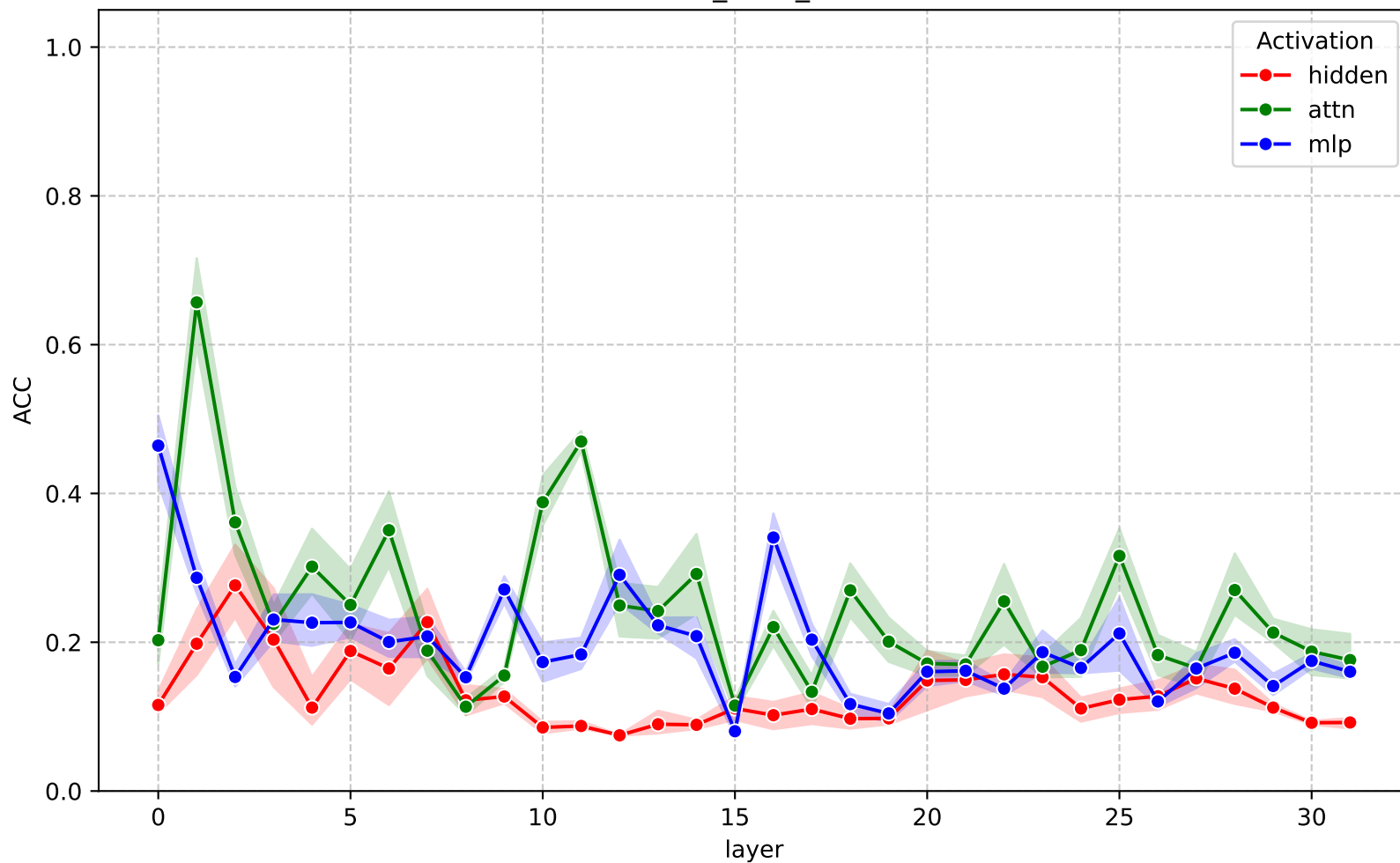
ACC across layers - gemma-3-4b-it (cross_cquad_svm)
