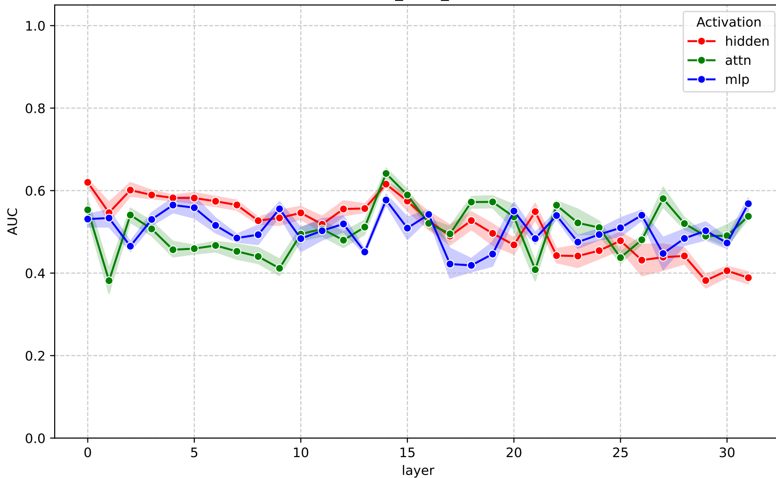
AUC across layers - gemma-3-4b-it (cross_cquad_svm)
