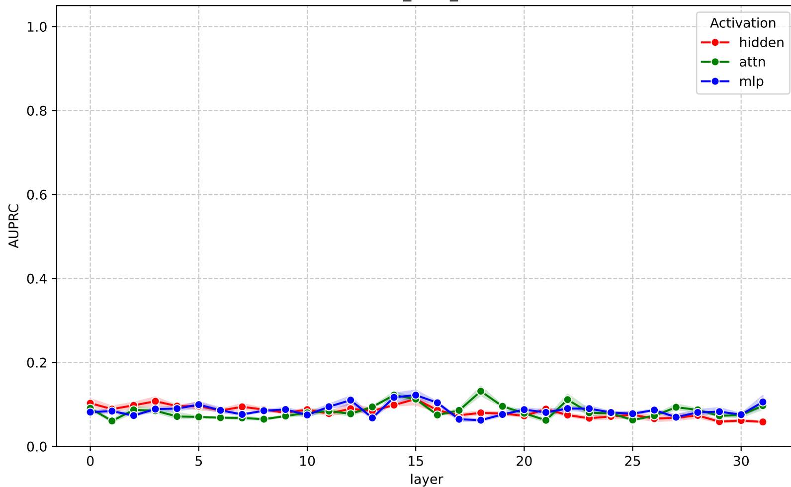
AUPRC across layers - gemma-3-4b-it (cross_cuad_svm)
