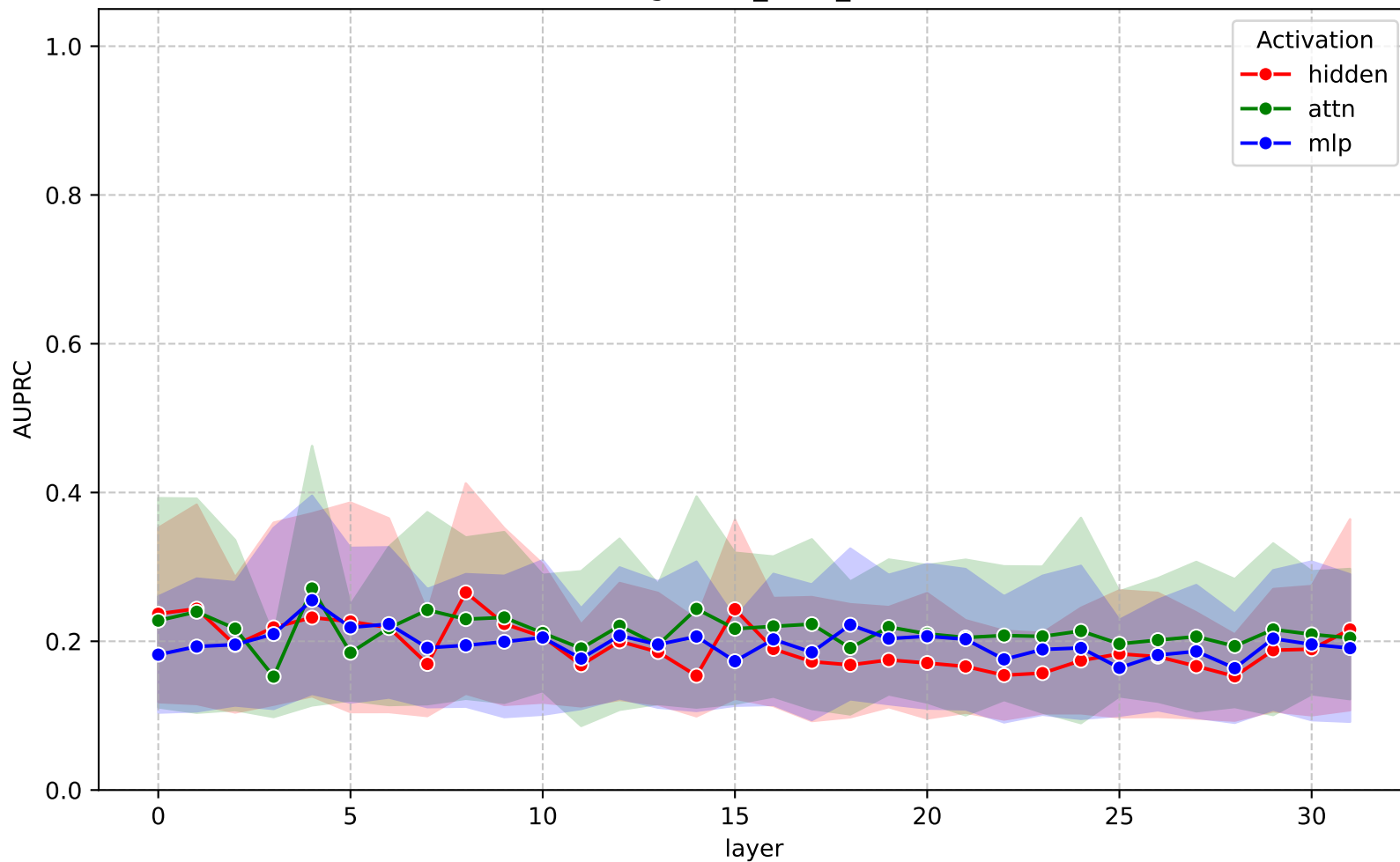
AUPRC across layers - gemma-3-4b-it (ragbench_cquad_ffn)
