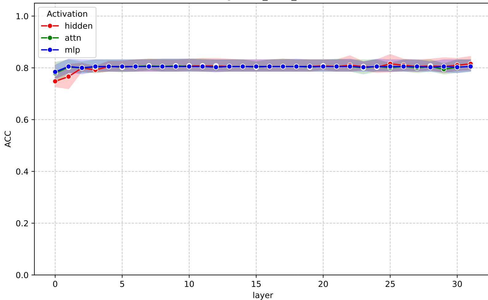
ACC across layers - gemma-3-4b-it (ragbench_cquad_ffn)
