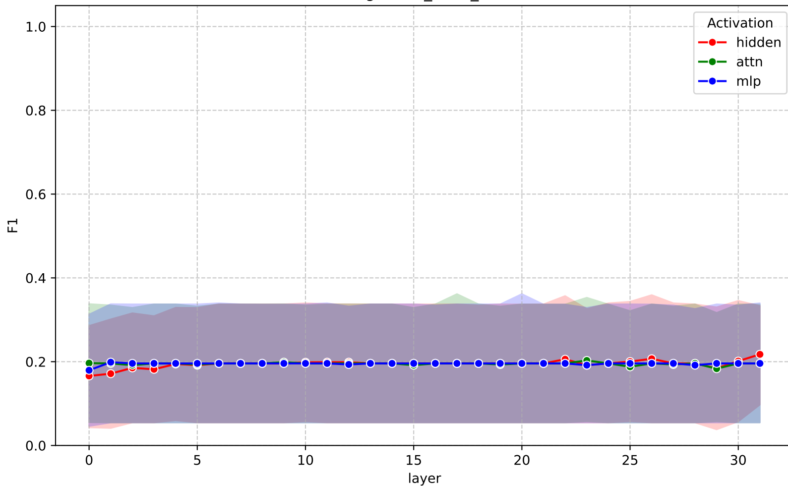
F1 across layers - gemma-3-4b-it (ragbench_cquad_ffn)
