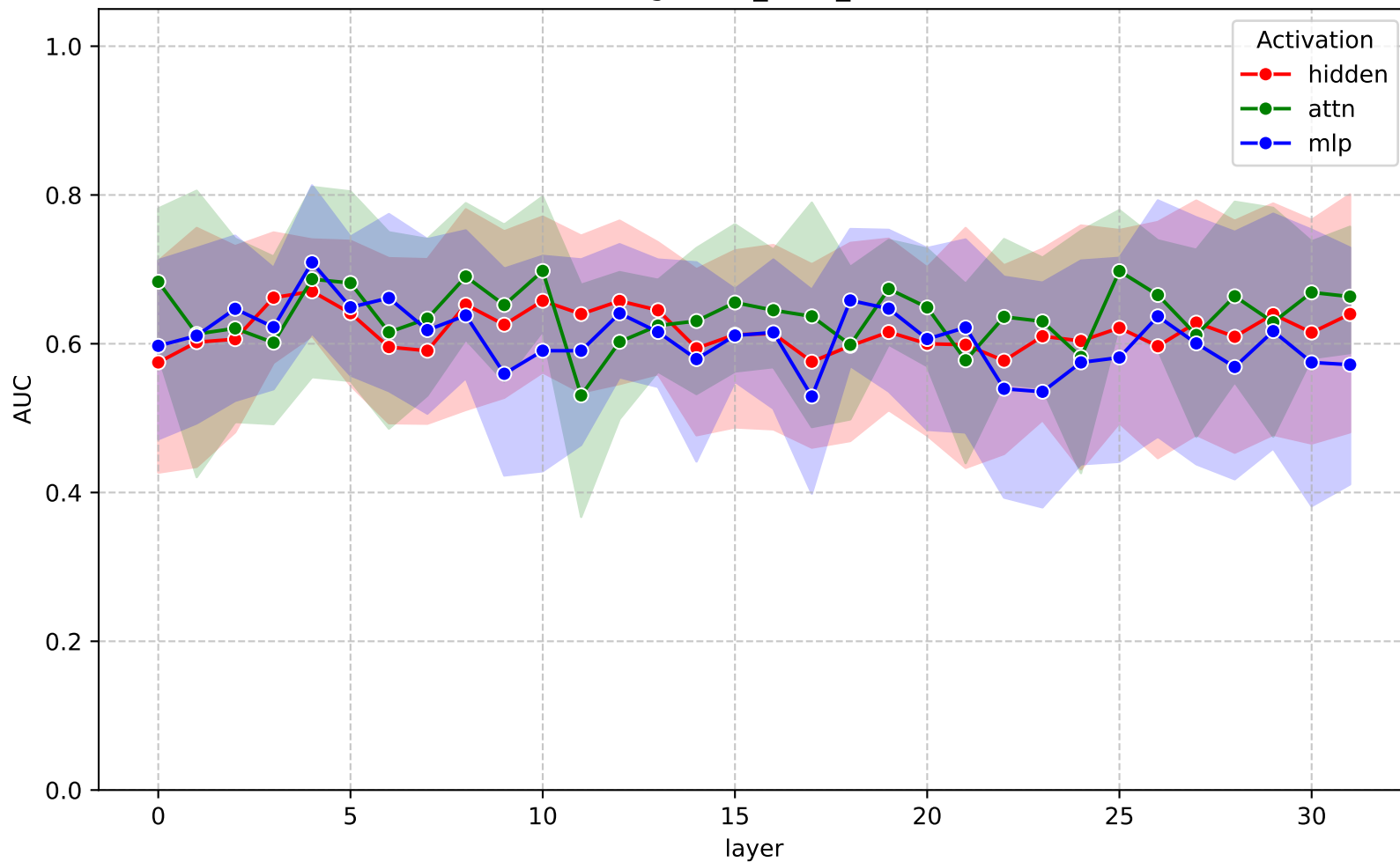
AUC across layers - gemma-3-4b-it (ragbench_cquad_ffn)
