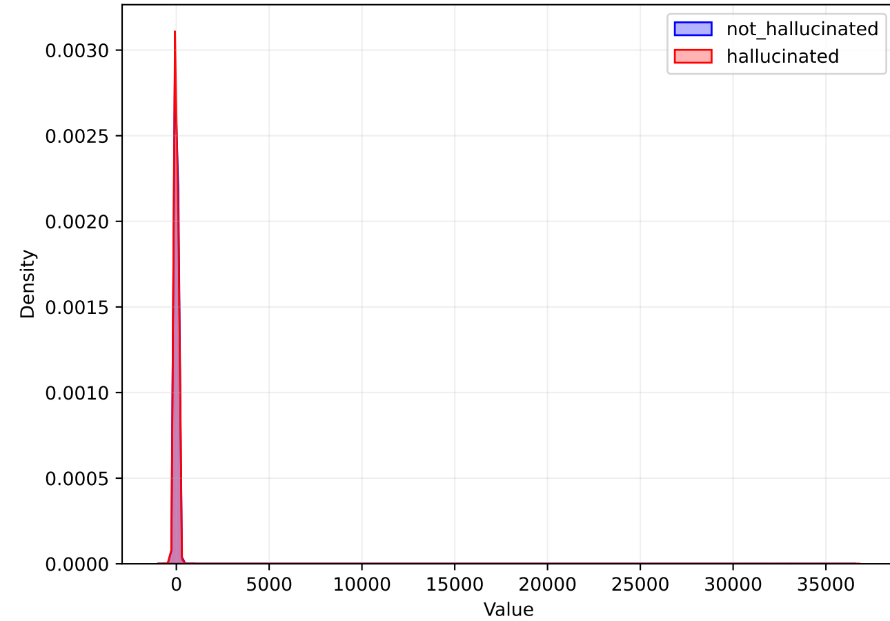
HIDDEN Distribution
