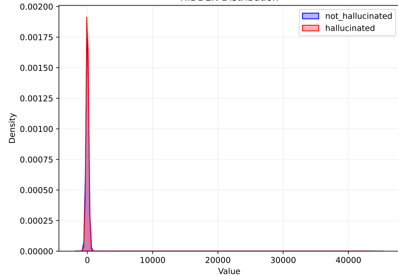
HIDDEN Distribution
