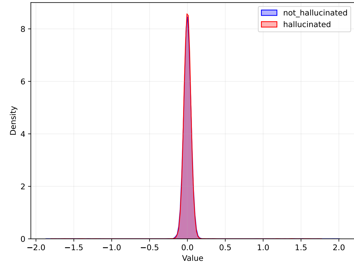
MLP Distribution
