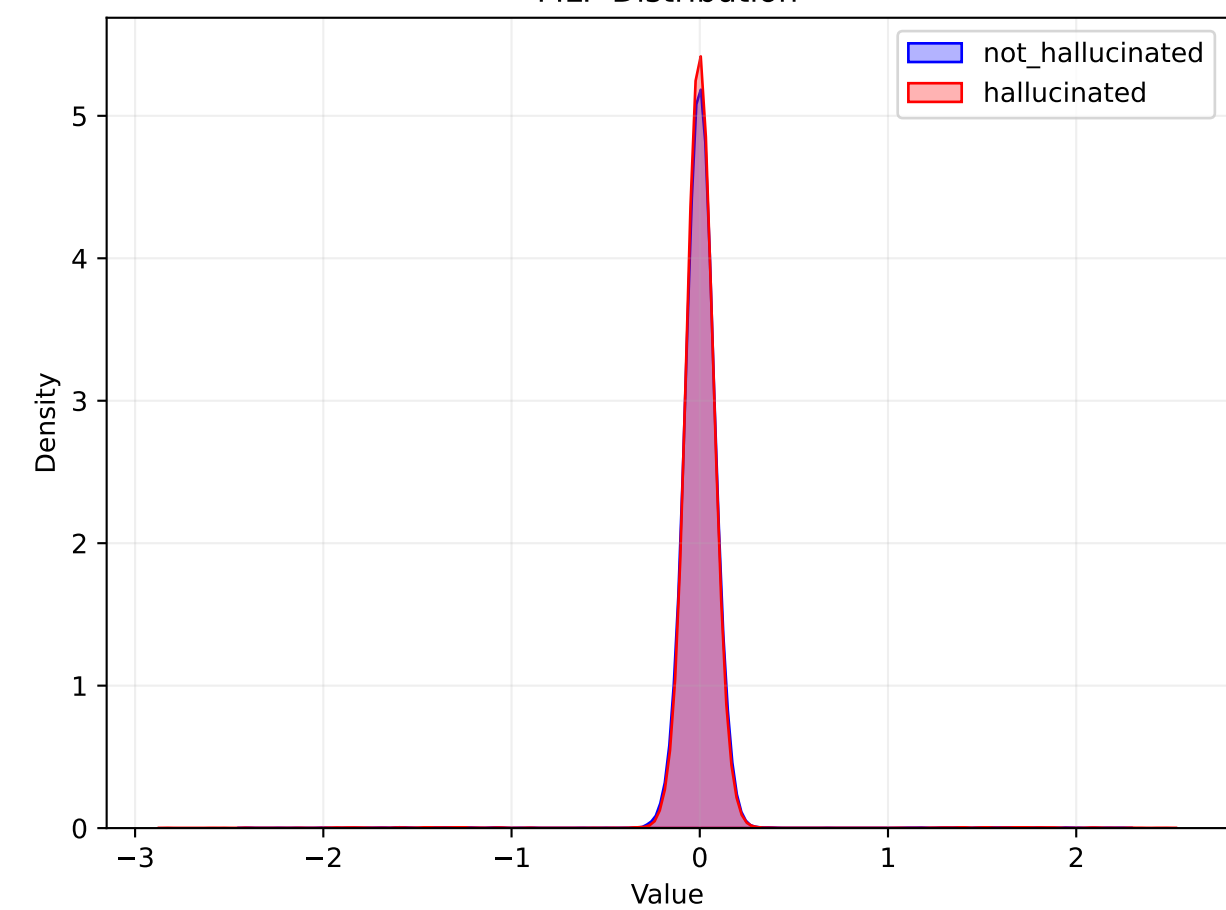
MLP Distribution
