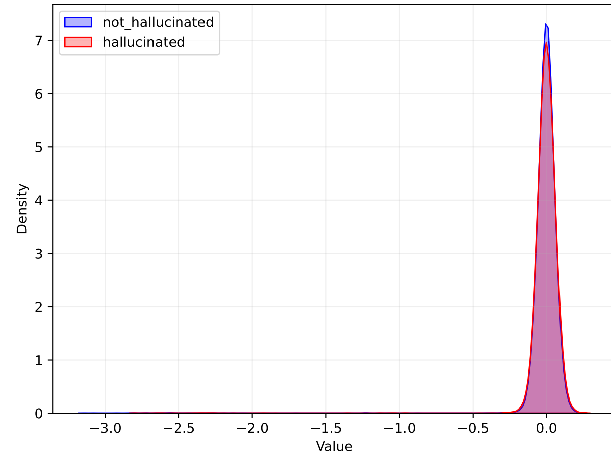
MLP Distribution
