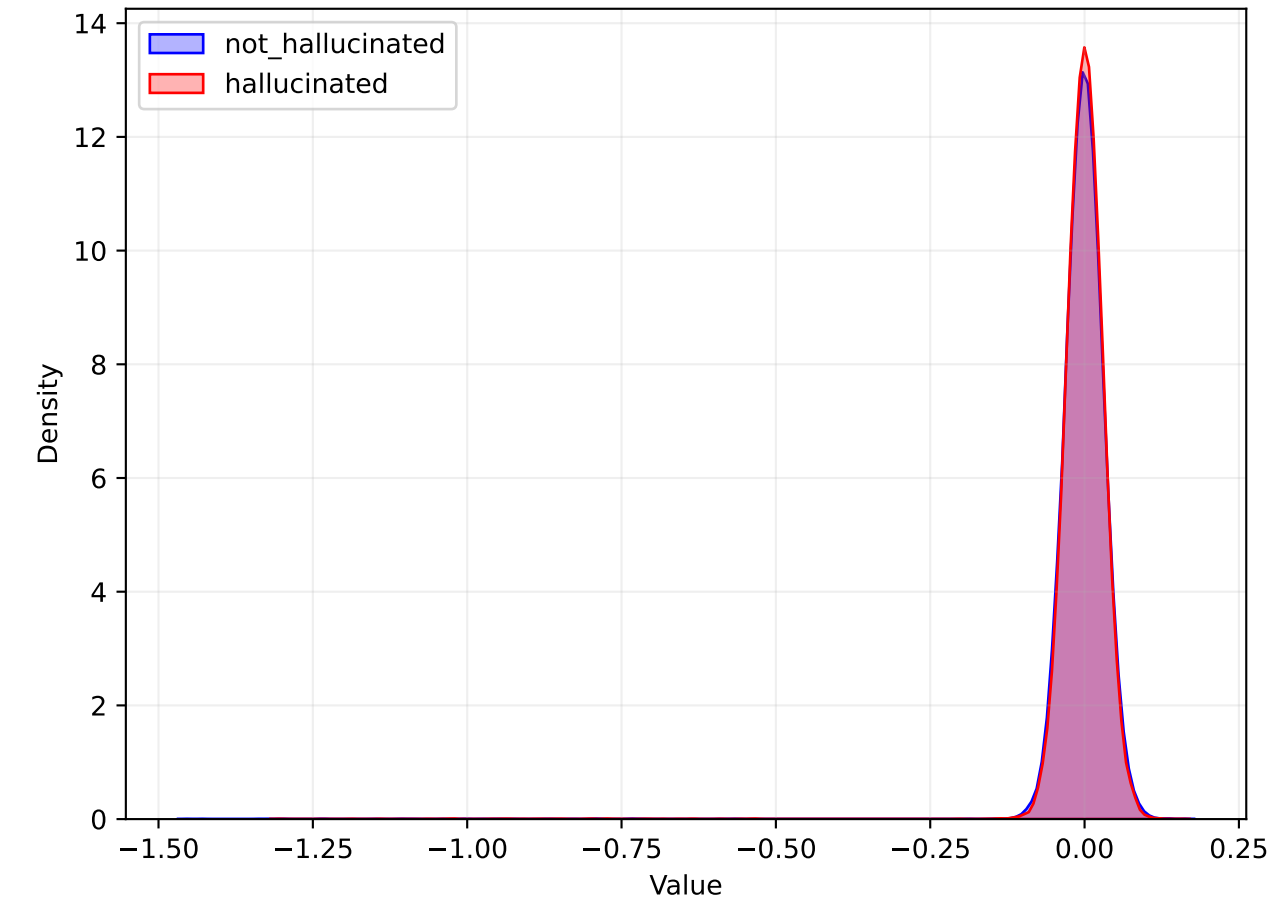
MLP Distribution
