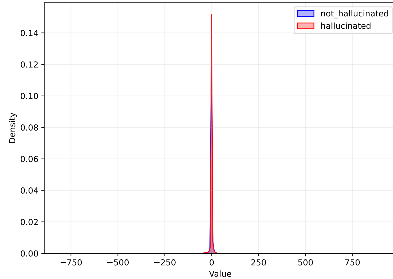
HIDDEN Distribution
