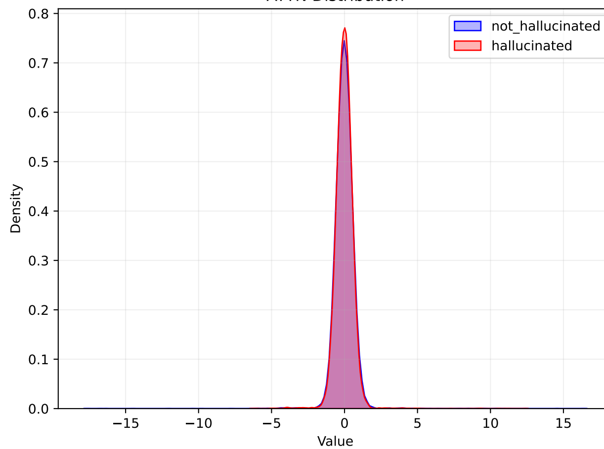
ATTN Distribution
