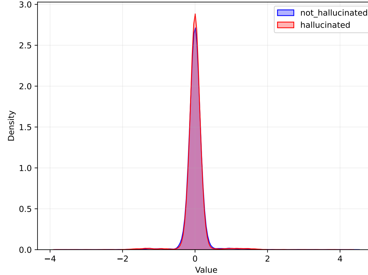
ATTN Distribution
