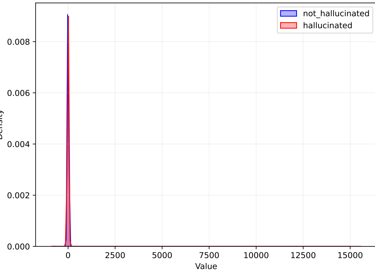
HIDDEN Distribution
