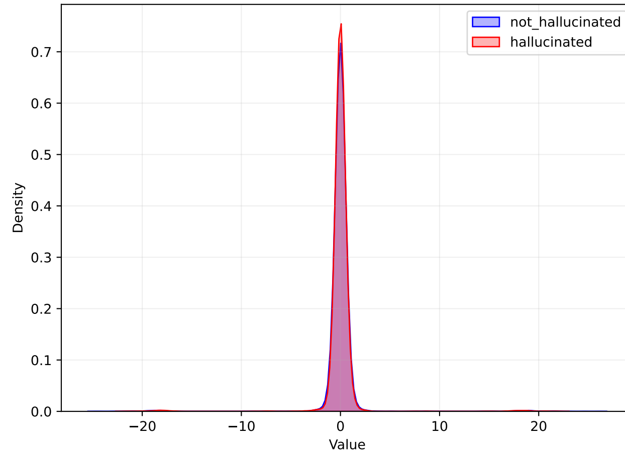
ATTN Distribution
