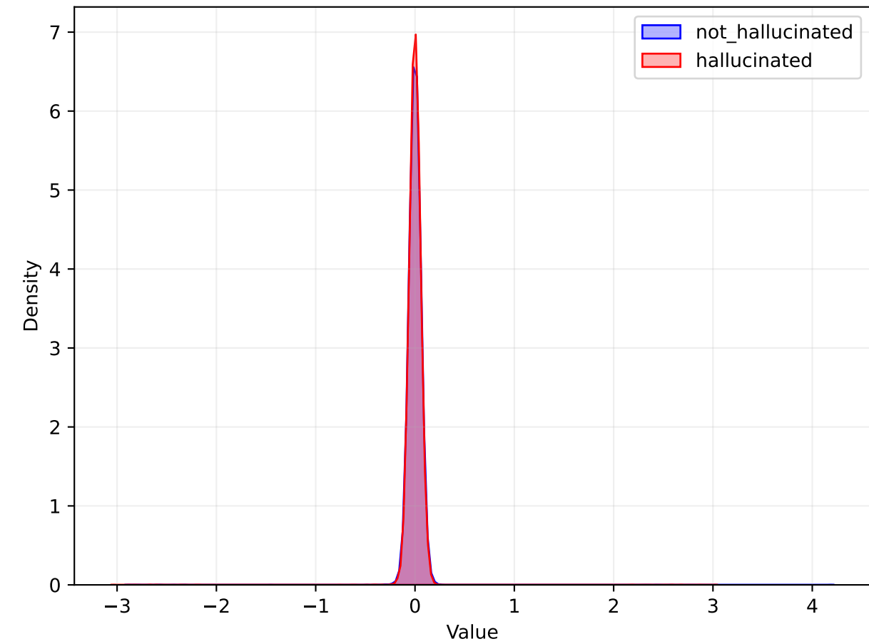
MLP Distribution
