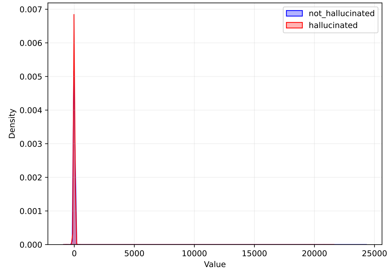
HIDDEN Distribution
