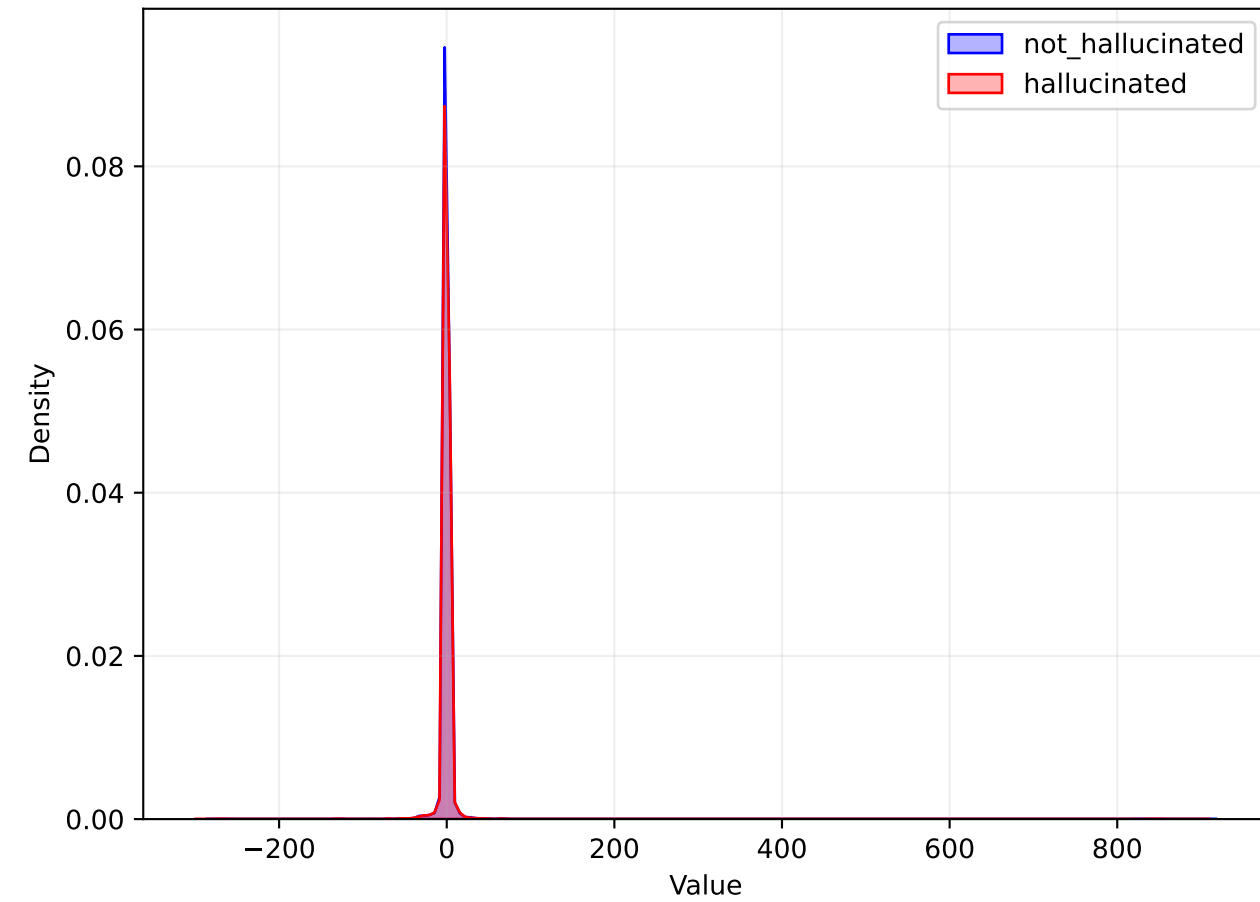
HIDDEN Distribution
