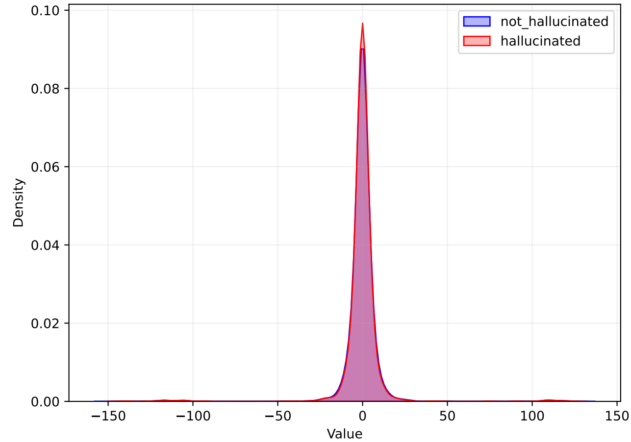
ATTN Distribution
