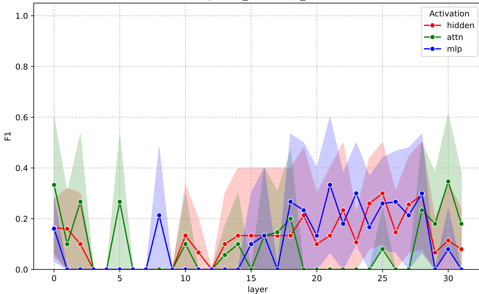
F1 across layers - gemma-3-4b-it (ragbench_delucionqa_ffn)
