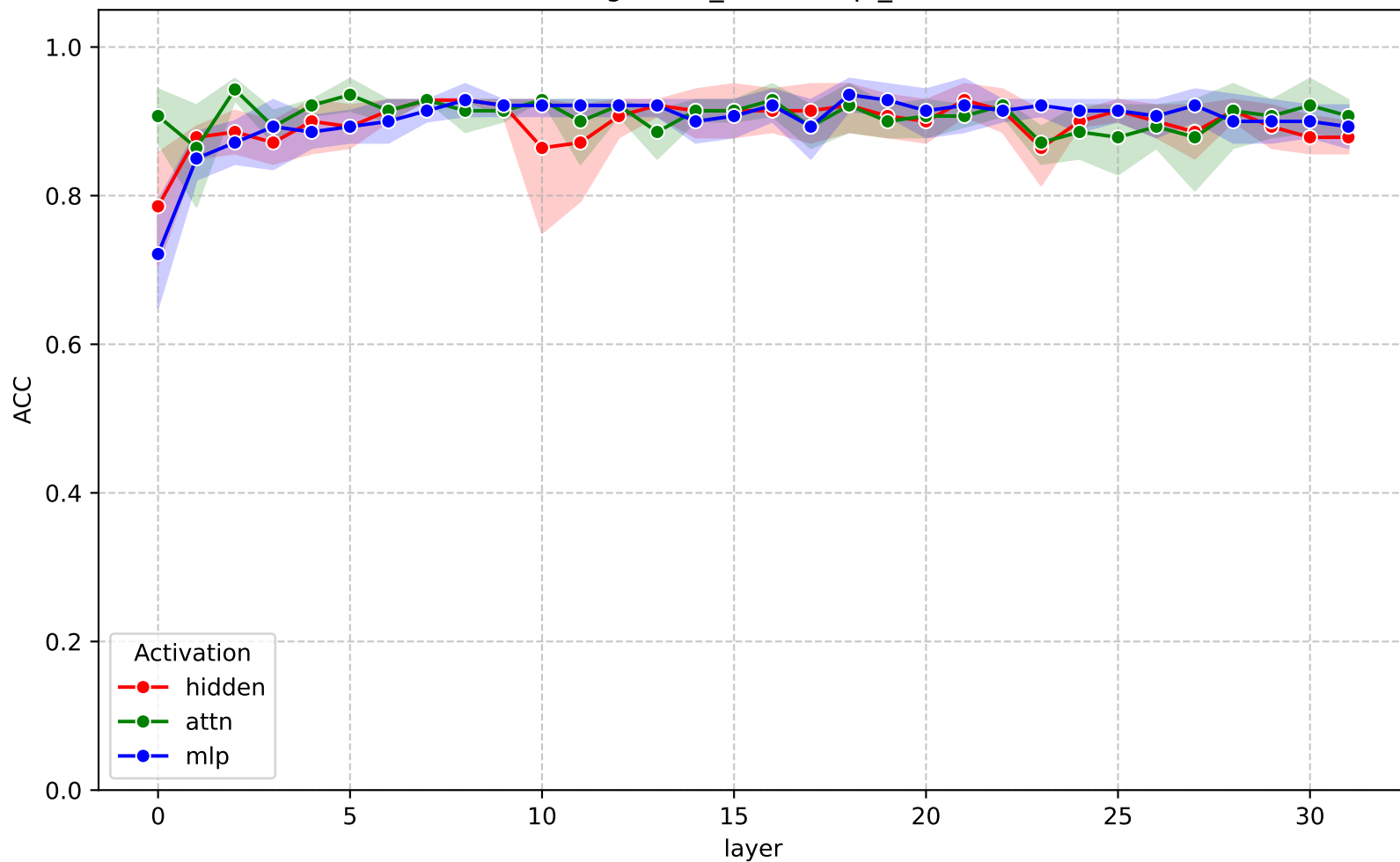
ACC across layers - gemma-3-4b-it (ragbench_delucionqa_ffn)
