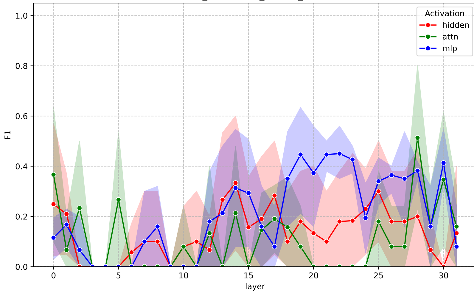
F1 across layers - gemma-3-4b-it (ragbench_delucionqa_logistic_regression)
