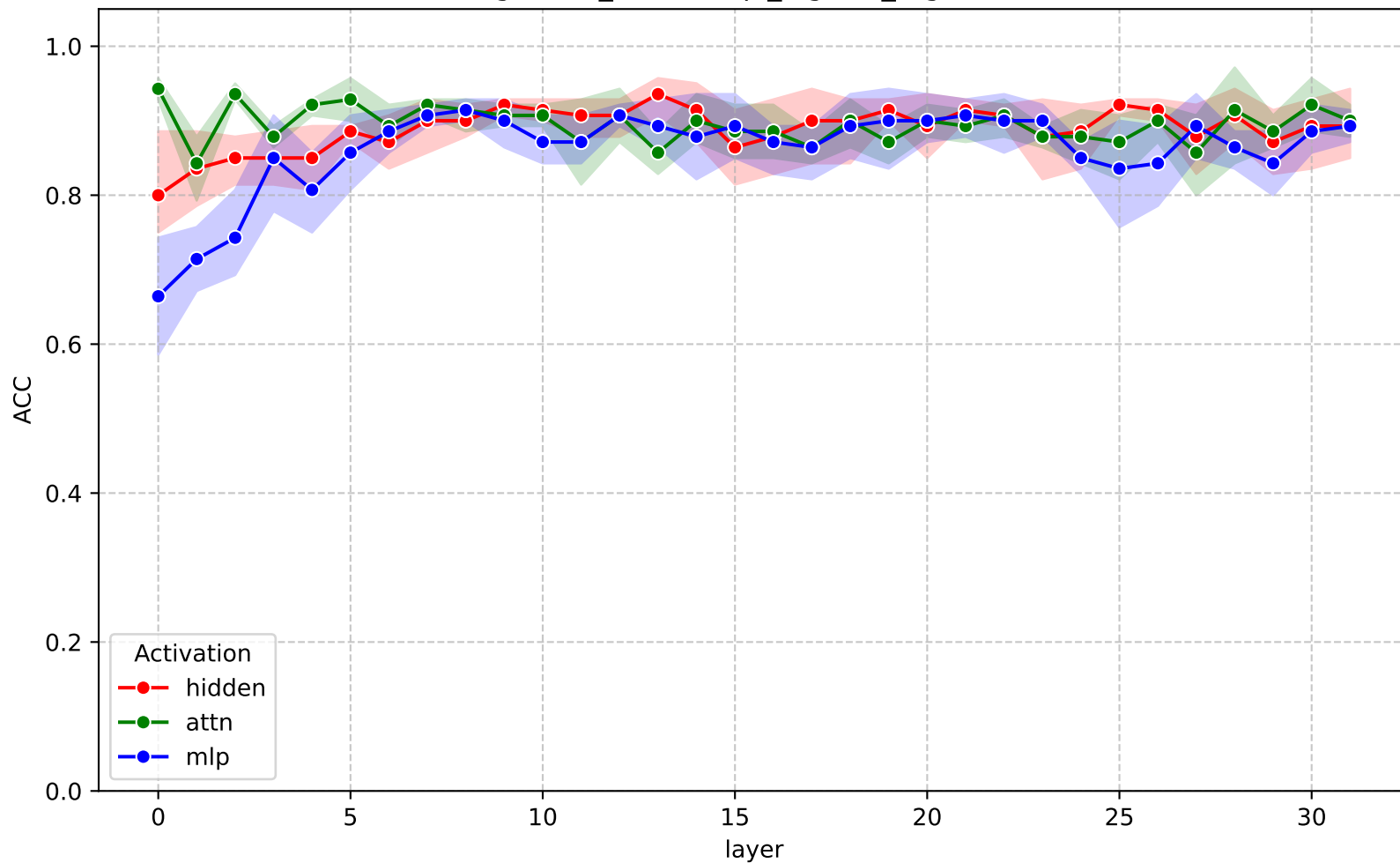
ACC across layers - gemma-3-4b-it (ragbench_delucionqa_logistic_regression)
