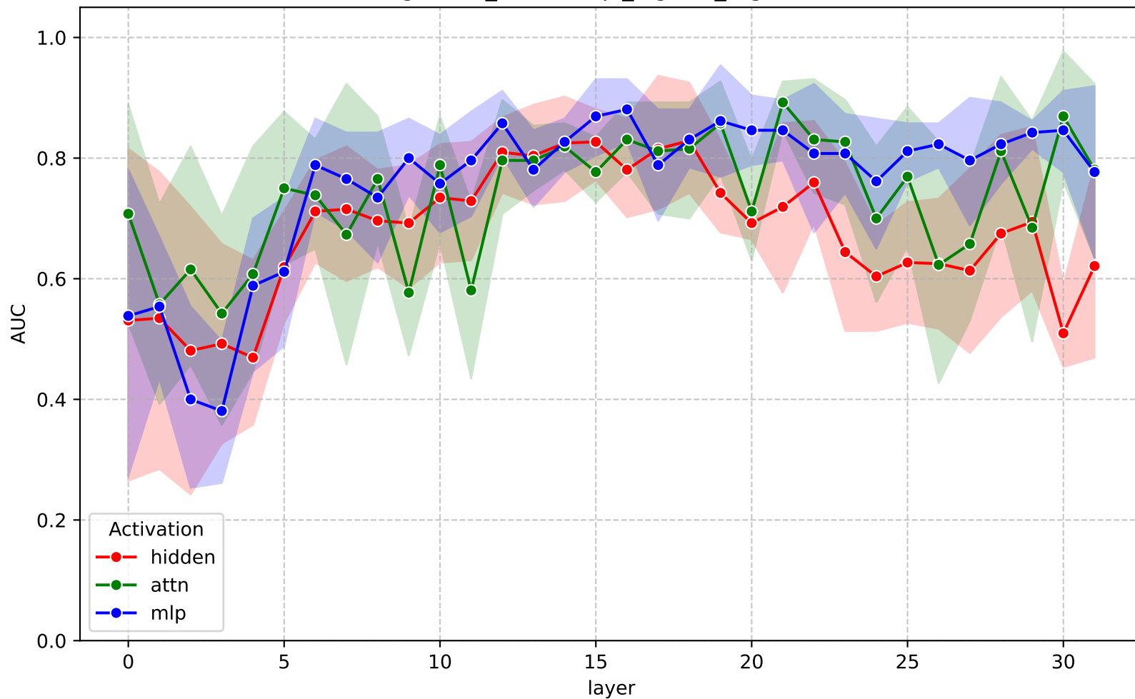
AUC across layers - gemma-3-4b-it (ragbench_delucionqa_logistic_regression)
