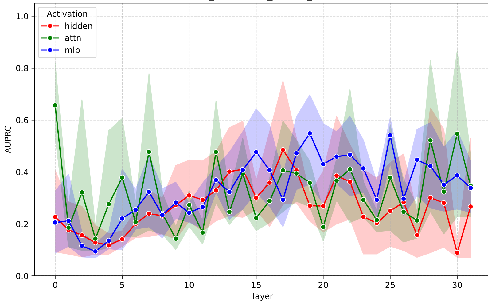
AUPRC across layers - gemma-3-4b-it (ragbench_delucionqa_logistic_regression)
