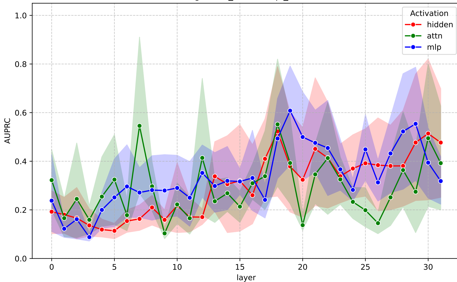
AUPRC across layers - gemma-3-4b-it (ragbench_delucionqa_svm)
