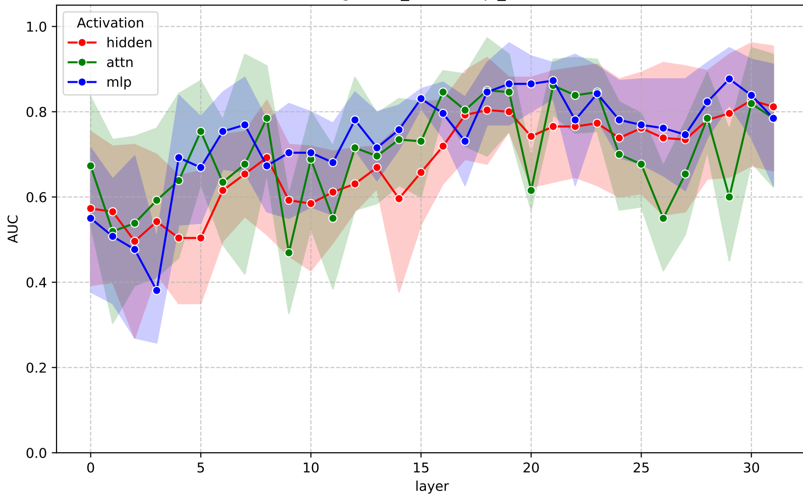
AUC across layers - gemma-3-4b-it (ragbench_delucionqa_svm)
