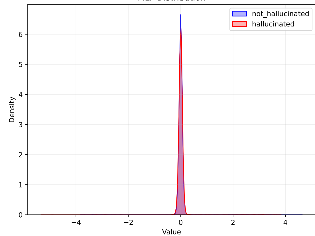
MLP Distribution
