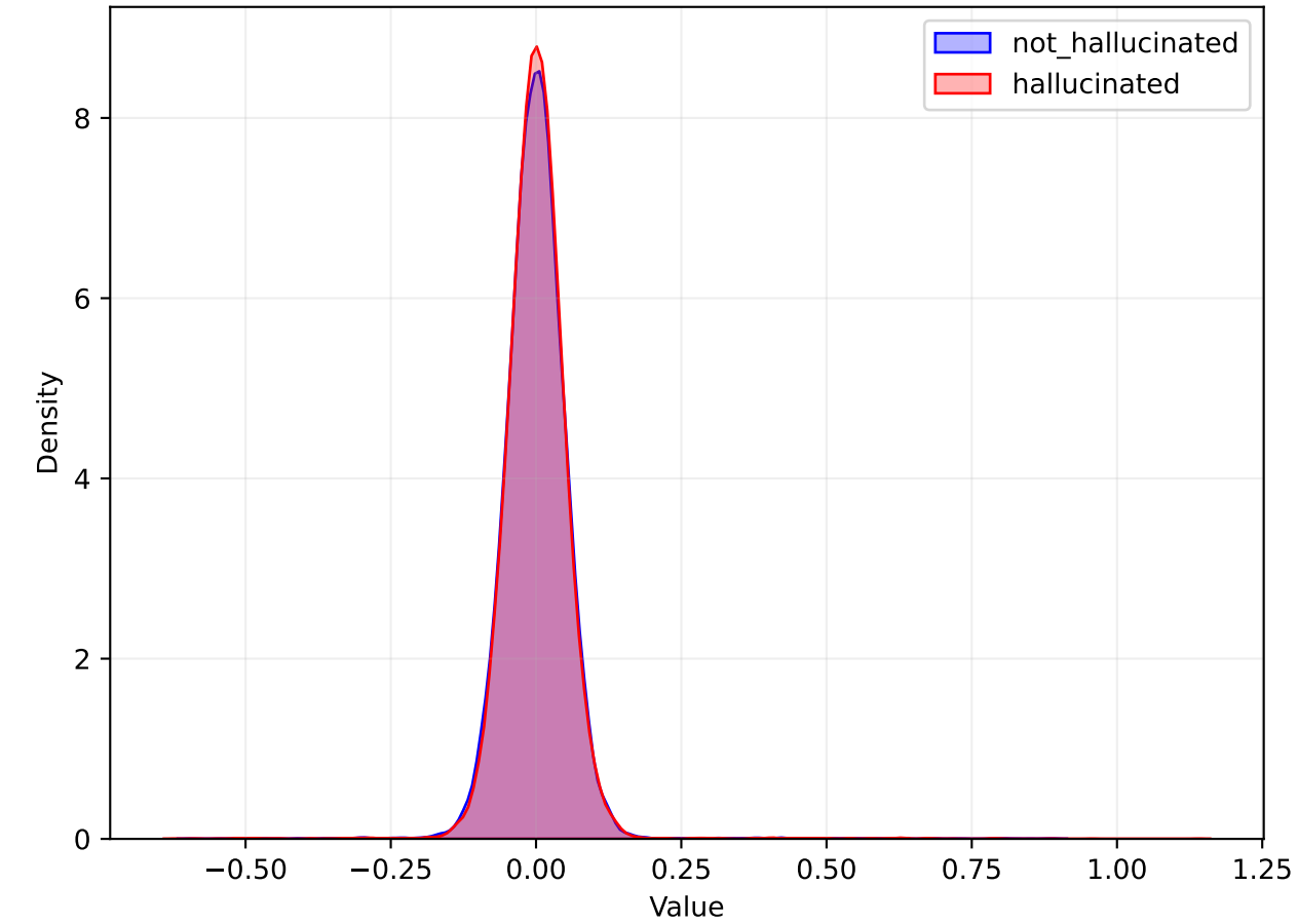
MLP Distribution
