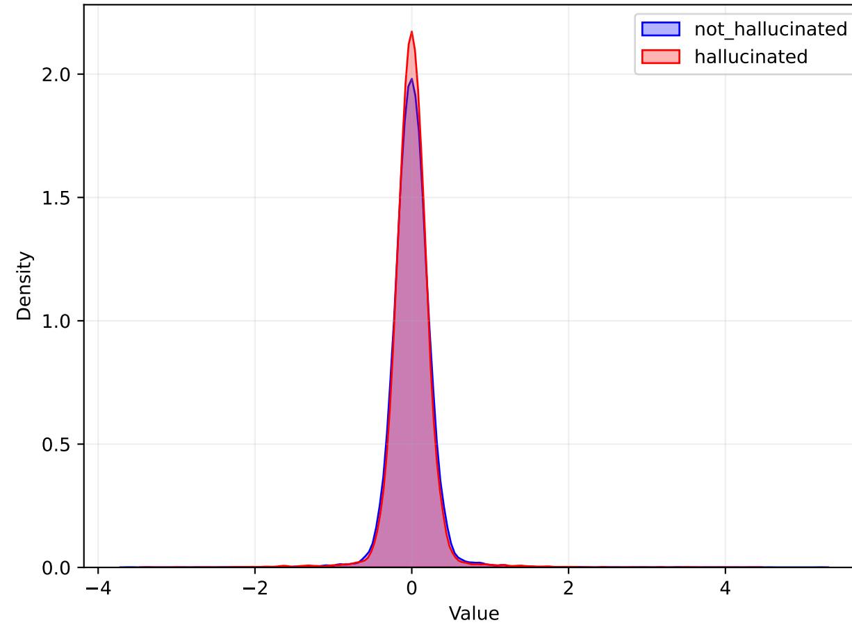
ATTN Distribution
