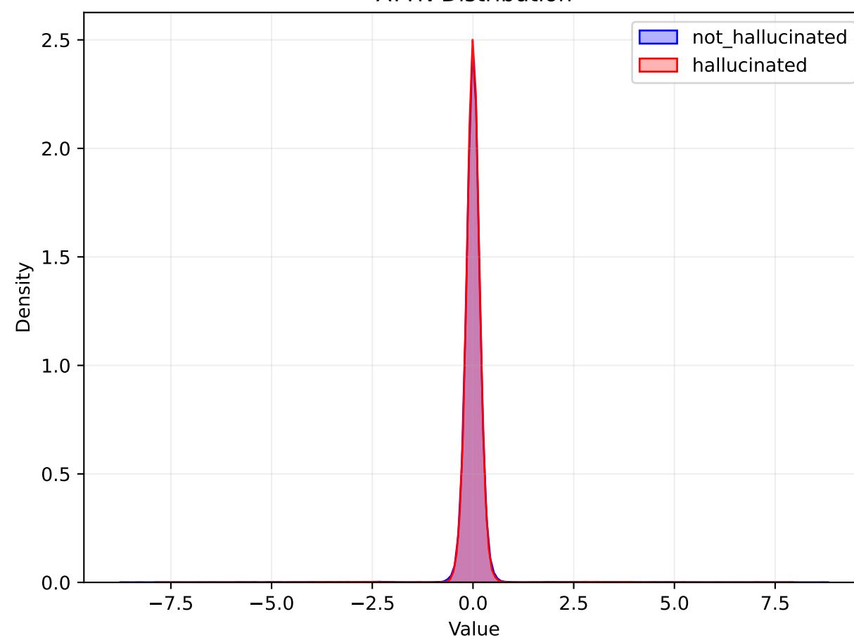
ATTN Distribution
