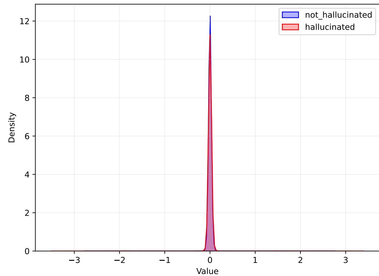
MLP Distribution
