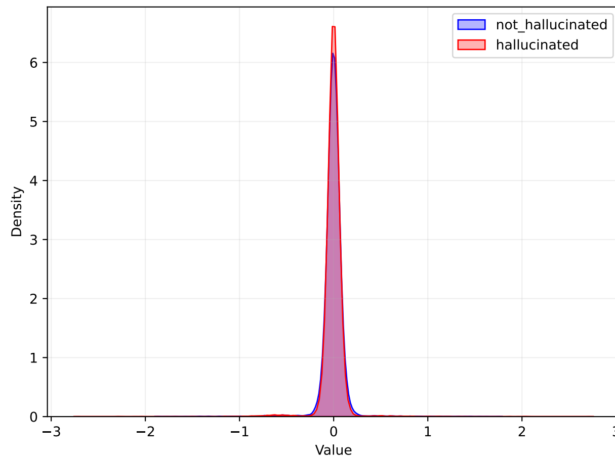
ATTN Distribution
