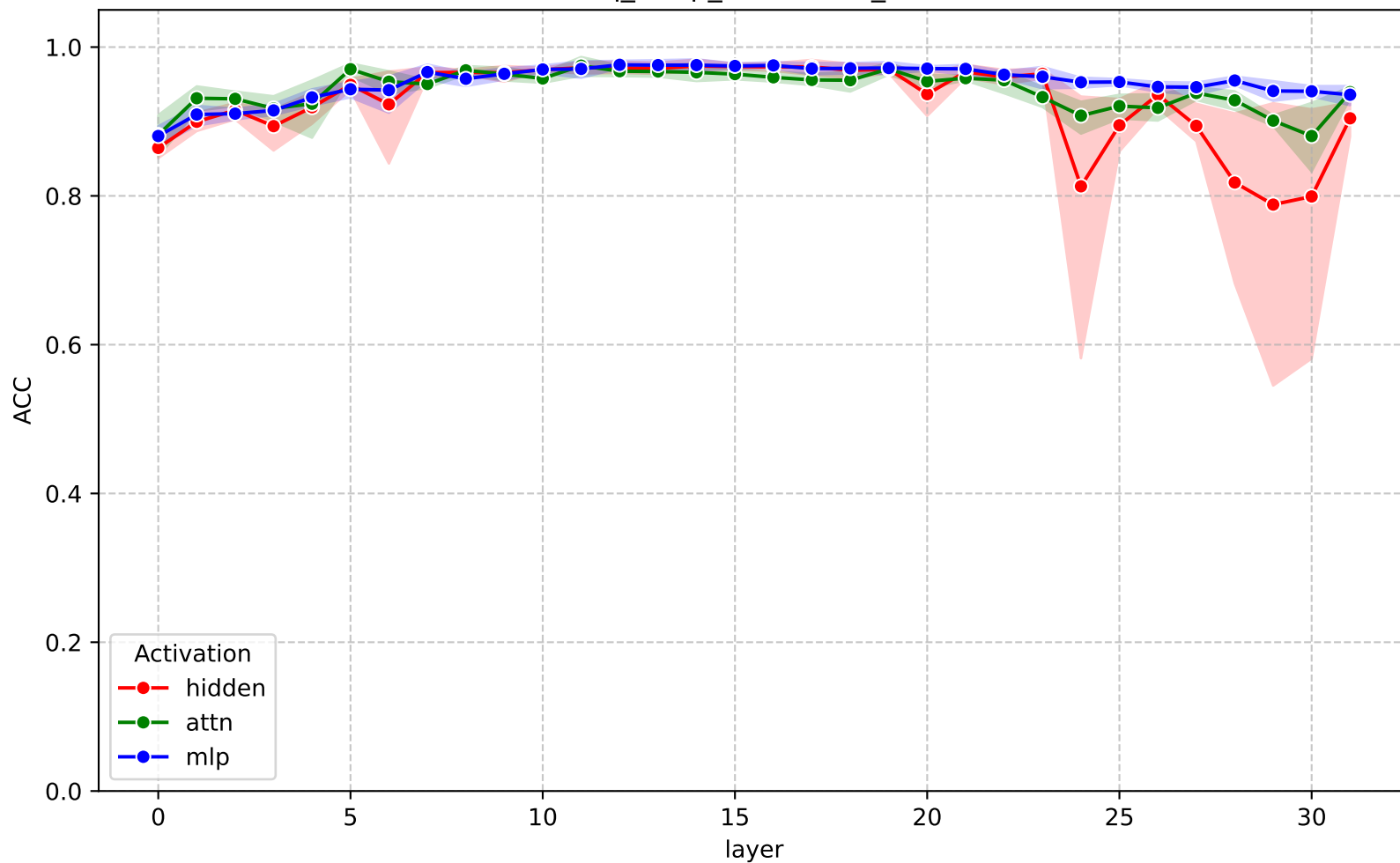
ACC across layers - gemma-3-4b-it (nq_swap_contextual_ffn)
