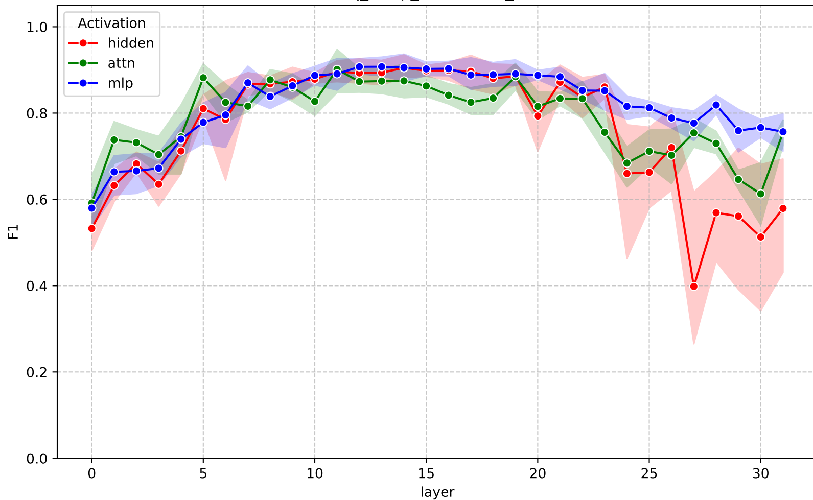
F1 across layers - gemma-3-4b-it (nq_swap_contextual_ffn)
