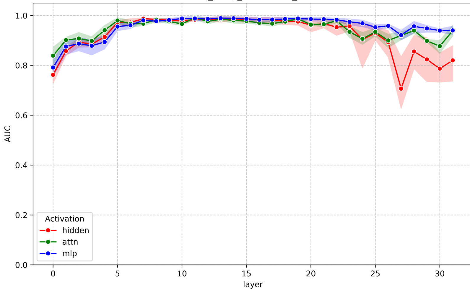
AUC across layers - gemma-3-4b-it (nq_swap_contextual_ffn)
