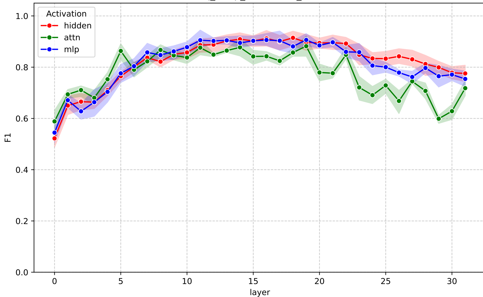
F1 across layers - gemma-3-4b-it (nq_swap_contextual_svm)
