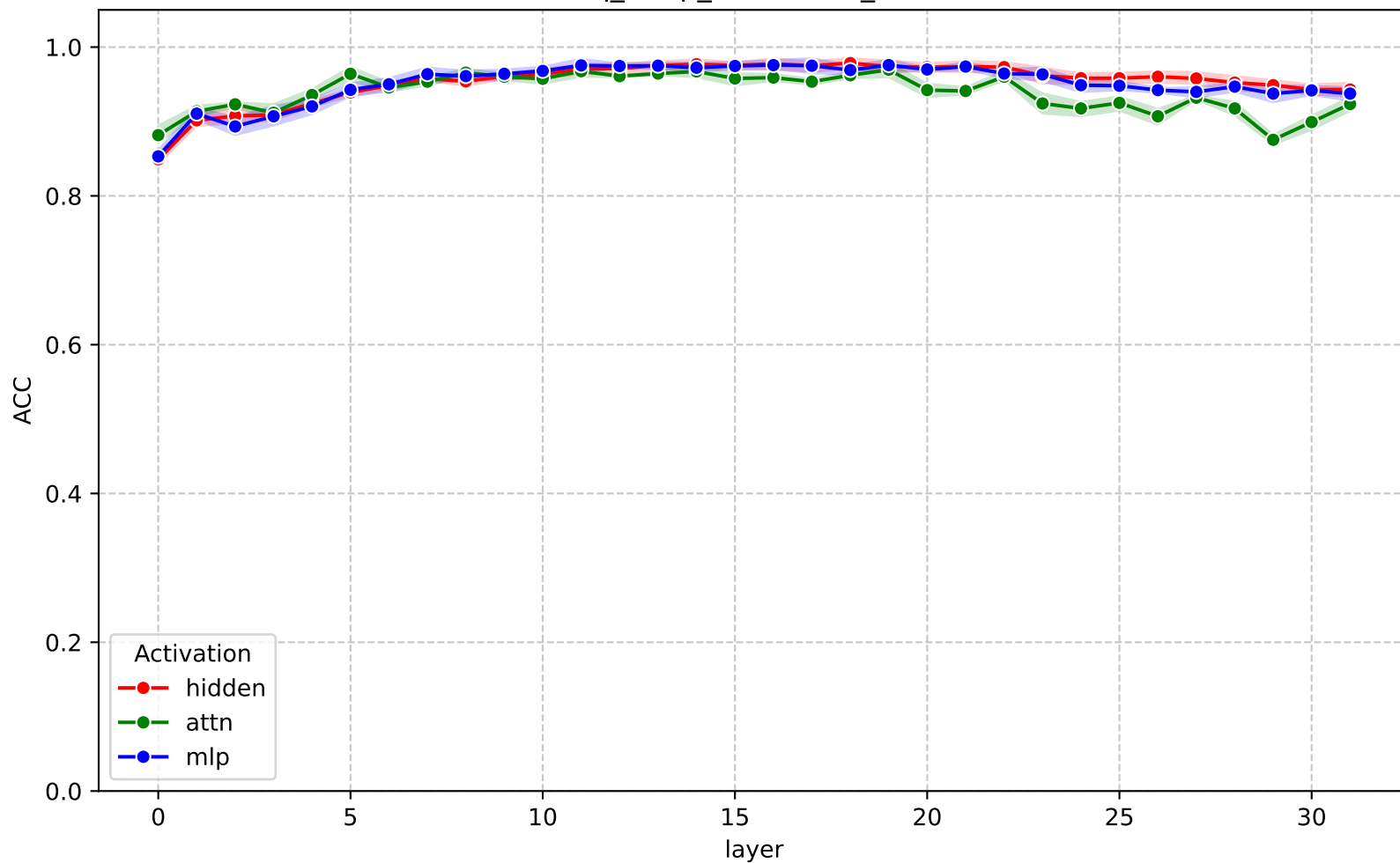
ACC across layers - gemma-3-4b-it (nq_swap_contextual_svm)
