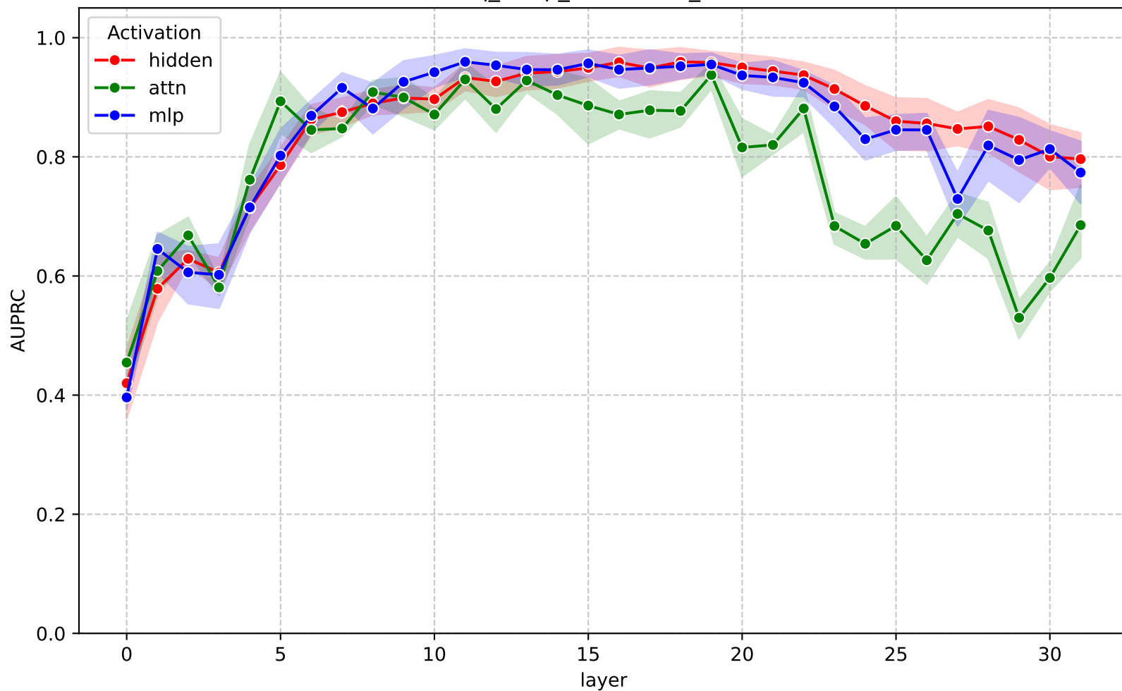
AUPRC across layers - gemma-3-4b-it (nq_swap_contextual_svm)
