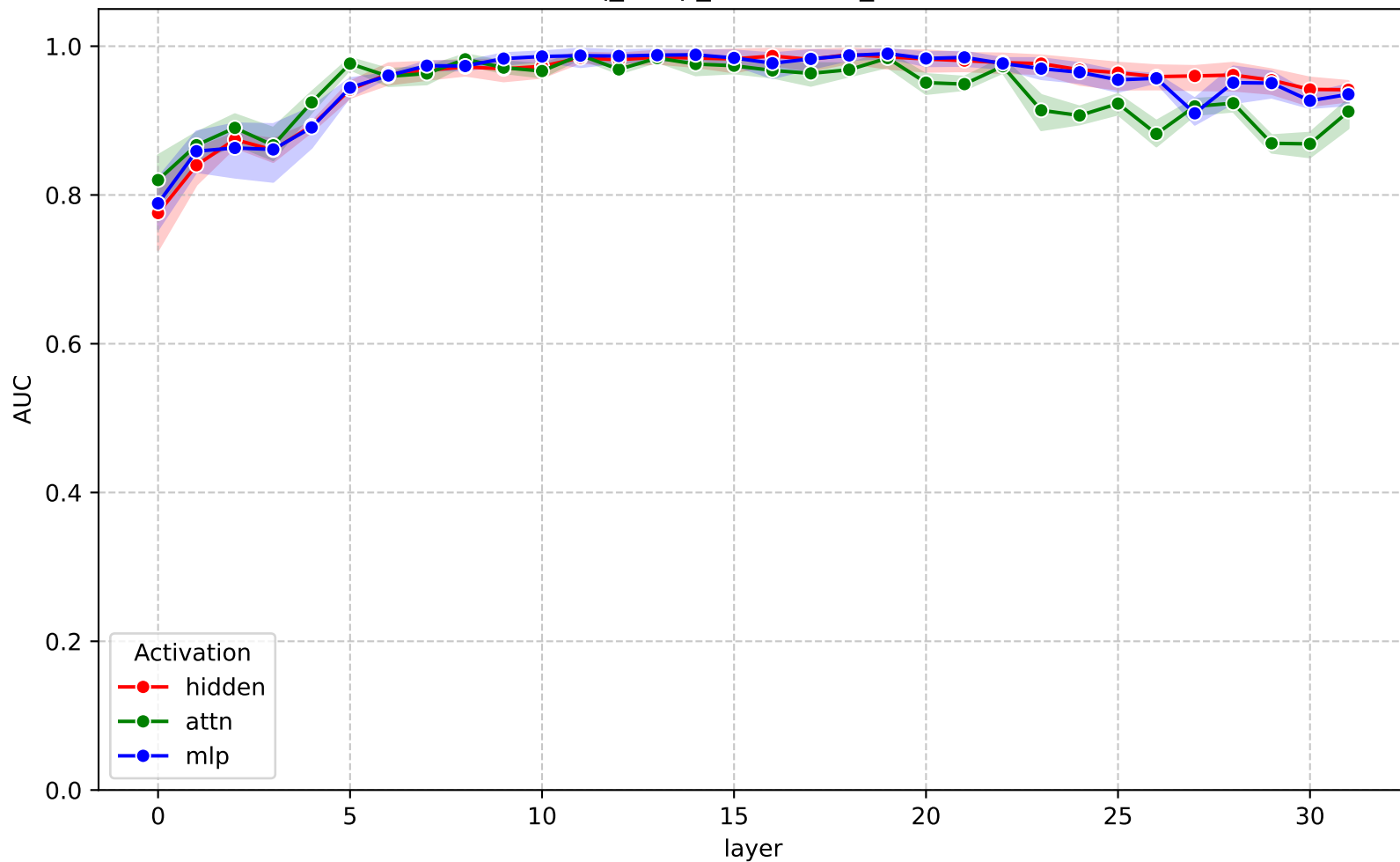
AUC across layers - gemma-3-4b-it (nq_swap_contextual_svm)
