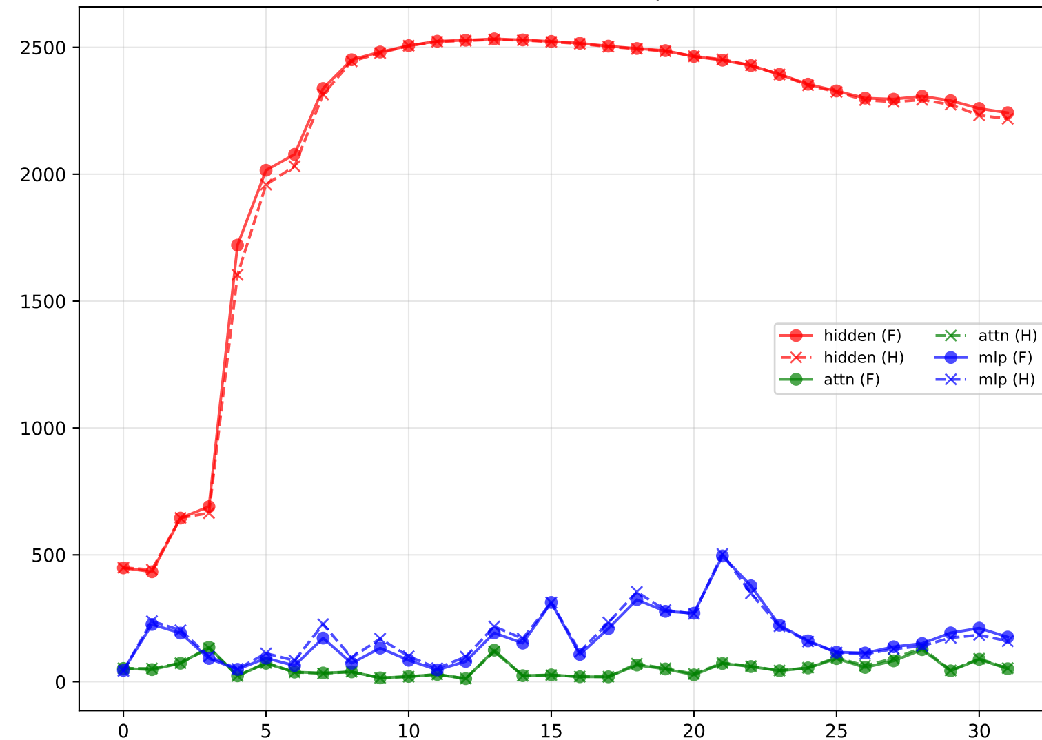
Kurtosis - Overlaid Comparison
