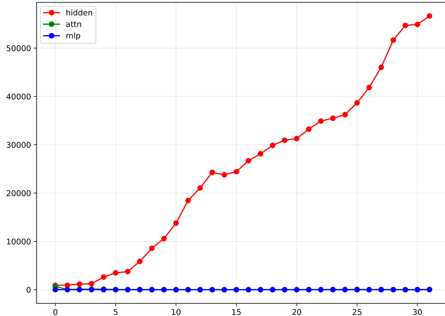
L2 - Faithful Only
