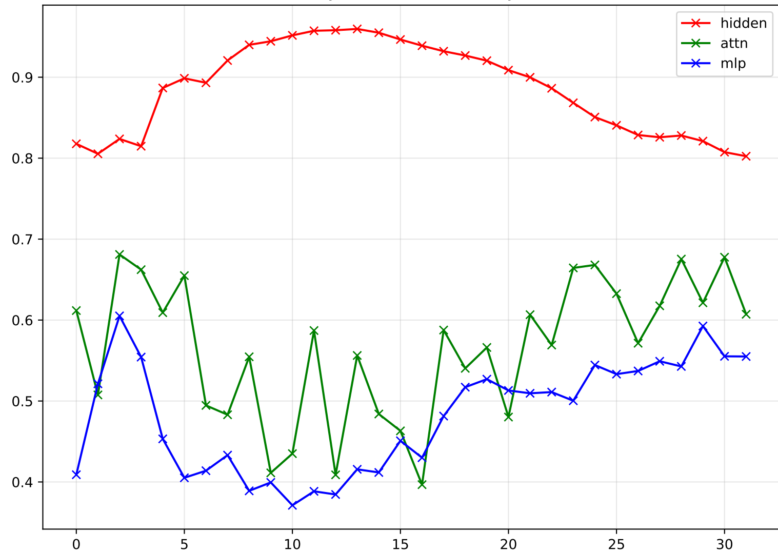
Hoyer - Hallucinated Only
