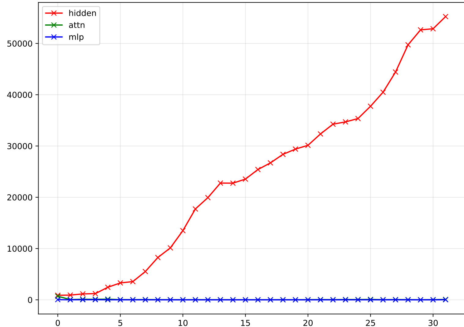
L2 - Hallucinated Only
