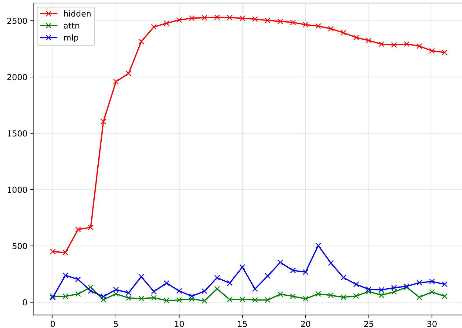
Kurtosis - Hallucinated Only
