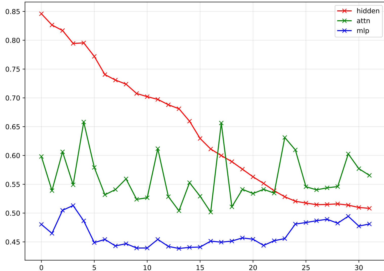
Gini - Hallucinated Only
