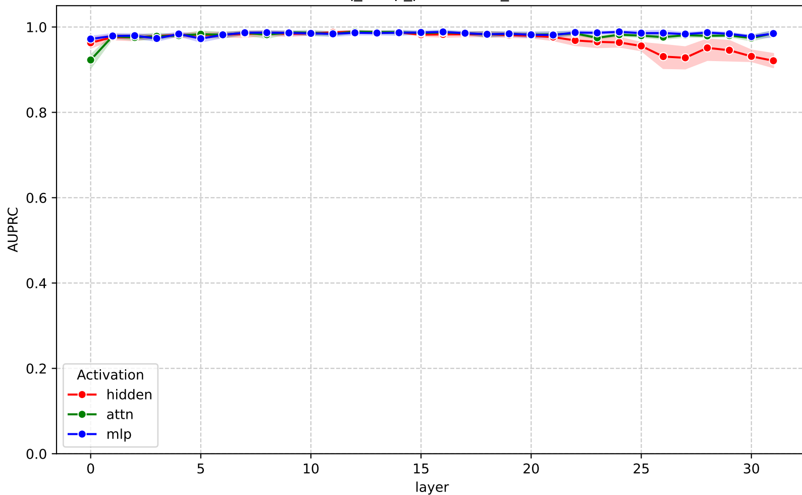
AUPRC across layers - gemma-3-4b-it (nq_swap_parametric_ffn)
