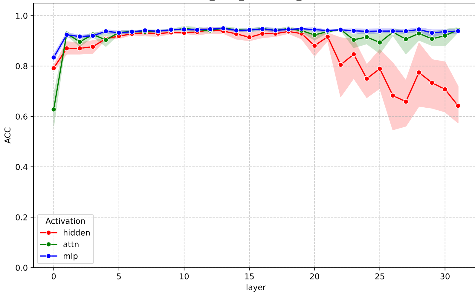
ACC across layers - gemma-3-4b-it (nq_swap_parametric_ffn)
