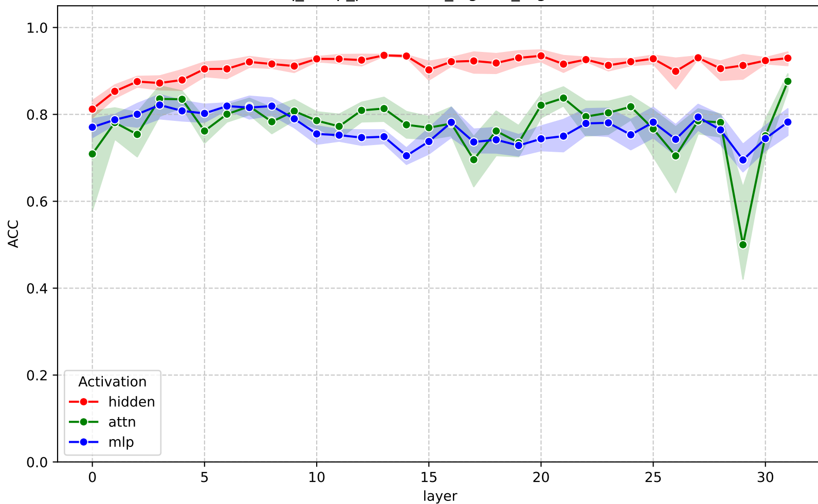
ACC across layers - gemma-3-4b-it (nq_swap_parametric_logistic_regression)
