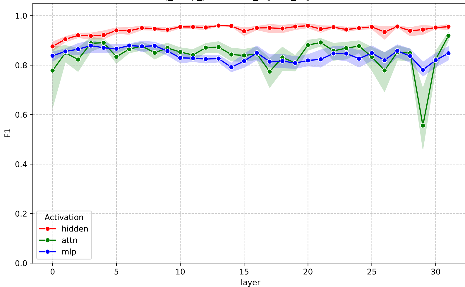
F1 across layers - gemma-3-4b-it (nq_swap_parametric_logistic_regression)
