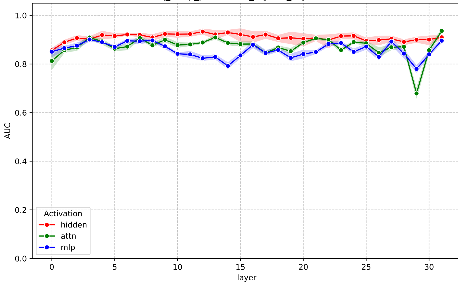
AUC across layers - gemma-3-4b-it (nq_swap_parametric_logistic_regression)
