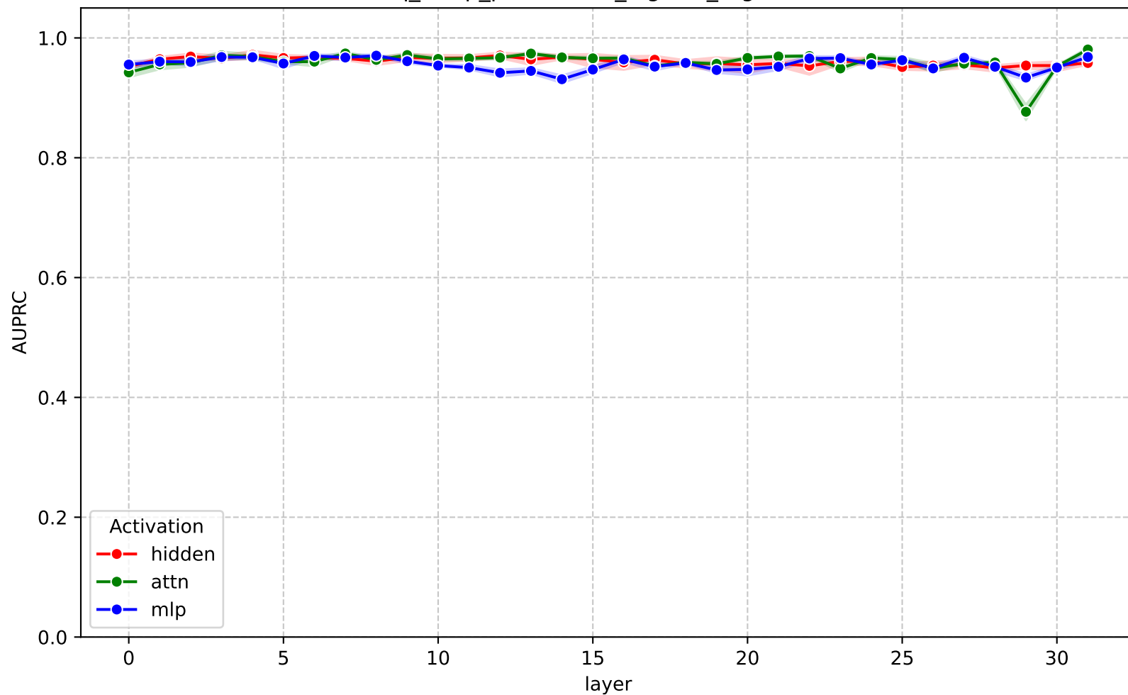
AUPRC across layers - gemma-3-4b-it (nq_swap_parametric_logistic_regression)
