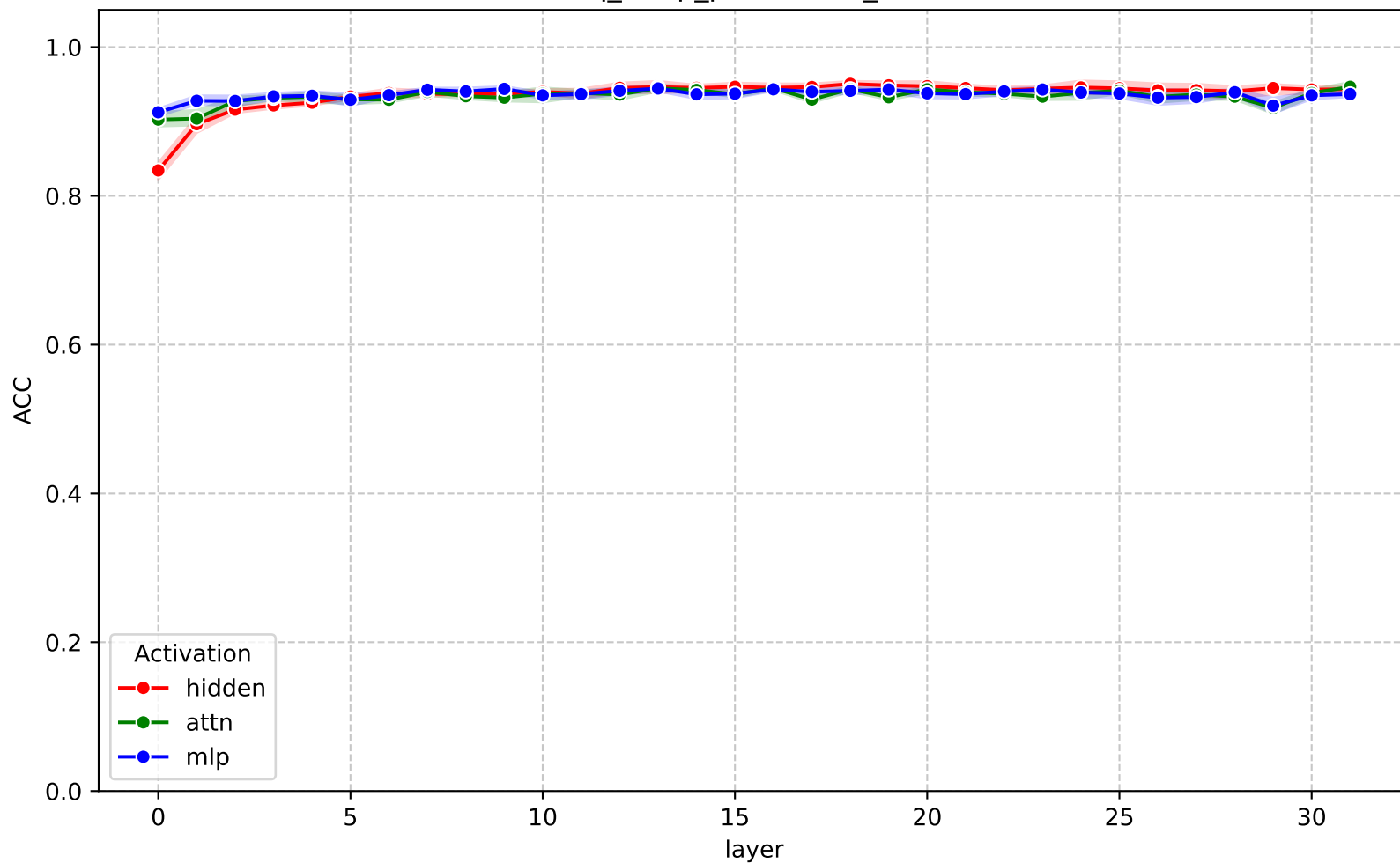
ACC across layers - gemma-3-4b-it (nq_swap_parametric_svm)
