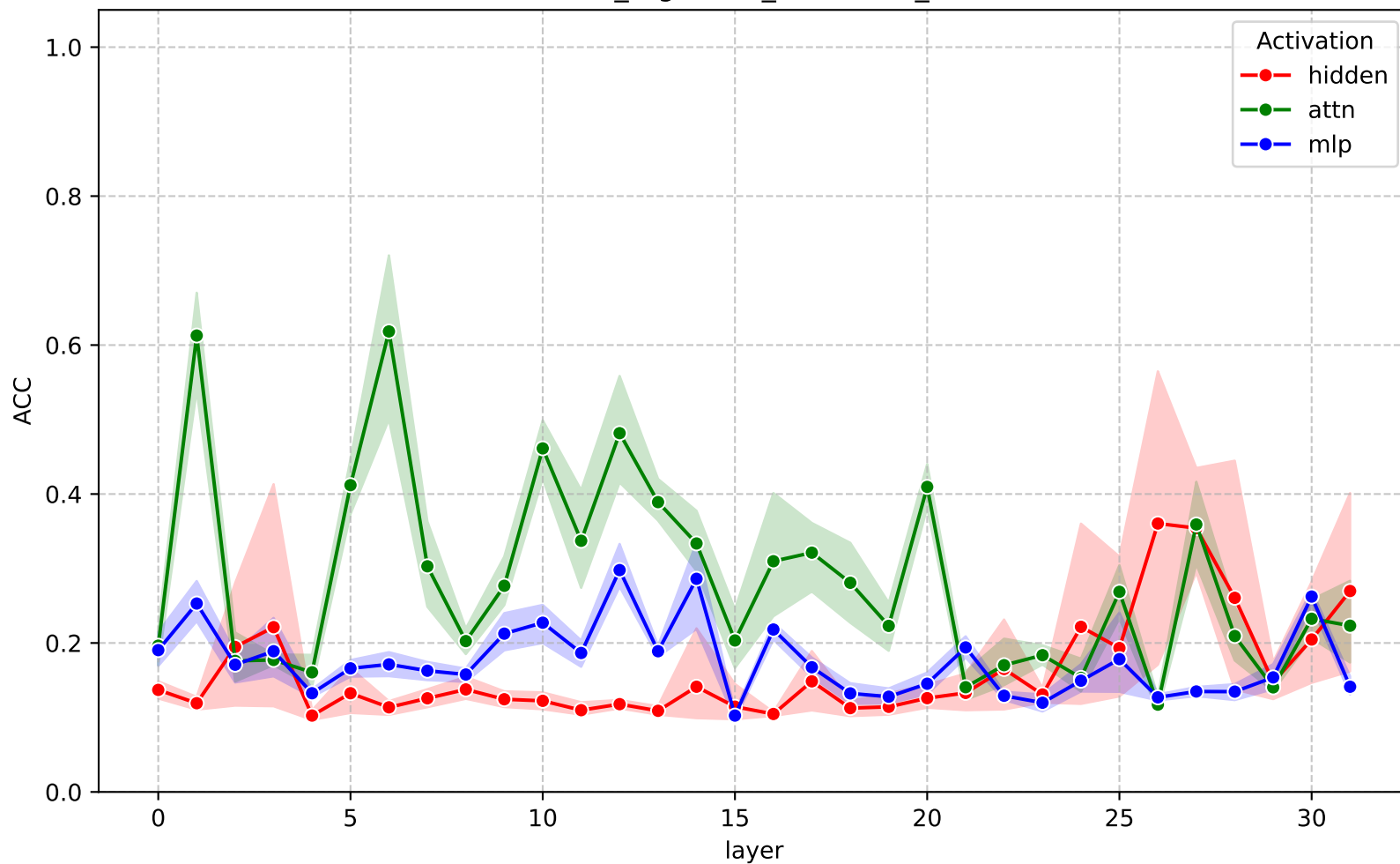
ACC across layers - gemma-3-4b-it (cross_ragbench_combined_ffn)
