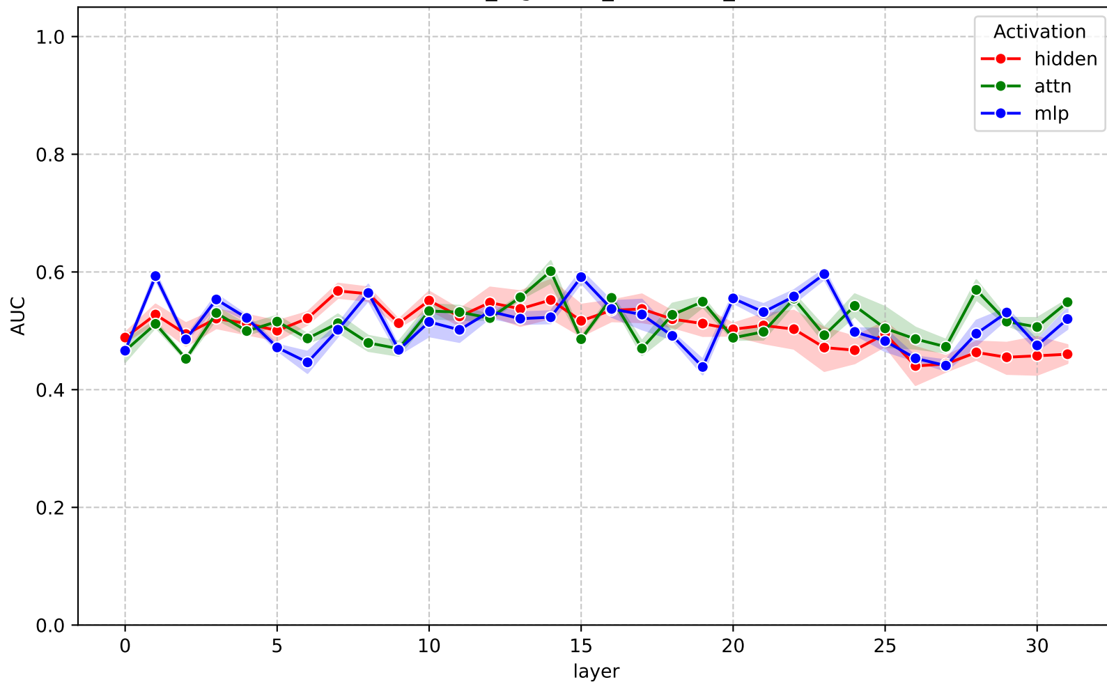
AUC across layers - gemma-3-4b-it (cross_ragbench_combined_ffn)
