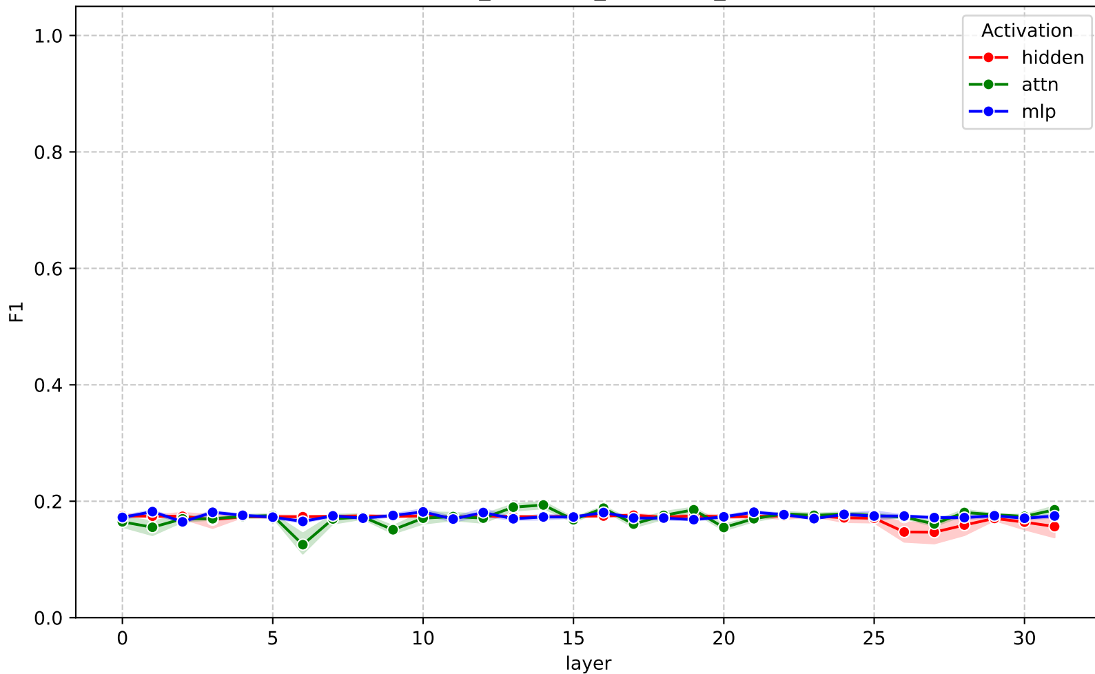
F1 across layers - gemma-3-4b-it (cross_ragbench_combined_ffn)
