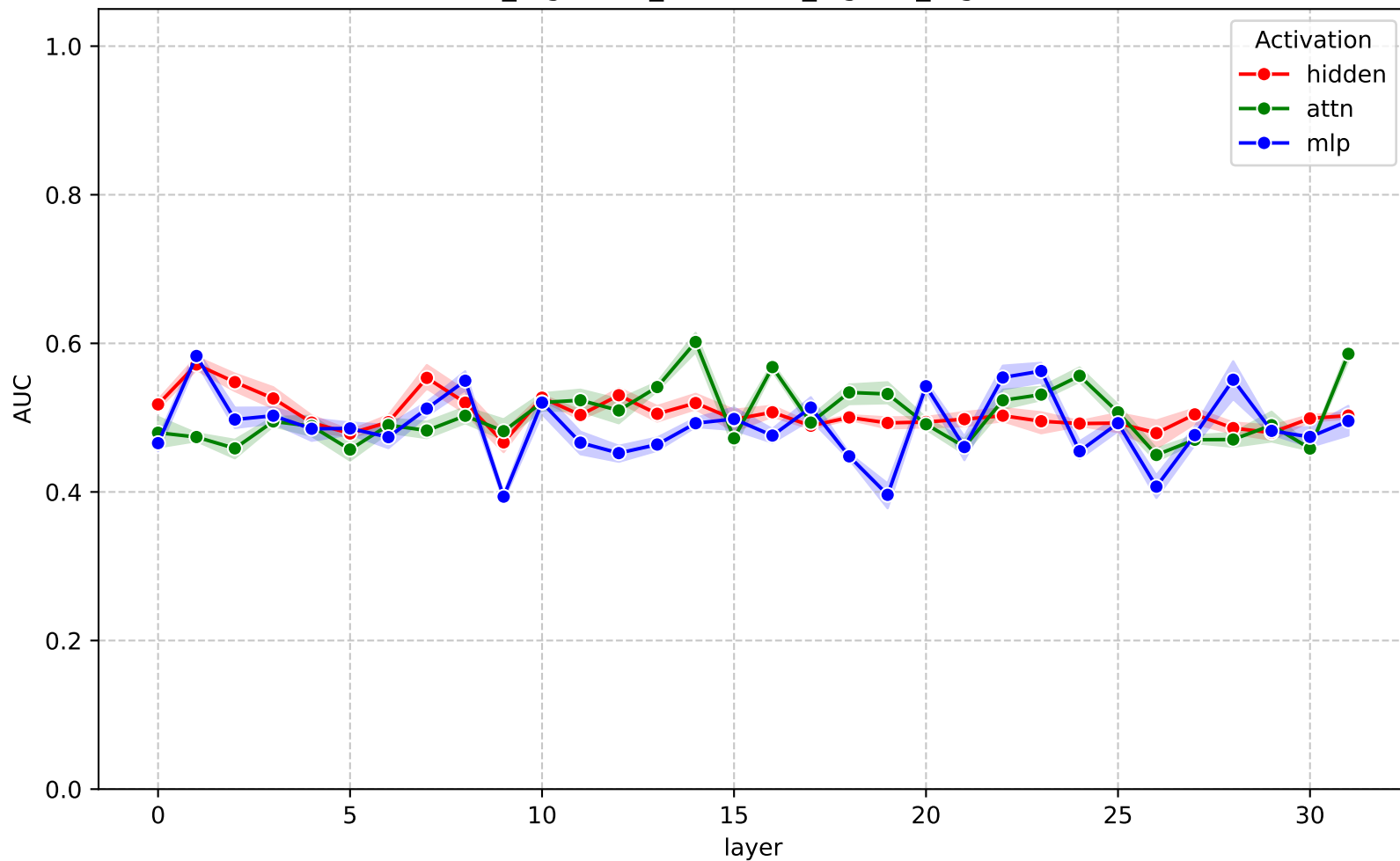
AUC across layers - gemma-3-4b-it (cross_ragbench_combined_logistic_regression)
