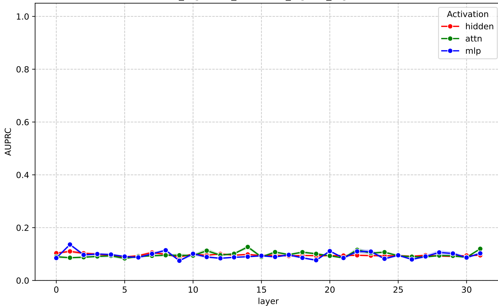
AUPRC across layers - gemma-3-4b-it (cross_ragbench_combined_logistic_regression)
