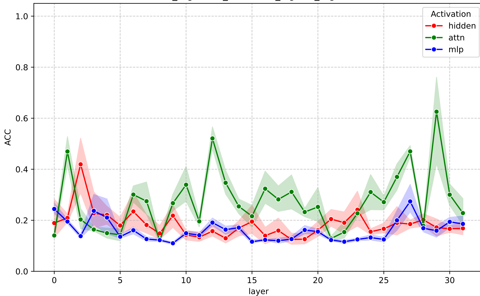
ACC across layers - gemma-3-4b-it (cross_ragbench_combined_logistic_regression)
