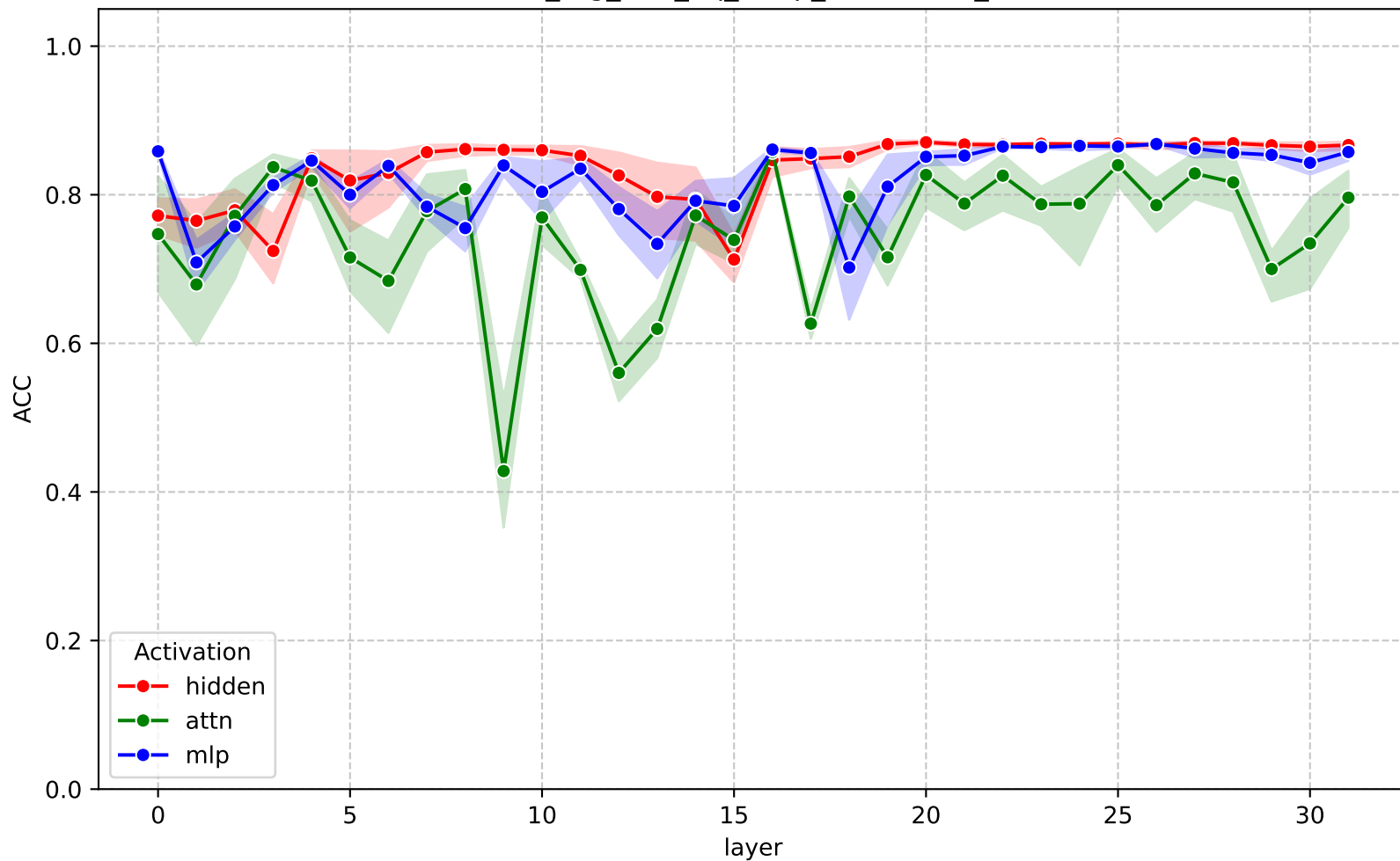
ACC across layers - gemma-3-4b-it (train_rag_test_nq_swap_contextual_ffn)
