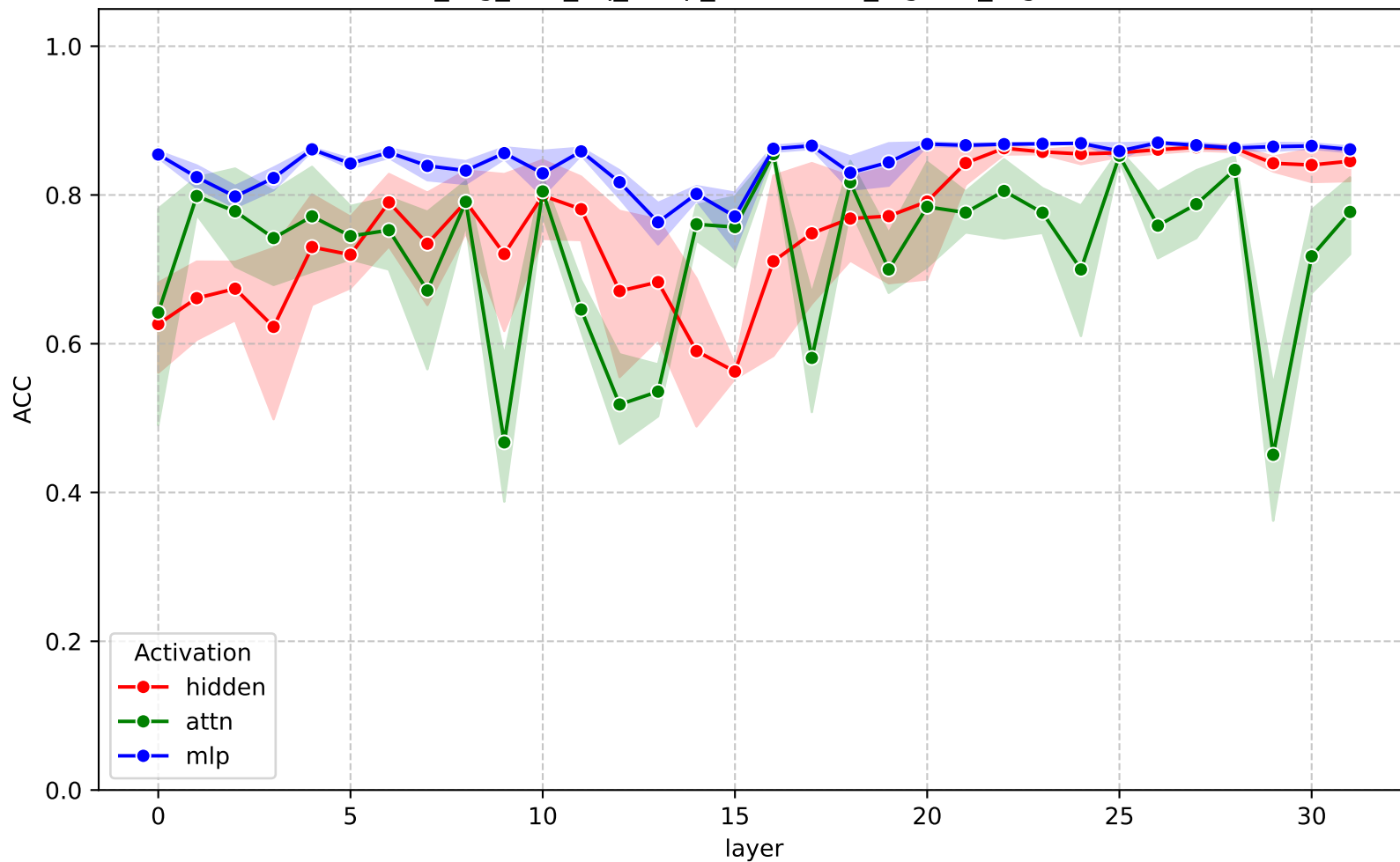
ACC across layers - gemma-3-4b-it (train_rag_test_nq_swap_contextual_logistic_regression)
