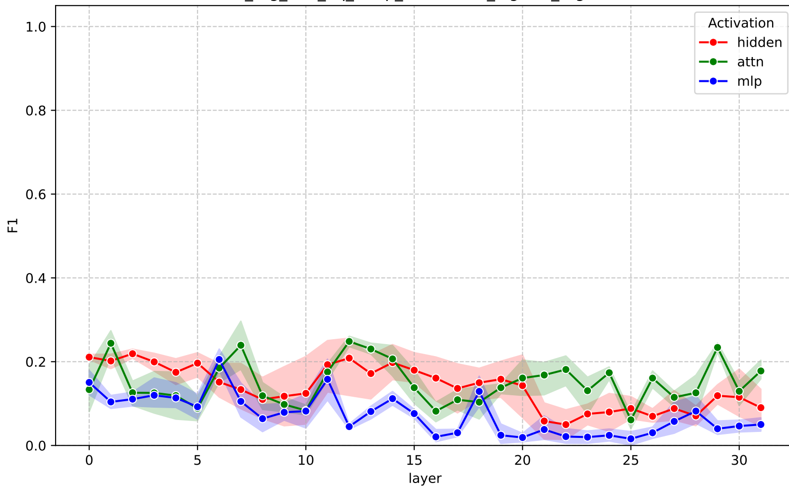
F1 across layers - gemma-3-4b-it (train_rag_test_nq_swap_contextual_logistic_regression)
