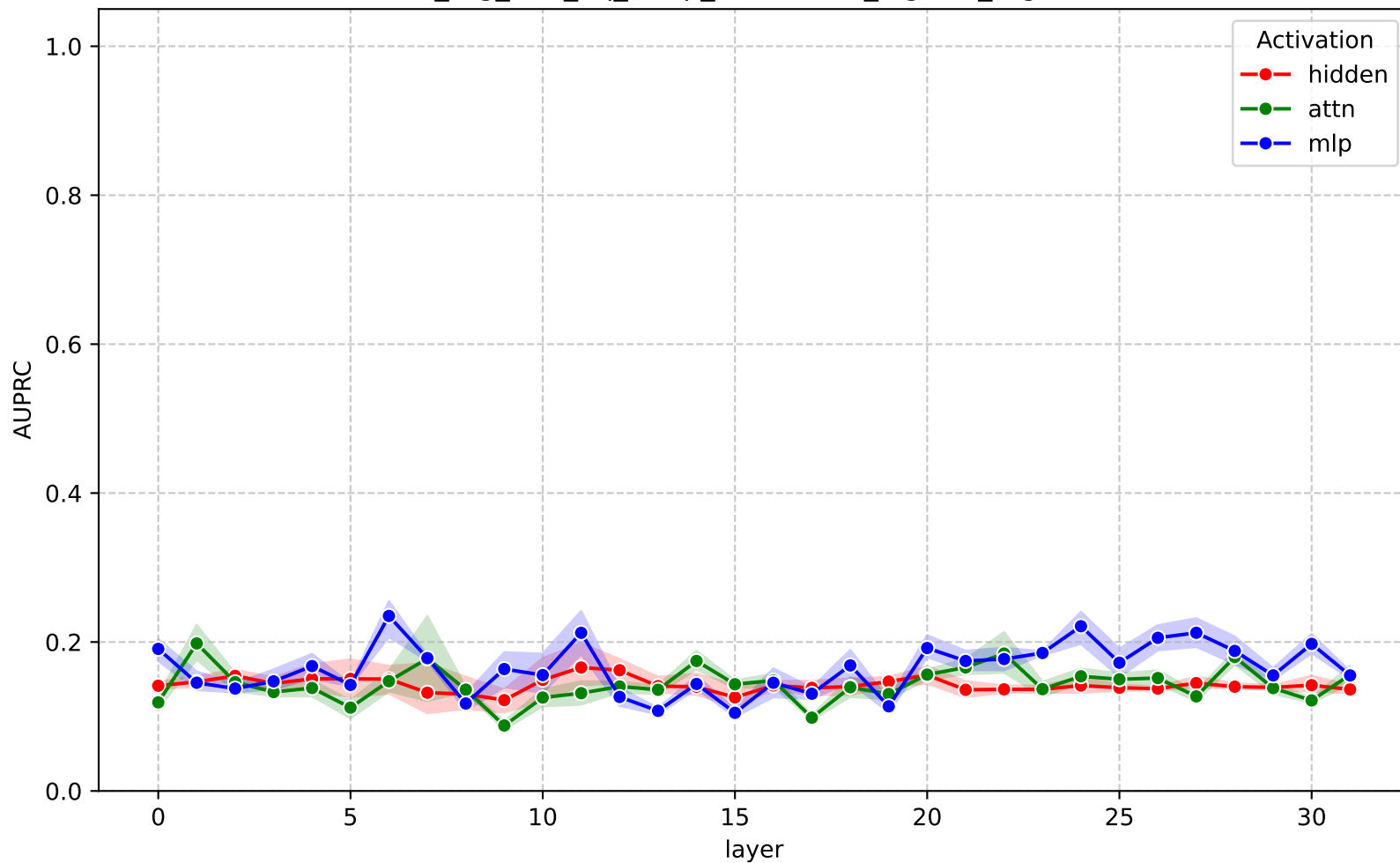
AUPRC across layers - gemma-3-4b-it (train_rag_test_nq_swap_contextual_logistic_regression)
