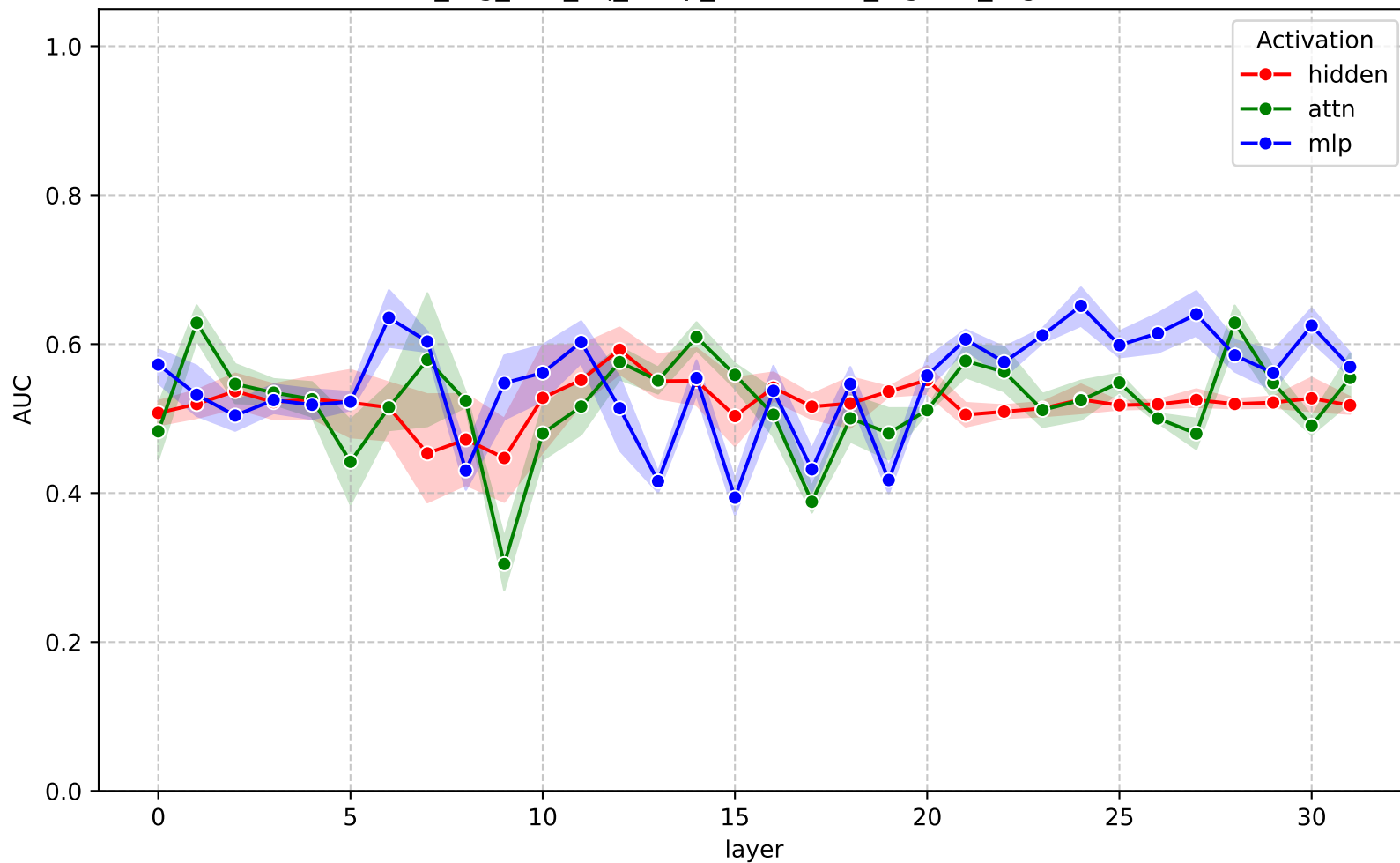
AUC across layers - gemma-3-4b-it (train_rag_test_nq_swap_contextual_logistic_regression)
