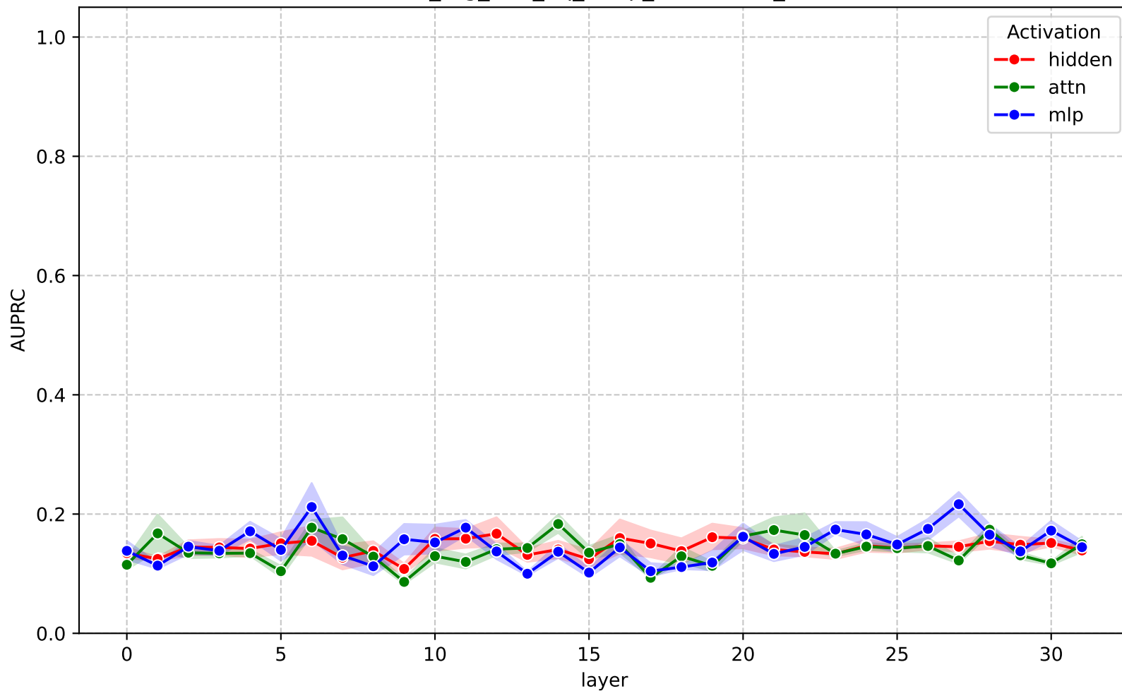
AUPRC across layers - gemma-3-4b-it (train_rag_test_nq_swap_contextual_svm)
