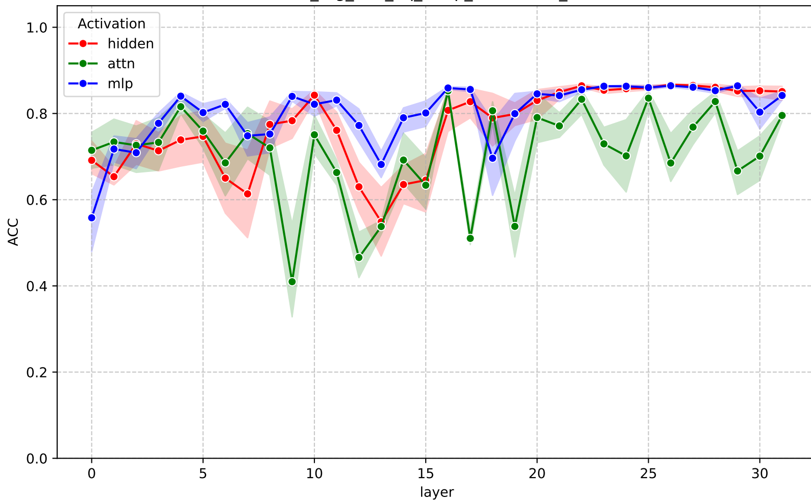
ACC across layers - gemma-3-4b-it (train_rag_test_nq_swap_contextual_svm)
