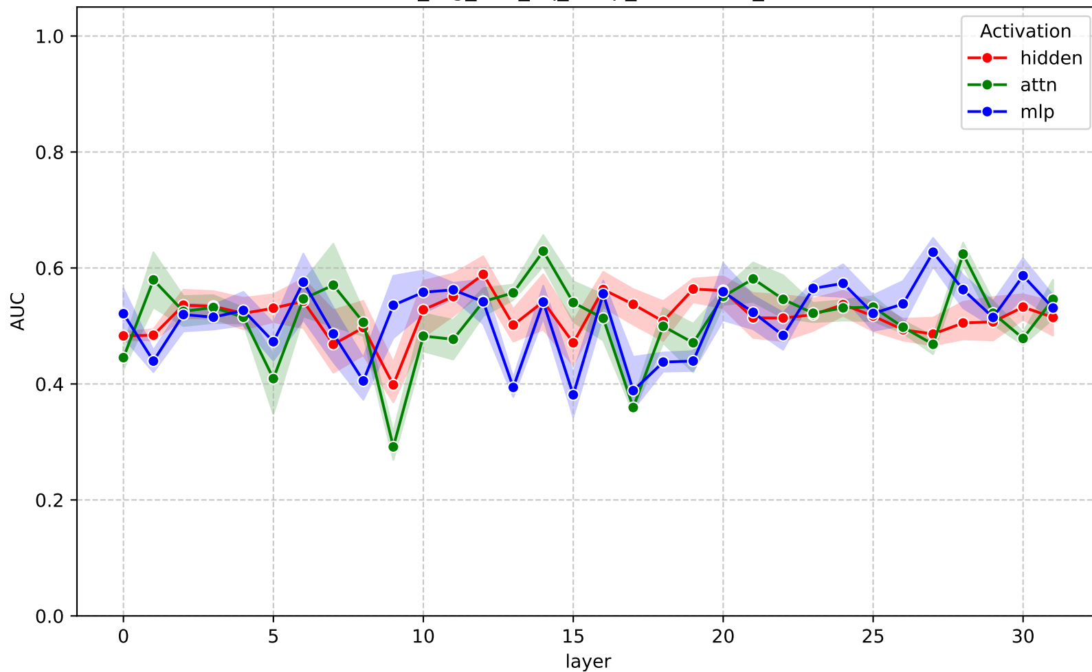
AUC across layers - gemma-3-4b-it (train_rag_test_nq_swap_contextual_svm)
