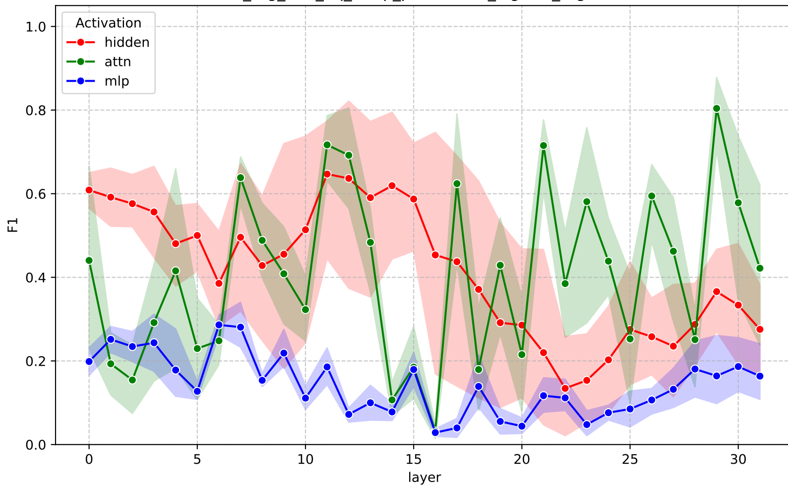
F1 across layers - gemma-3-4b-it (train_rag_test_nq_swap_parametric_logistic_regression)
