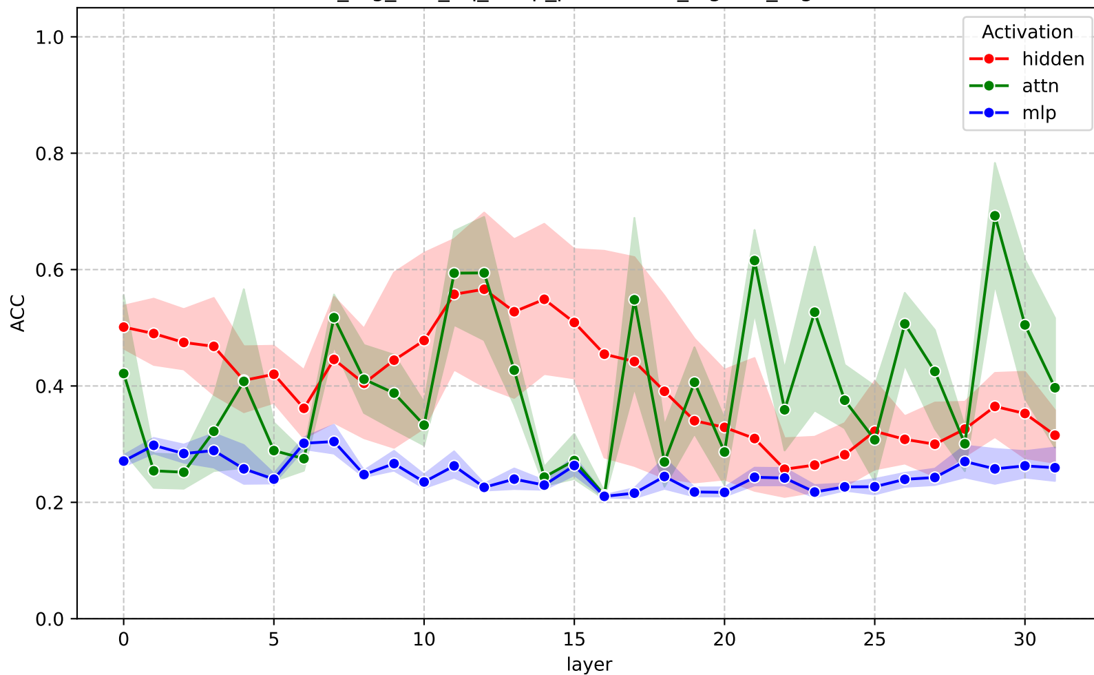
ACC across layers - gemma-3-4b-it (train_rag_test_nq_swap_parametric_logistic_regression)
