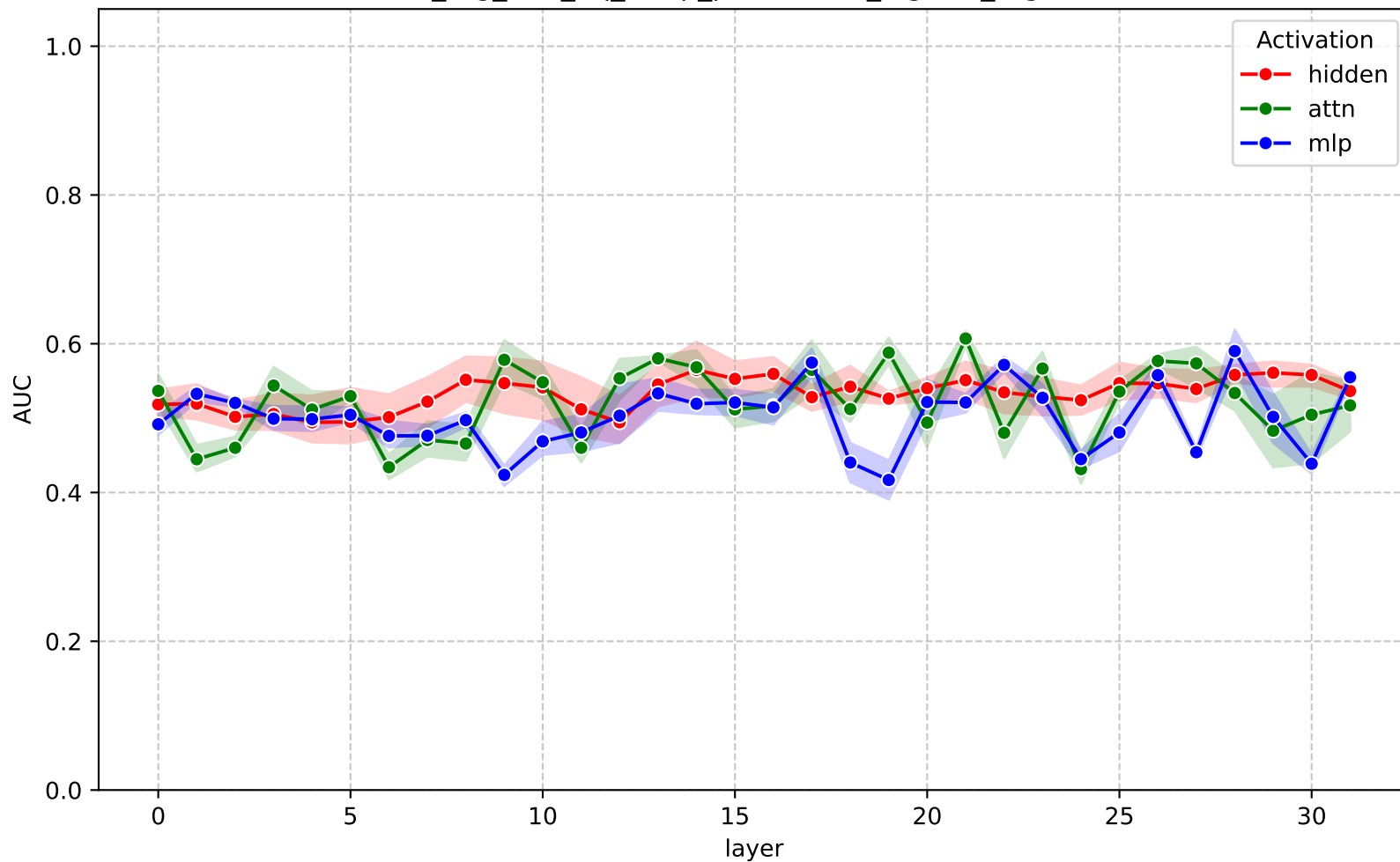
AUC across layers - gemma-3-4b-it (train_rag_test_nq_swap_parametric_logistic_regression)
