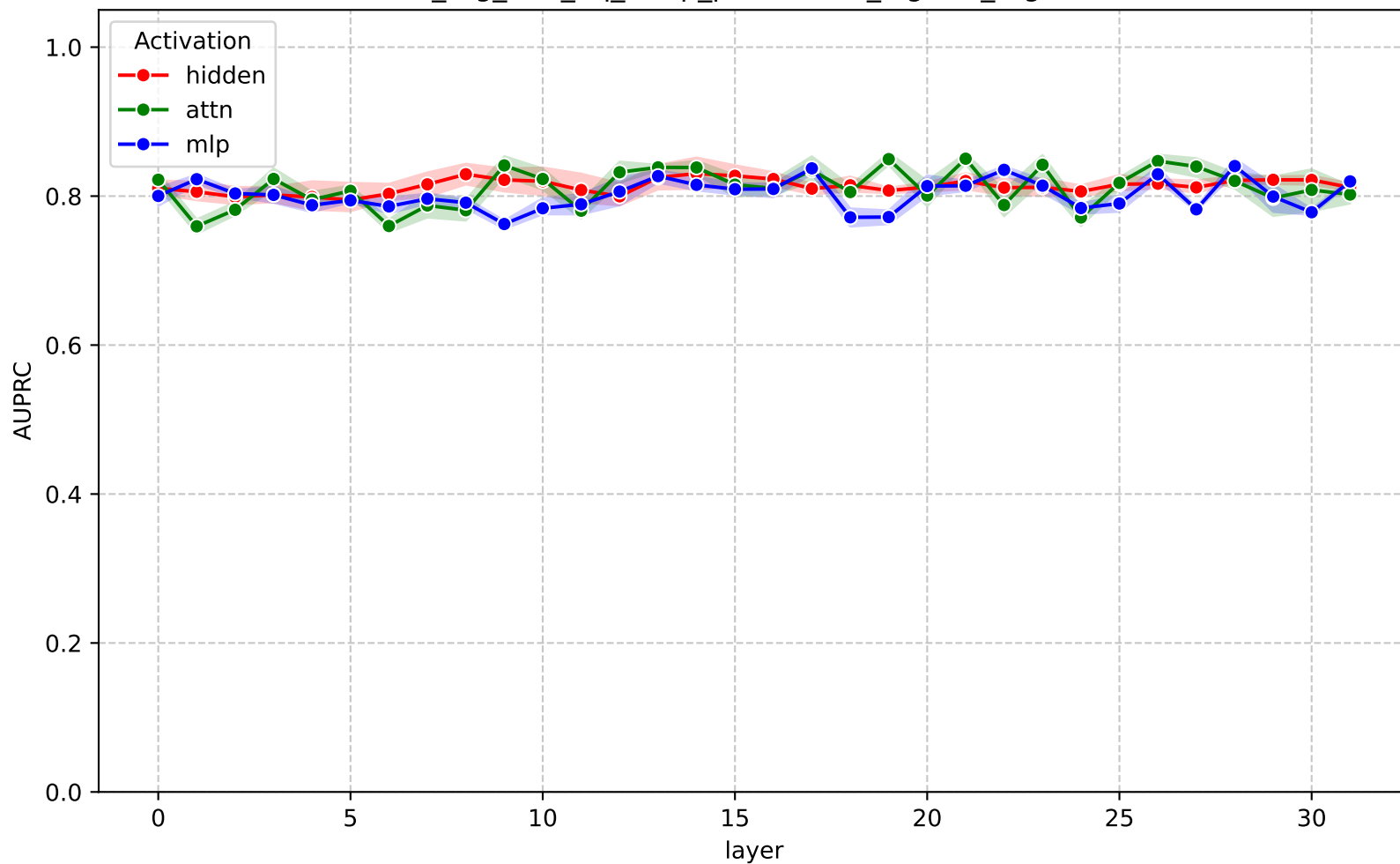
AUPRC across layers - gemma-3-4b-it (train_rag_test_nq_swap_parametric_logistic_regression)
